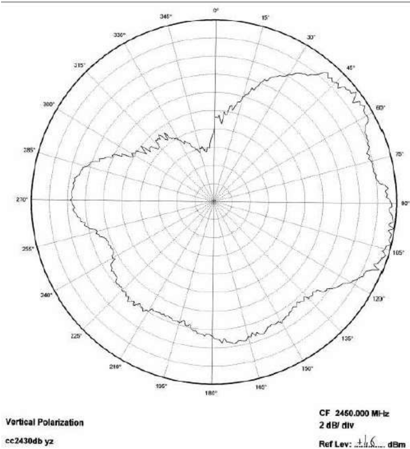
Figure 7. YZ Plane–Vertical Polarization
