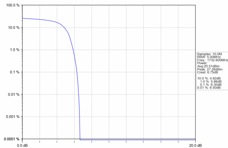
Band4 HSUPA MCH 1732.6MHz Subtest 1 NTNV
