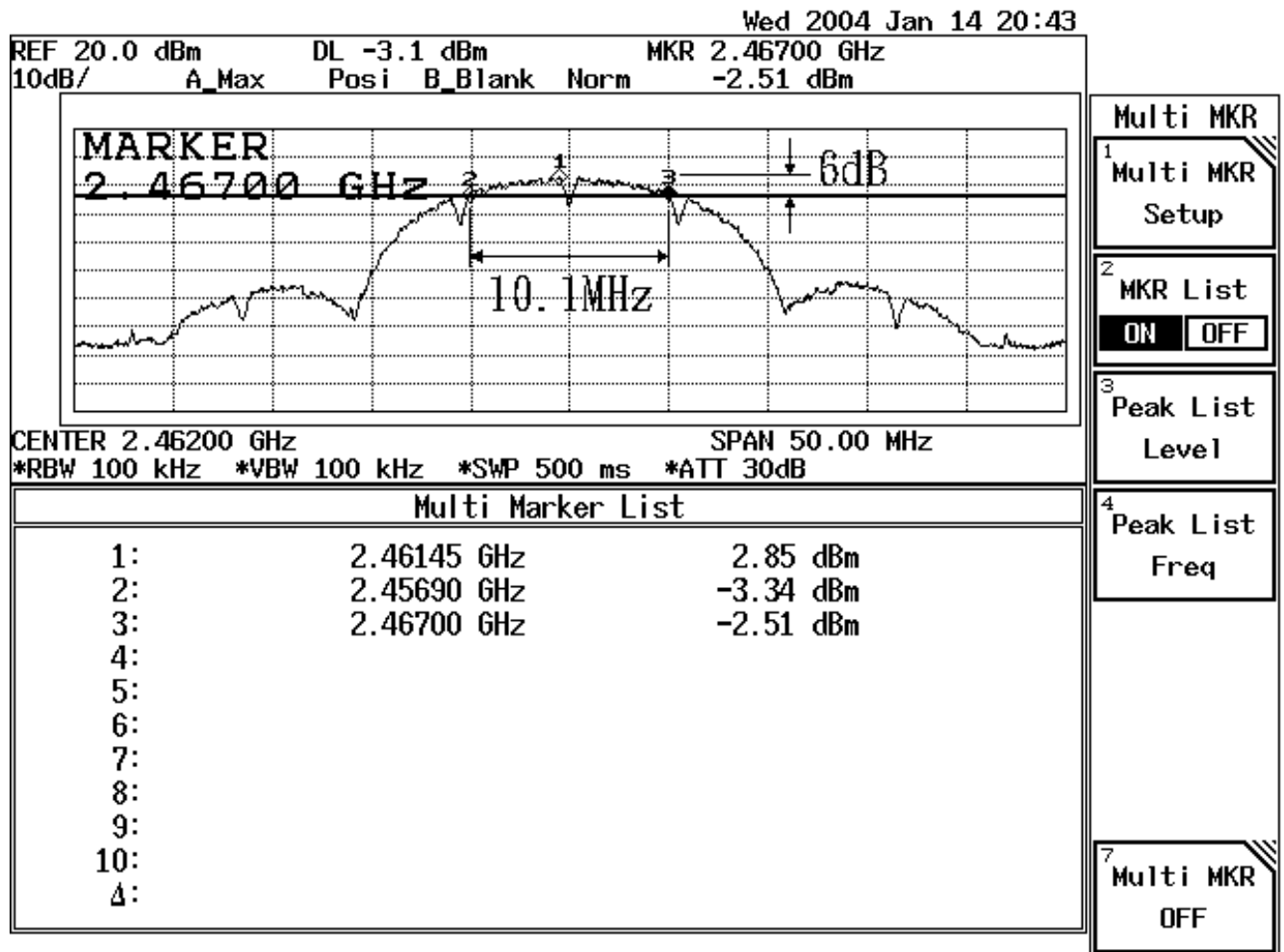
Figure Channel 11: 11Mbps
