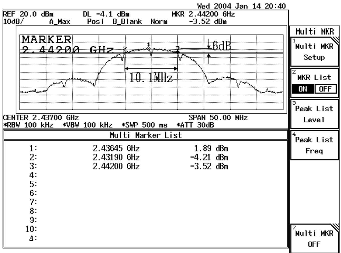
Figure Channel 6: 11Mbps
