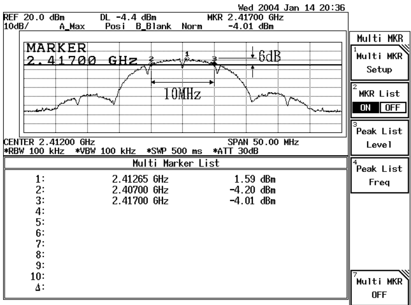
Figure Channel 1: 11Mbps
