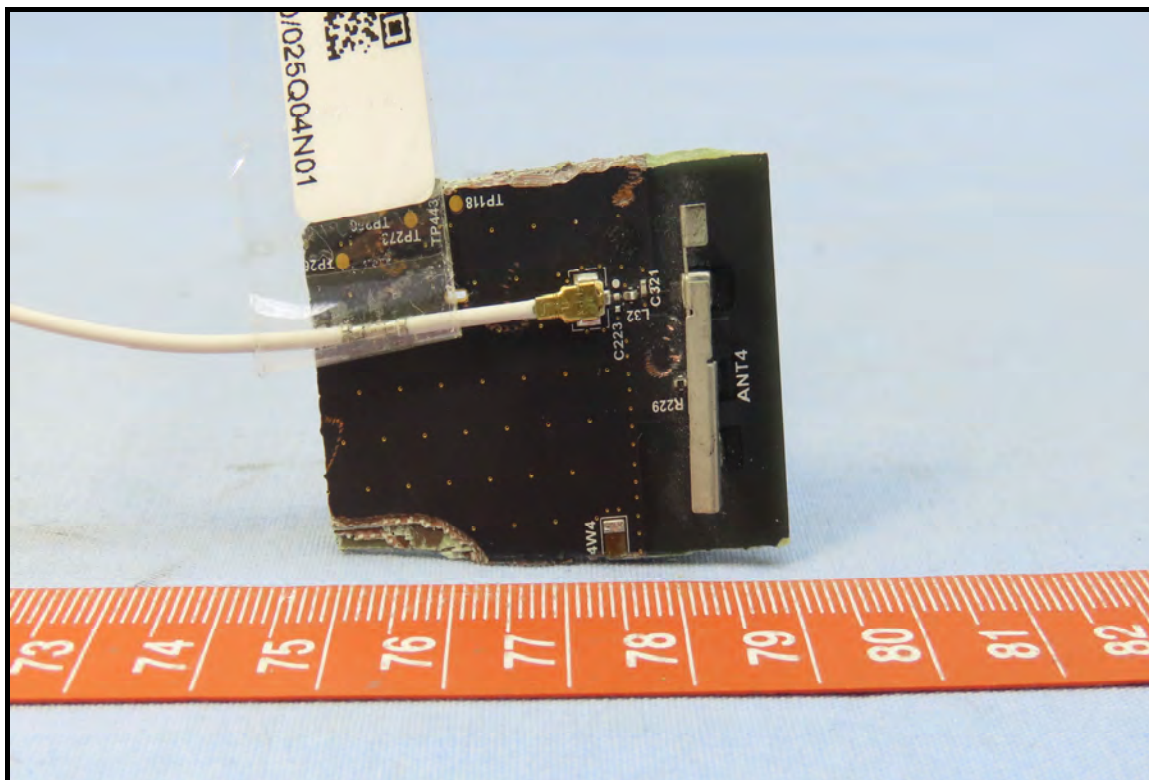
Antenna 2
