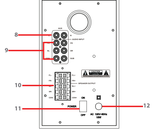
Subwoofer (Back)
