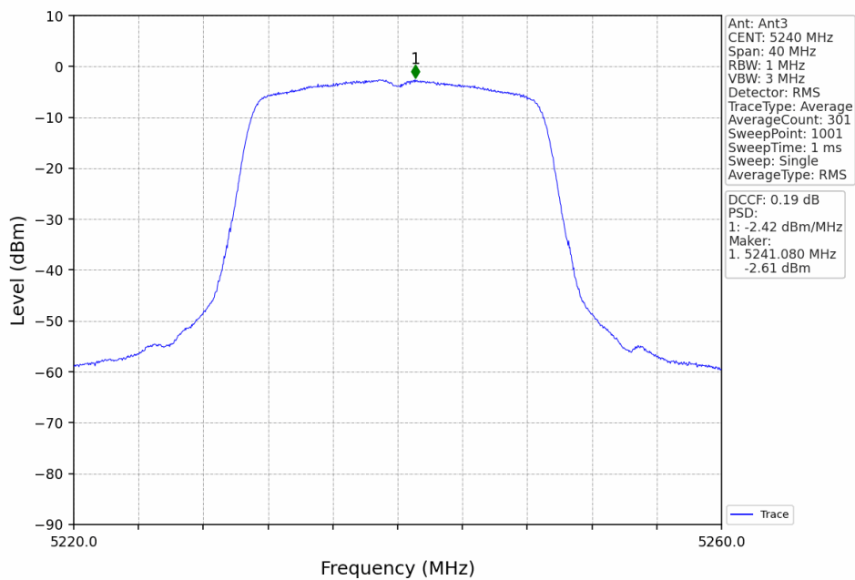
802.11n(HT20)_HCH_5240MHz_Ant3_NTNV
