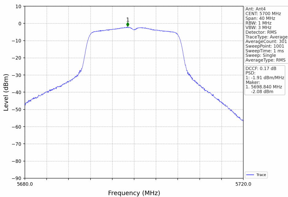
802.11a_HCH_5700MHz_Ant4_NTNV
