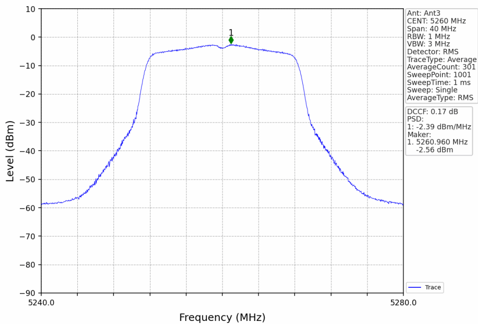
802.11a_LCH_5260MHz_Ant3_NTNV
