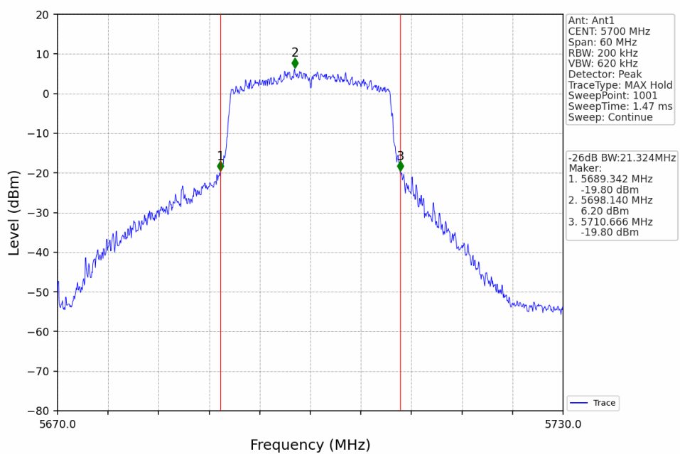
802.11ax(HEW20)_HCH_5700MHz_RU242_Left_Ant1_NTNV
