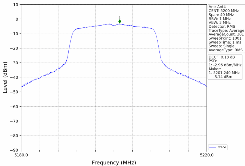
802.11n(HT20)_MCH_5200MHz_Ant4_NTNV
