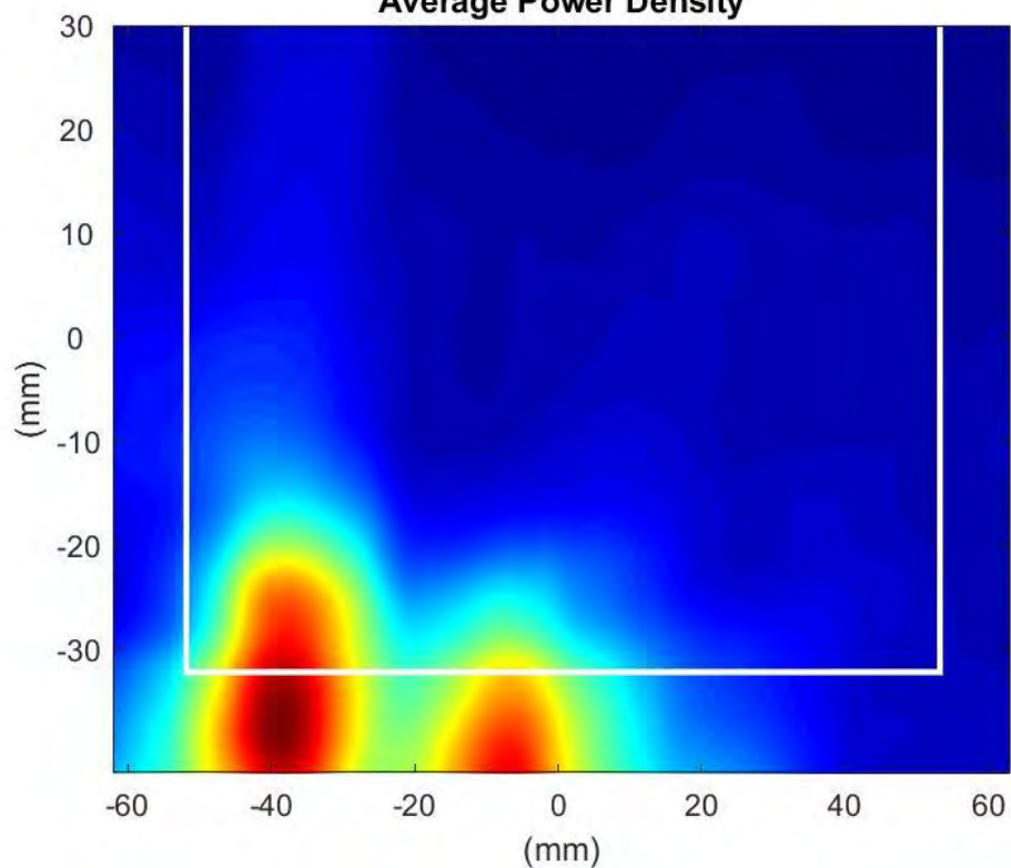
Phaser0 Beam:145 Surface:S1 Average Power Density
