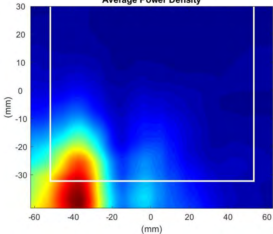
Phaser0 Beam:145 Surface:S2 Average Power Density
