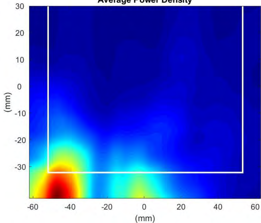
Phaser0 Beam:173 Surface:S1 Average Power Density
