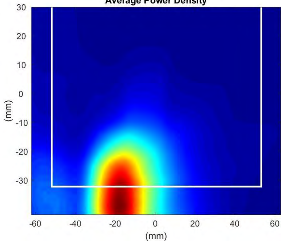
Phaser0 Beam:143 Surface:S2 Average Power Density
