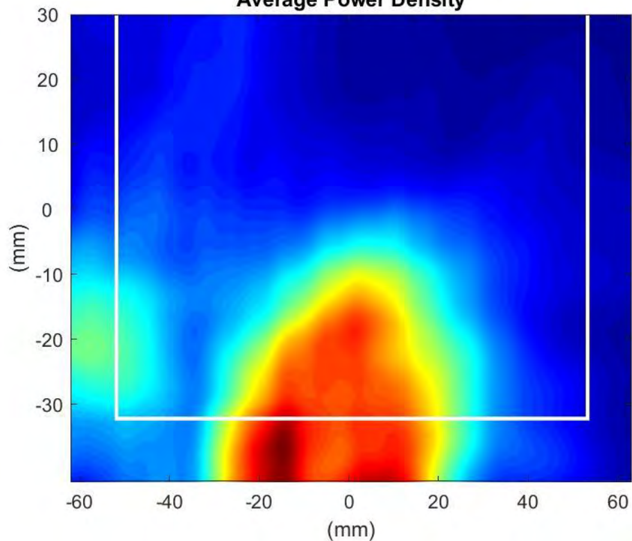
Phaser0 Beam:157 Surface:S2 Average Power Density
