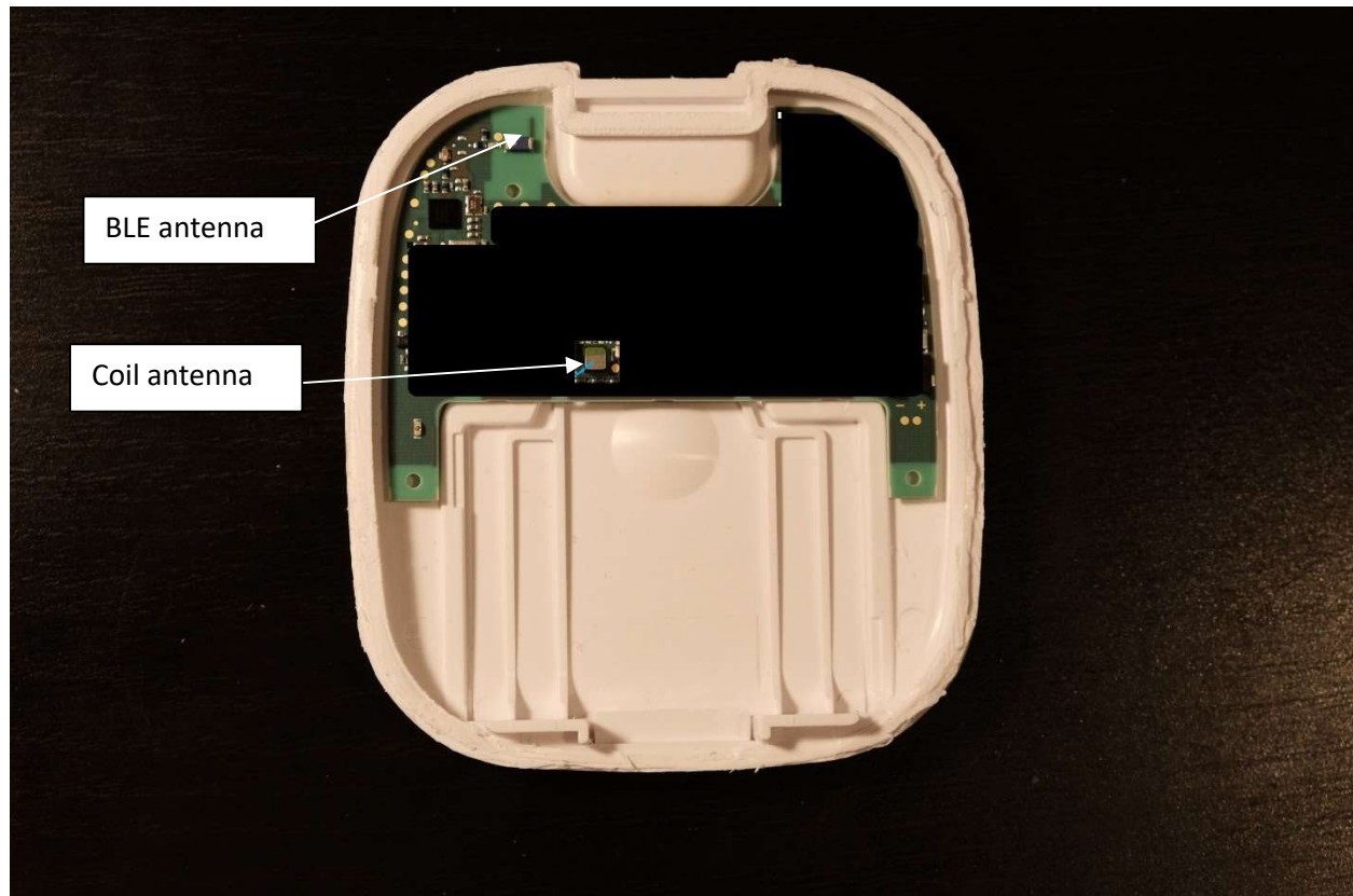
Figure 1 Antenna on PCB
