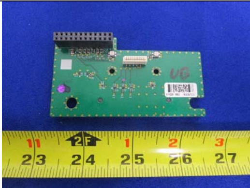
PCB 1- Front View
