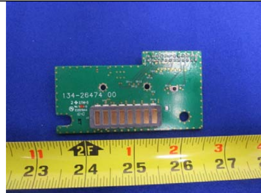
PCB 1 - Rear View
