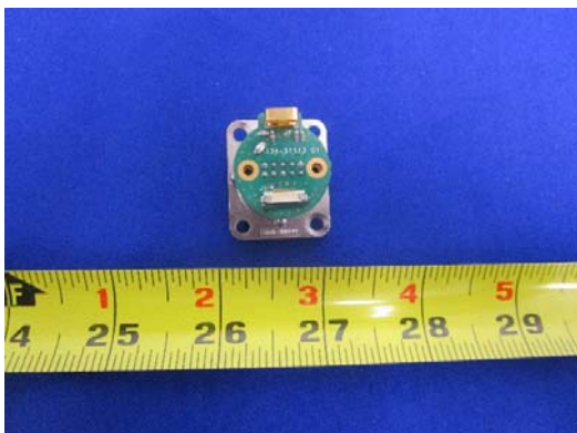
PCB 5 - Front View
