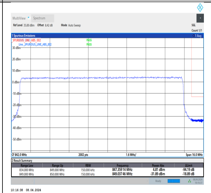
Band26_15MHz_QPSK_26965_75RB#0
