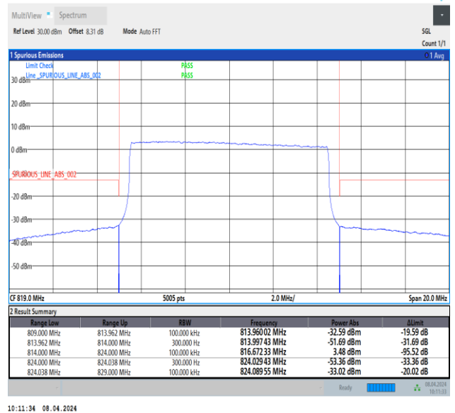
Band26_10MHz_64QAM_26740_50RB#0
