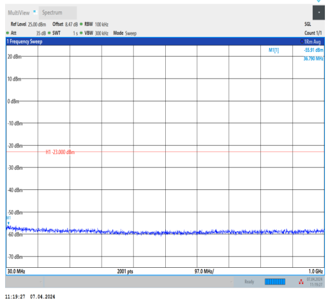
Band2_3MHz_QPSK_18615_1RB#0_30~1000_30~1000
