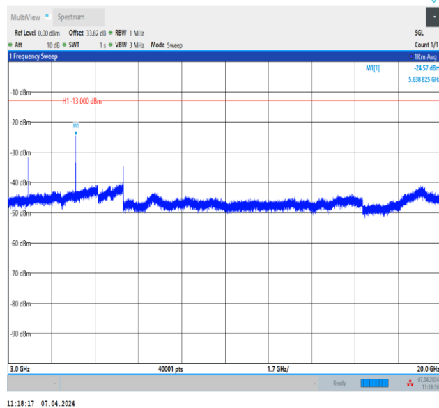
Band2_1.4MHz_QPSK_18900_1RB#0_3000~20000_3000~20000
