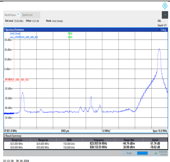
Band26_15MHz_64QAM_26865_1RB#74
