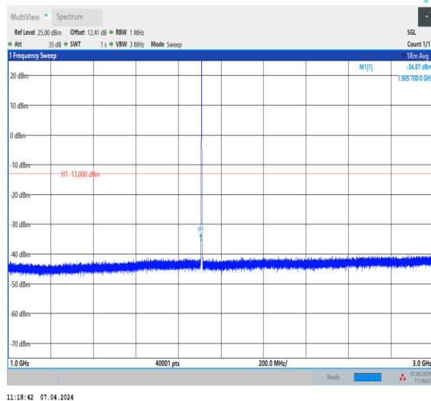
Band2_1.4MHz_QPSK_19193_1RB#0_1000~3000_1000~3000
