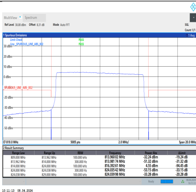
Band26_10MHz_16QAM_26740_50RB#0
