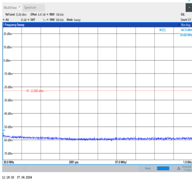
Band2_1.4MHz_QPSK_19193_1RB#0_30~1000_30~1000
