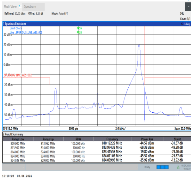
Band26_10MHz_64QAM_26740_1RB#49
