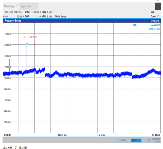
Band2_3MHz_QPSK_18615_1RB#0_3000~20000_3000~20000
