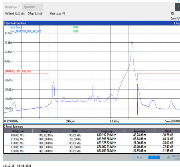
Band26_10MHz_16QAM_26740_1RB#49
