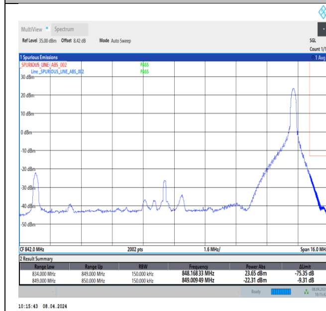
Band26_15MHz_QPSK_26965_1RB#74
