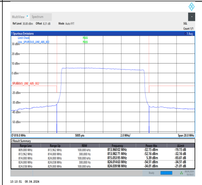
Band26_10MHz_QPSK_26740_50RB#0
