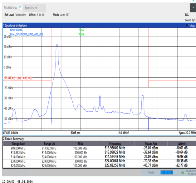
Band26_10MHz_16QAM_26740_1RB#0
