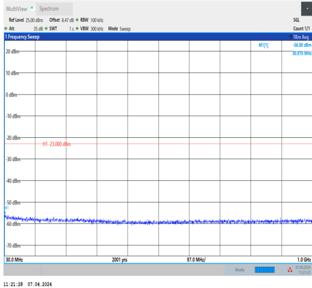
Band2_5MHz_QPSK_18625_1RB#0_30~1000_30~1000
