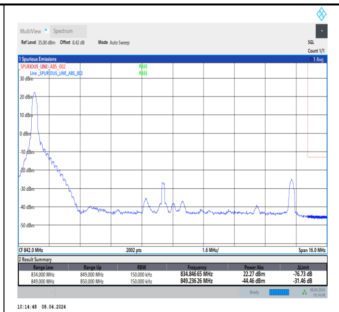
Band26_15MHz_QPSK_26965_1RB#0
