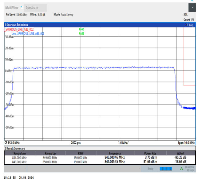
Band26_15MHz_16QAM_26965_75RB#0
