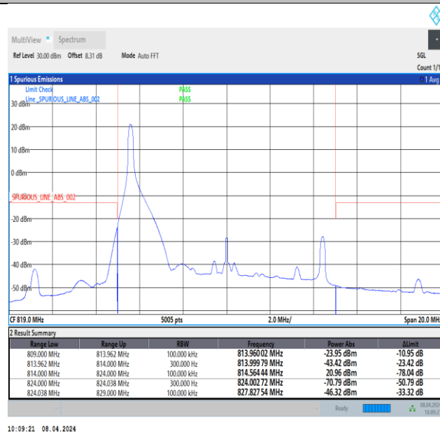
Band26_10MHz_64QAM_26740_1RB#0
