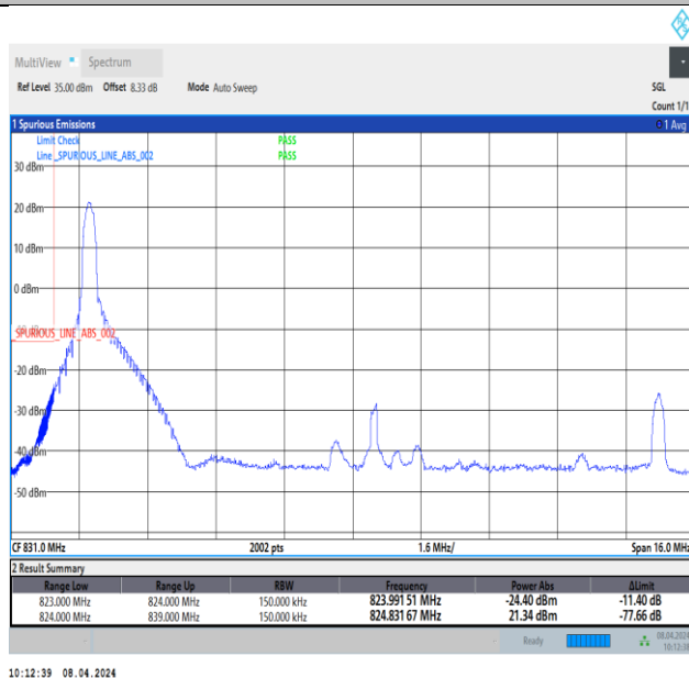
Band26_15MHz_64QAM_26865_1RB#0
