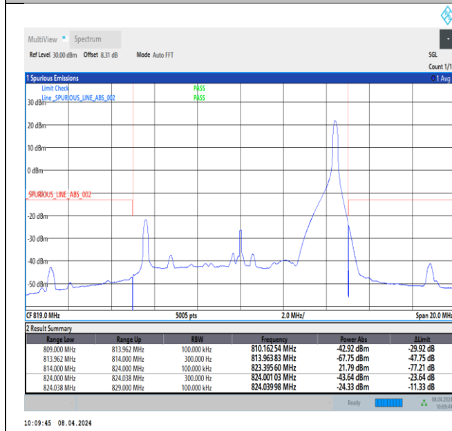
Band26_10MHz_QPSK_26740_1RB#49
