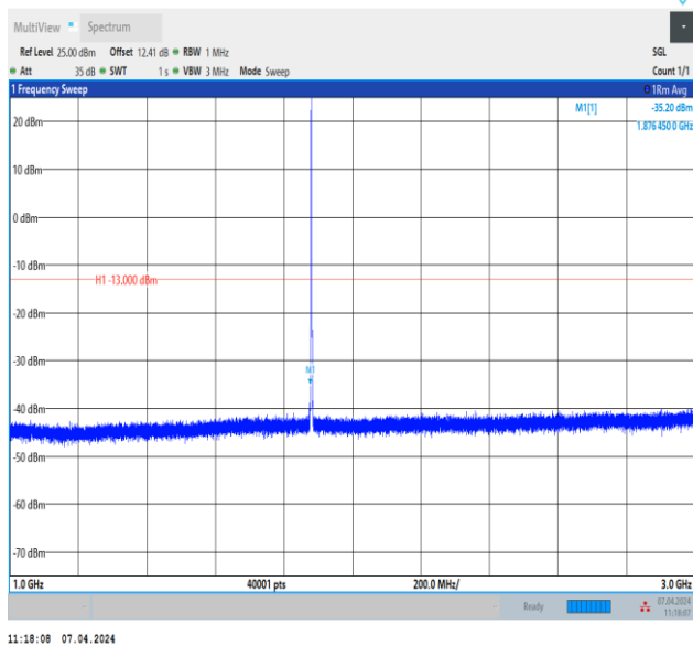
Band2_1.4MHz_QPSK_18900_1RB#0_1000~3000_1000~3000
