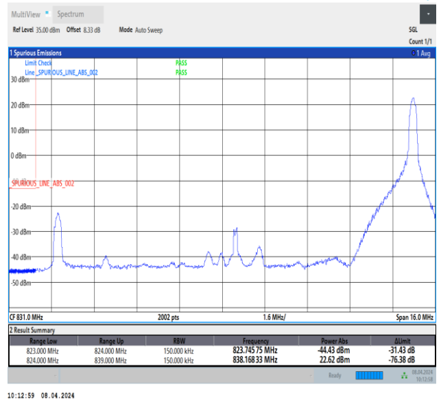
Band26_15MHz_QPSK_26865_1RB#74
