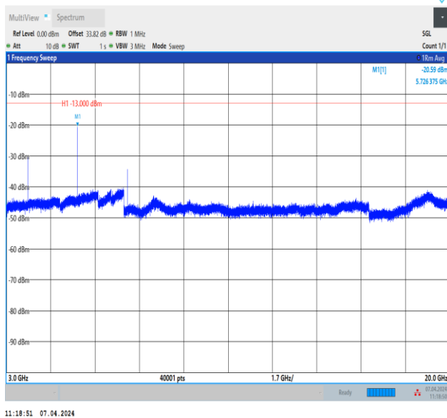
Band2_1.4MHz_QPSK_19193_1RB#0_3000~20000_3000~20000
