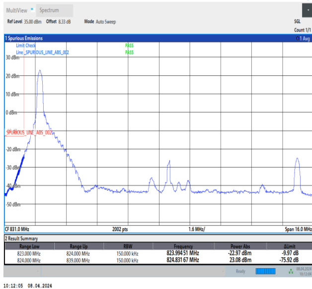
Band26_15MHz_QPSK_26865_1RB#0
