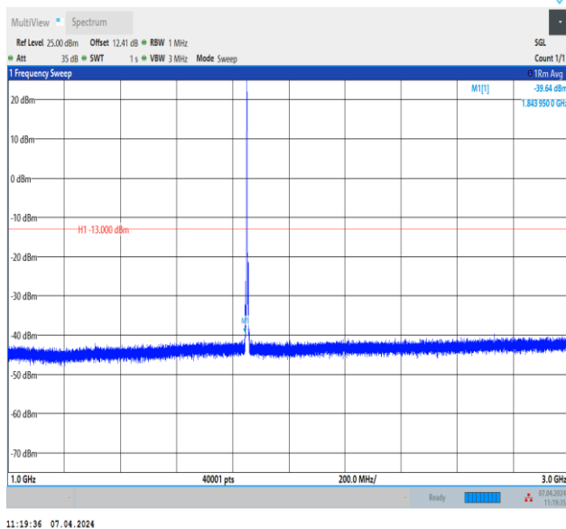
Band2_3MHz_QPSK_18615_1RB#0_1000~3000_1000~3000
