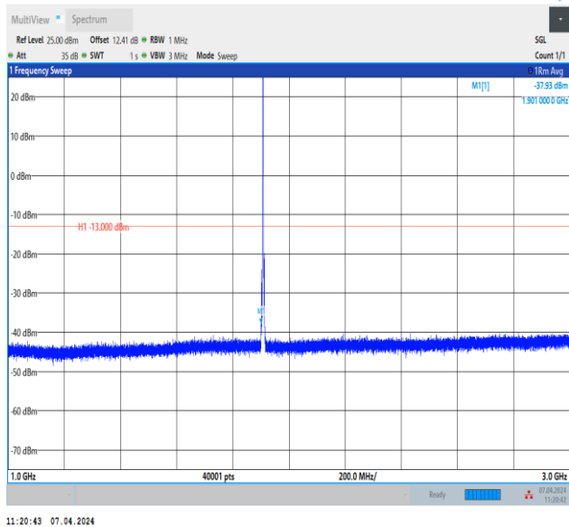
Band2_3MHz_QPSK_19185_1RB#0_1000~3000_1000~300 0
