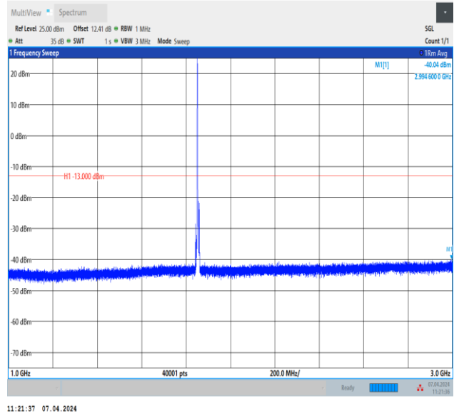
Band2_5MHz_QPSK_18625_1RB#0_1000~3000_1000~300 0
