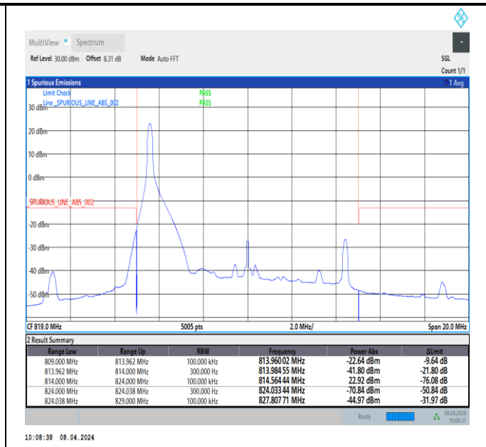
Band26_10MHz_QPSK_26740_1RB#0
