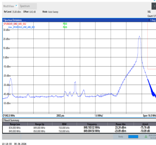
Band26_15MHz_16QAM_26965_1RB#74
