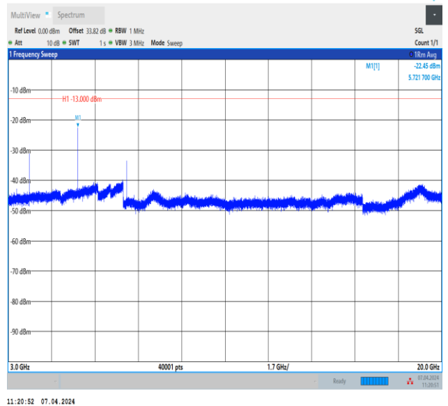
Band2_3MHz_QPSK_19185_1RB#0_3000~20000_3000~20 000
