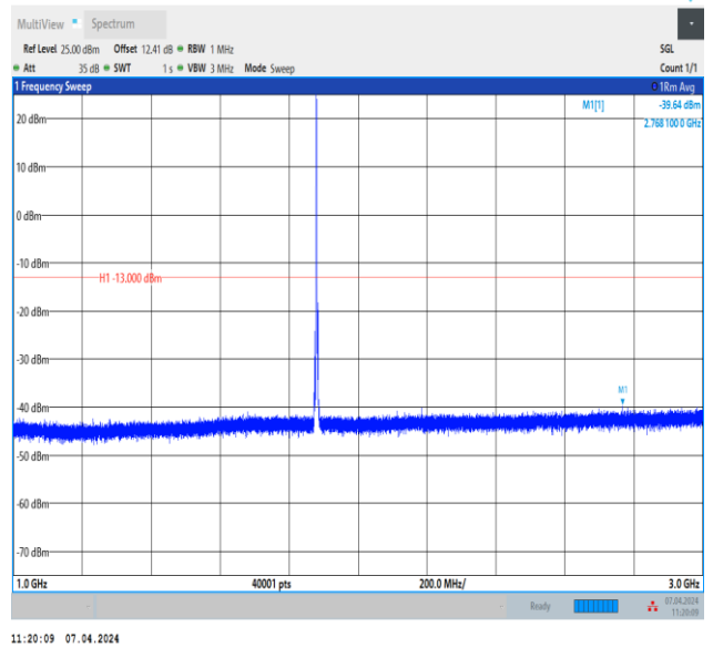
Band2_3MHz_QPSK_18900_1RB#0_1000~3000_1000~300 0
