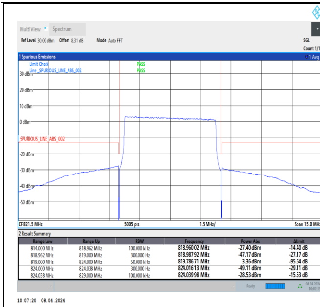
Band26_5MHz_64QAM_26765_25RB#0
