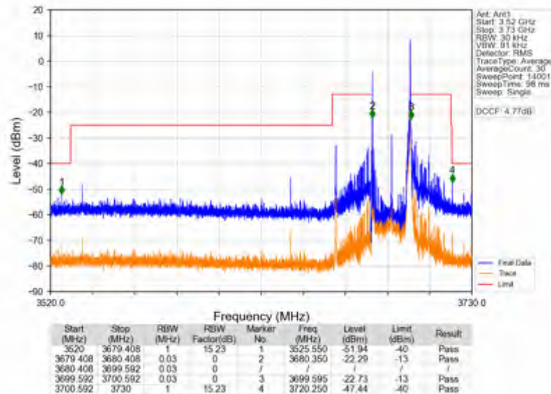
n78d_15kHz_SISO_NTNV_20MHz_CP-OFDM_QPSK_3690MHz_Inner_1RB_Right
