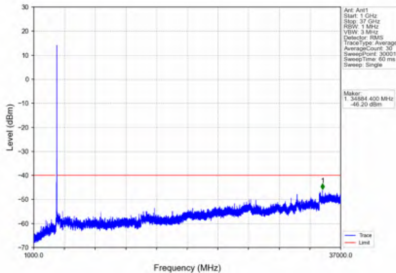
n78d_15kHz_SISO_NTNV_20MHz_DFT-s-OFDM QPSK_3690MHz_Edge_1RB_Right
