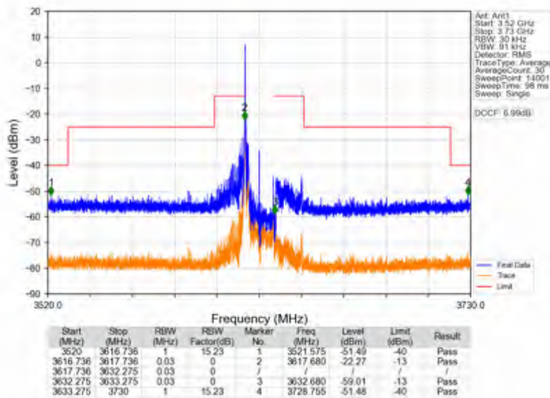
n78d_15kHz_SISO_NTNV_15MHz_CP-OFDM QPSK_3625.005MHz_Edge_1RB_Left
