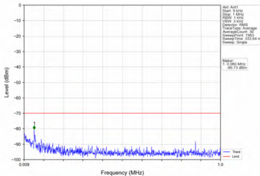
n78d_15kHz_SISO_NTNV_15MHz_CP-OFDM QPSK_3692.49MHz_Edge_1RB_Right
