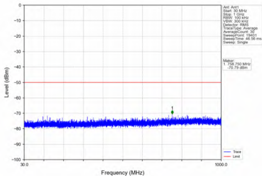
n78d 15kHz SISO NTN 10MHz CP-OFDM QPSK 3555MHz Outer Full
