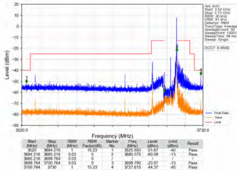
n78d_15kHz_SISO_NTNV_15MHz_CP-OFDM QPSK_3692.49MHz_Edge_1RB_Right
