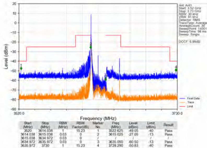
n78d_15kHz_SISO_NTNV_20MHz_DFT-s-OFDM QPSK_3625.005MHz_Edge_1RB_Left
