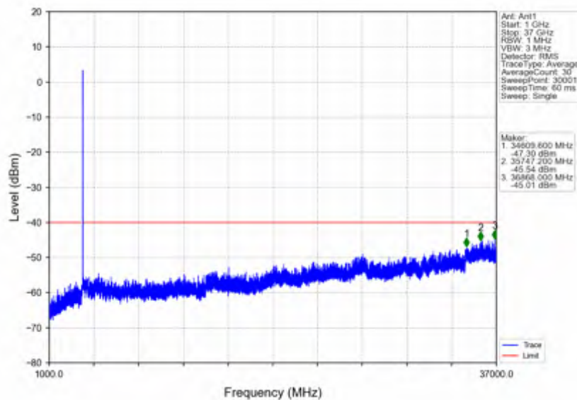
n78d_15kHz_SISO_NTNV_15MHz_DFT-s-OFDM_QPSK_3692.49MHz_Inner_1RB_Right
