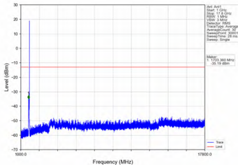
n66_30kHz_SISO_NTNV_40MHz_CP-OFDM QPSK_1760MHz_Outer_Full
