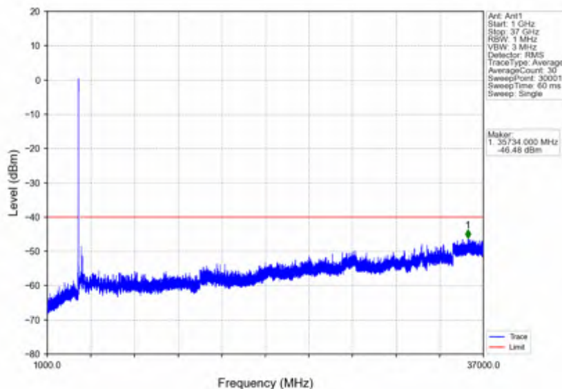
n78d_15kHz_SISO_NTNV_20MHz_DFT-s-OFDM_QPSK_3560.01MHz_Inner_1RB_Left
