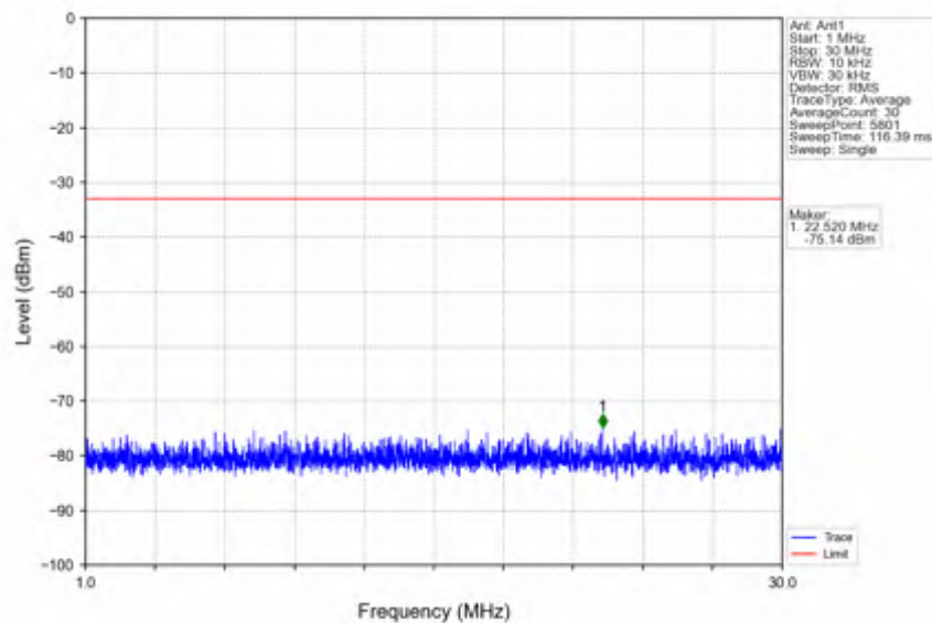
n66_30kHz_SISO_NTNV_40MHz_CP-OFDM QPSK_1760MHz_Outer_Full
