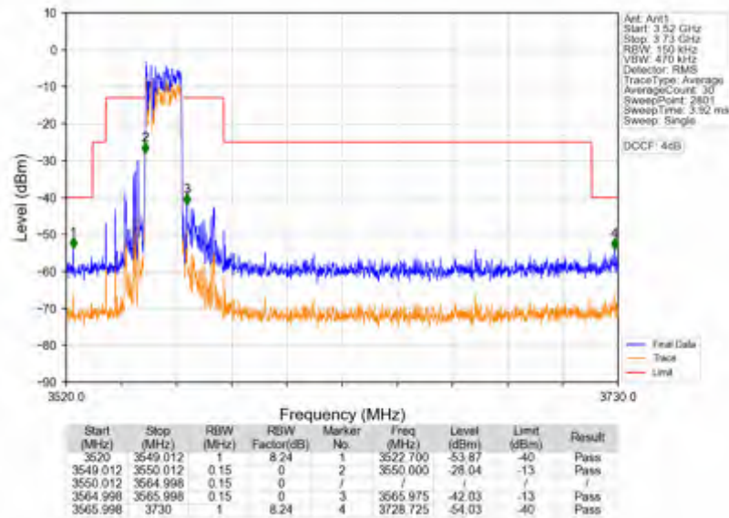
n78d_15kHz_SISO_NTNV_15MHz_DFT-s-OFDM QPSK_3557.505MHz_Outer_Full
