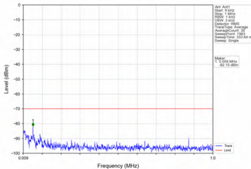
n78d_15kHz_SISO_NTNV_10MHz_CP-OFDM_QPSK_3555MHz_Edge_1RB_Left
