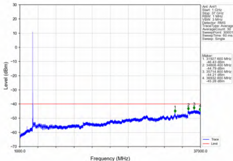
n78d_15kHz_SISO_NTNV_25MHz_DFT-s-OFDM_PI/2_BPSK_3562.5MHz_Outer_Full
