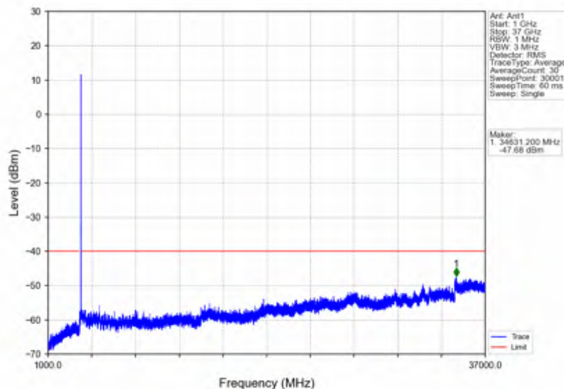
n78d_15kHz_SISO_NTNV_10MHz_CP-OFDM QPSK_3694.995MHz_Outer_Full
