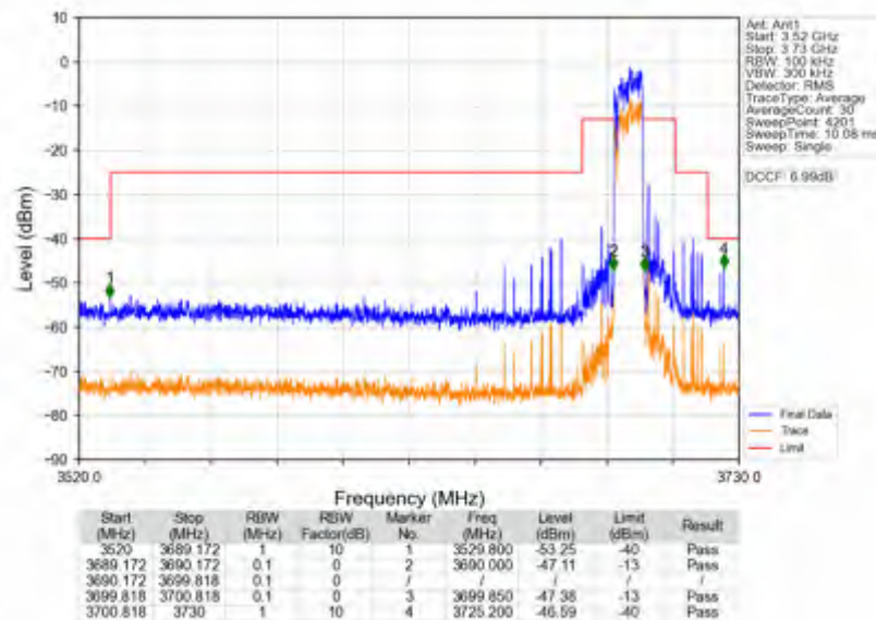
n78d_15kHz_SISO_NTNV_10MHz_DFT-s-OFDM QPSK_3694.995MHz_Outer_Full
