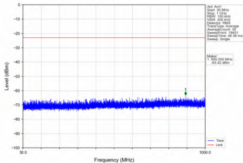
n66_30kHz_SISO_NTNV_40MHz_CP-OFDM_QPSK_1745MHz_Edge_1RB_Left
