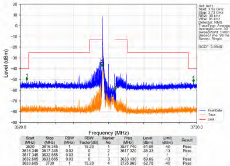
n78d_15kHz_SISO_NTNV_15MHz_DFT-s-OFDM QPSK_3625.005MHz_Edge_1RB_Left
