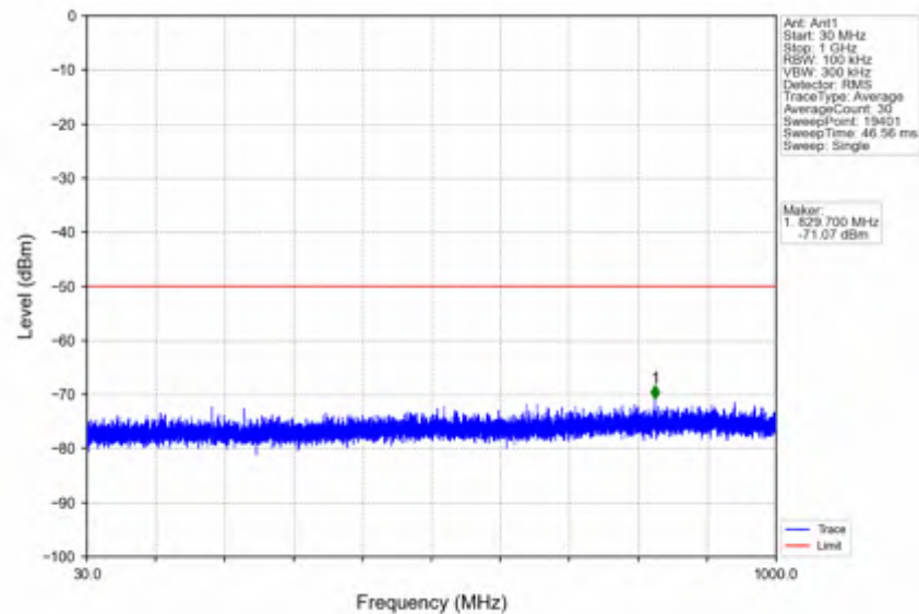
n78d_15kHz_SISO_NTNV_10MHz_CP-OFDM QPSK_3625.005MHz_Edge_1RB_Left
