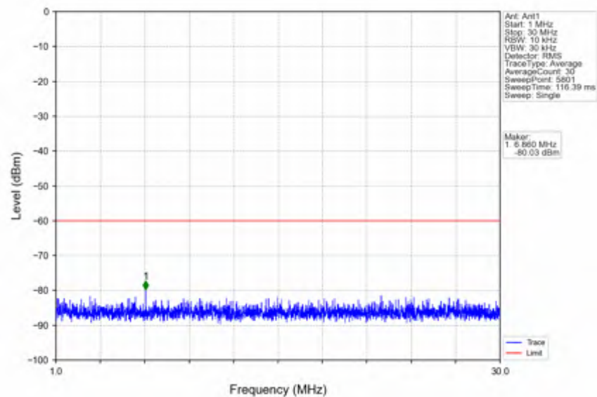
n78d_15kHz_SISO_NTNV_15MHz_CP-OFDM QPSK_3692.49MHz_Outer_Full
