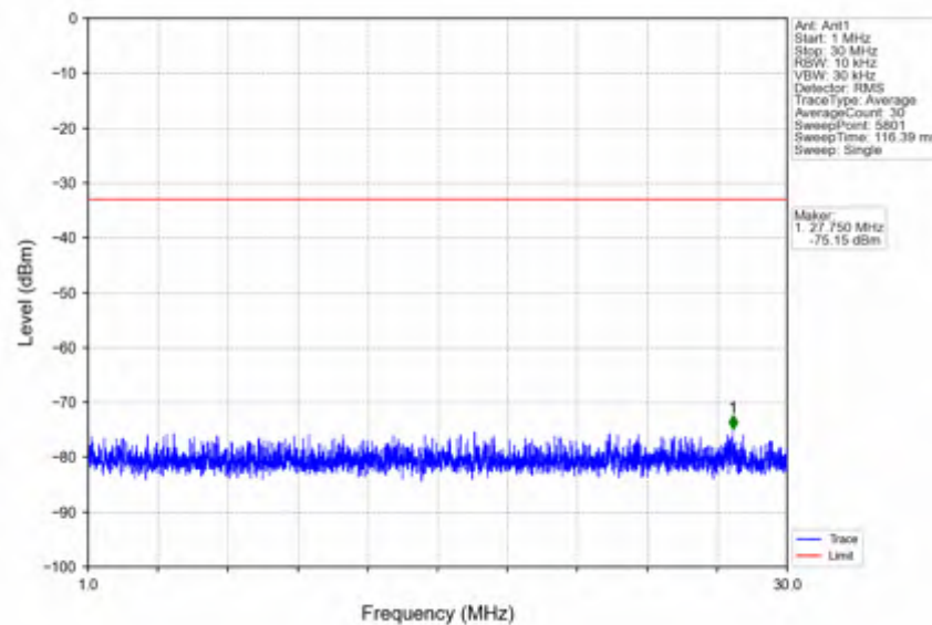
n66_30kHz_SISO_NTNV_40MHz_CP-OFDM QPSK_1760MHz_Edge_1RB_Right
