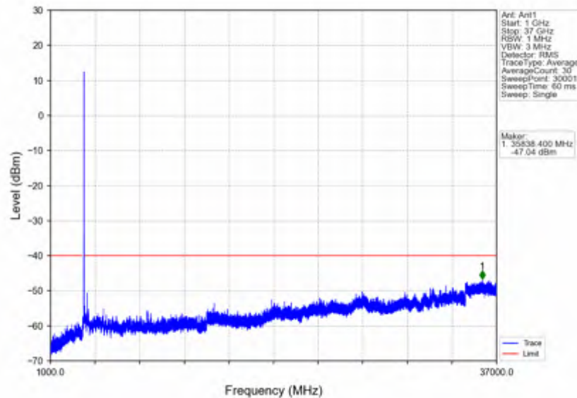
n78d_15kHz_SISO_NTNV_15MHz_DFT-s-OFDM QPSK_3692.49MHz_Edge_1RB_Right
