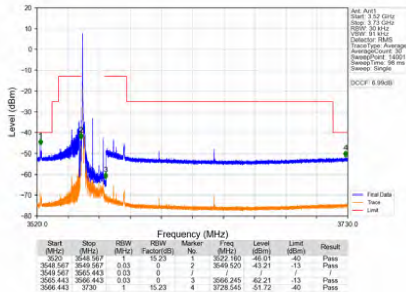
n78d_15kHz_SISO_NTNV_15MHz_DFT-s-OFDM_PI/2_BPSK_3557.505MHz_Edge_1RB_Left
