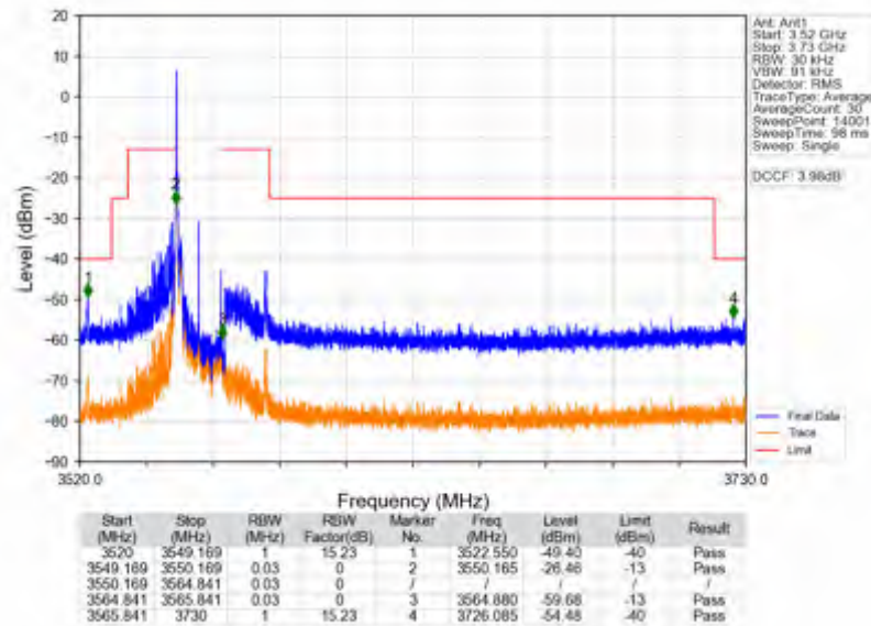
n78d_15kHz_SISO_NTNV_15MHz_CP-OFDM_QPSK_3557.505MHz_Edge_1RB_Left
