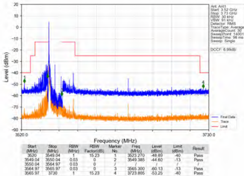
n78d_15kHz_SISO_NTNV_15MHz_DFT-s-OFDM QPSK_3557.505MHz_Inner_1RB_Left
