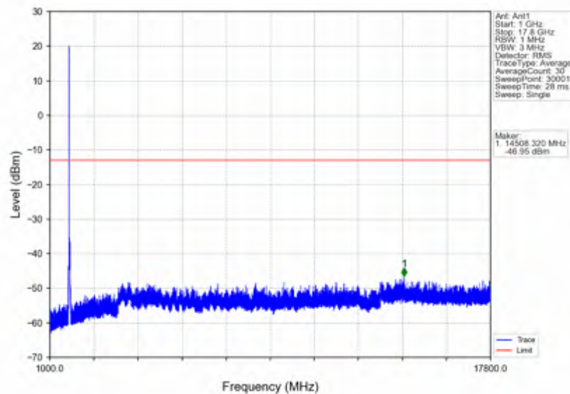
n66_30kHz_SISO_NTNV_40MHz_CP-OFDM_QPSK_1745MHz_Edge_1RB_Left
