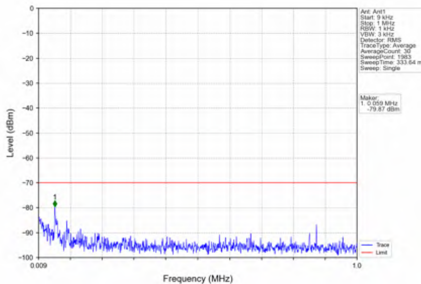
n78d_15kHz_SISO_NTNV_15MHz_DFT-s-OFDM QPSK_3625.005MHz_Edge_1RB_Left
