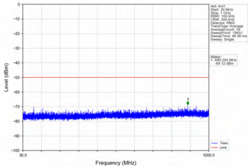
n78d_15kHz_SISO_NTNV_15MHz_CP-OFDM_QPSK_3557.505MHz_Inner_1RB_Left
