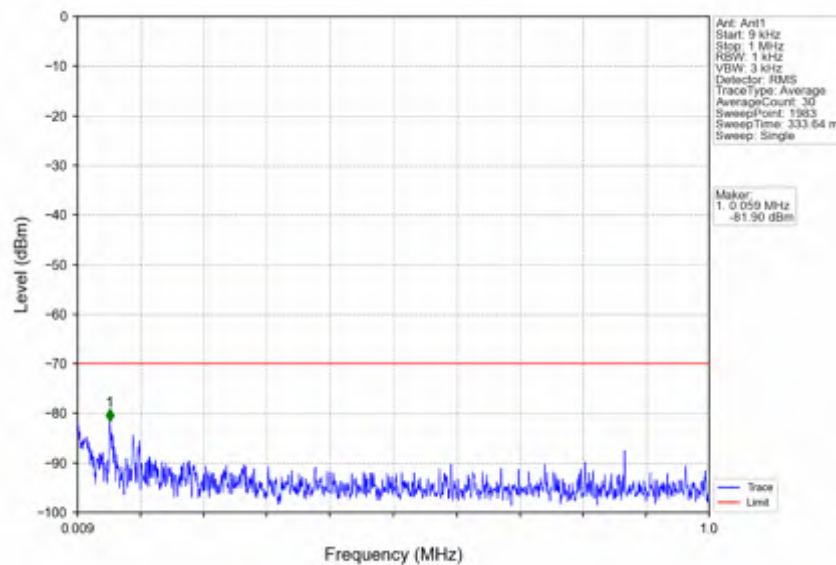
n78d_15kHz_SISO_NTNV_20MHz_DFT-s-OFDM QPSK_3625.005MHz_Edge_1RB_Left
