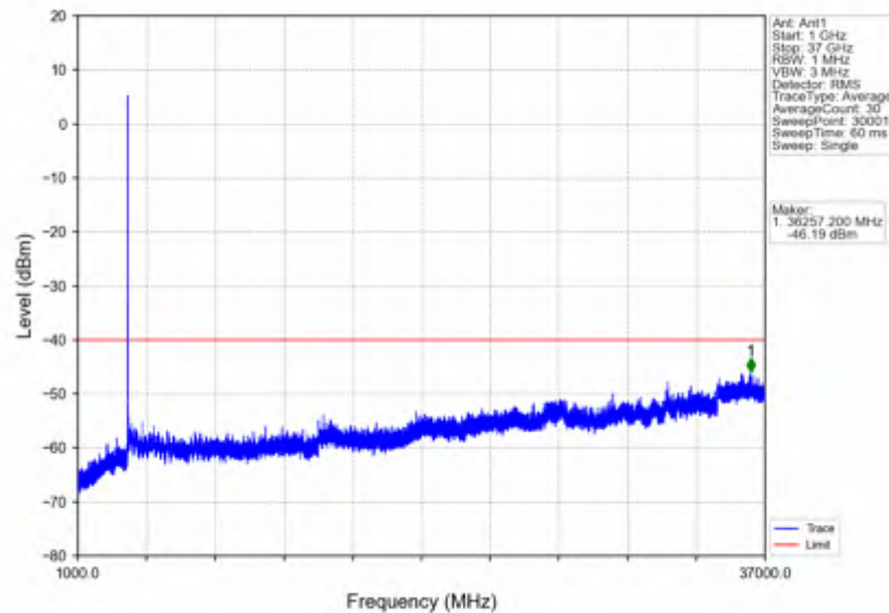
n78d_15kHz_SISO_NTNV_15MHz_CP-OFDM_QPSK_3625.005MHz_Edge_1RB_Left
