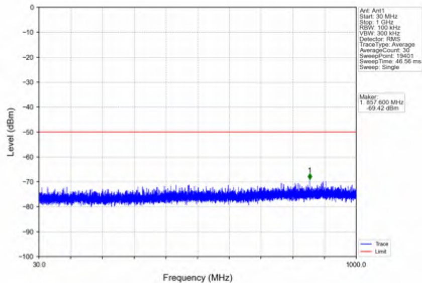
n78d_15kHz_SISO_NTNV_15MHz_DFT-s-OFDM QPSK_3692.49MHz_Edge_1RB_Right
