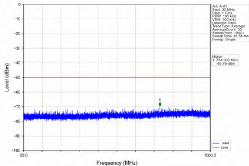
n78d_15kHz_SISO_NTNV_20MHz_DFT-s-OFDM_QPSK_3690MHz_Inner_1RB_Right
