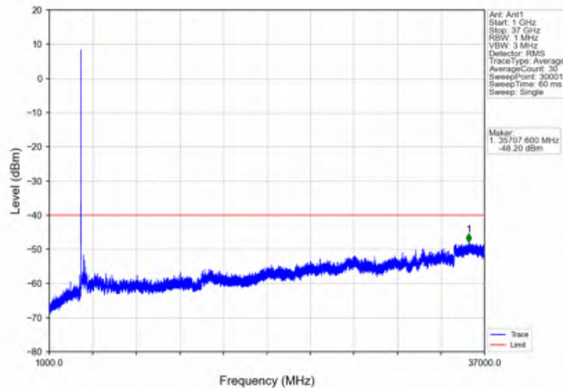
n78d_15kHz_SISO_NTNV_10MHz_CP-OFDM QPSK_3625.005MHz_Edge_1RB_Left
