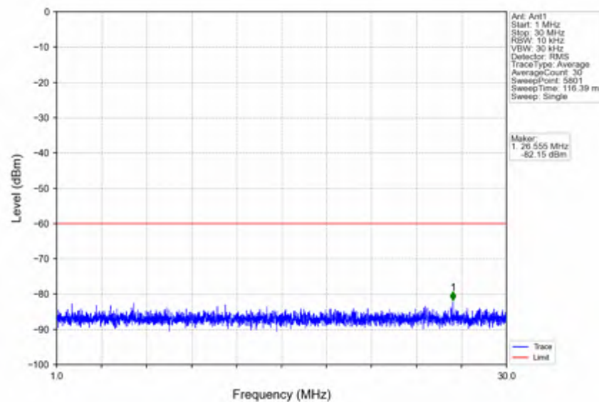
n78d_15kHz_SISO_NTNV_10MHz_DFT-s-OFDM_QPSK_3555MHz_Outer_Full
