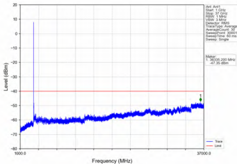
n78d_15kHz_SISO_NTNV_10MHz_DFT-s-OFDM QPSK_3694.995MHz_Edge_1RB_Right
