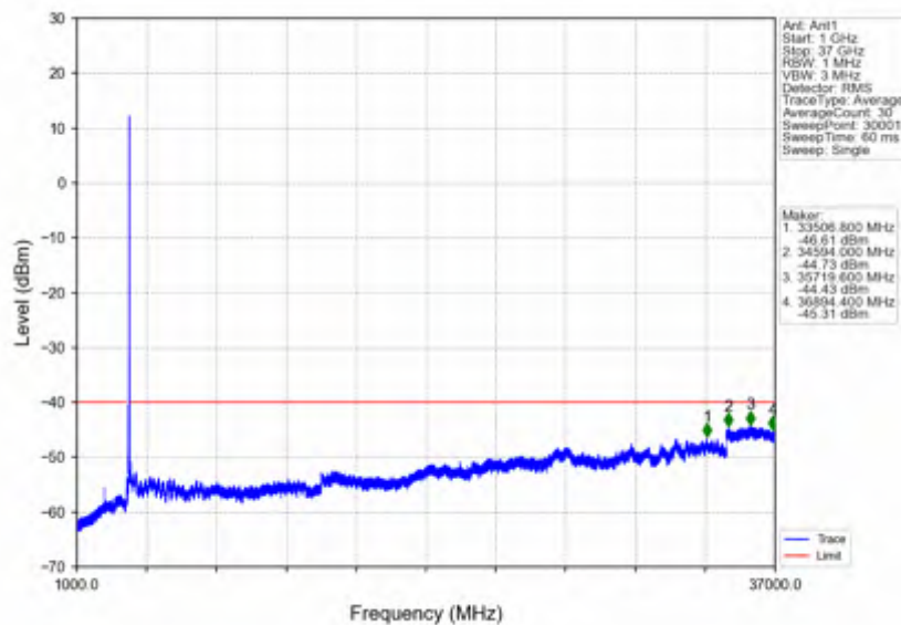
n78d 15kHz SISO NTN 20MHz CP-OFDM QPSK 3690MHz Outer Full
