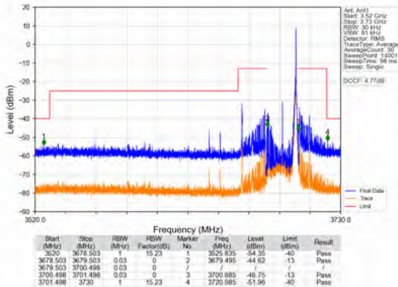
n78d_15kHz_SISO_NTNV_20MHz_DFT-s-OFDM_QPSK_3690MHz_Inner_1RB_Right
