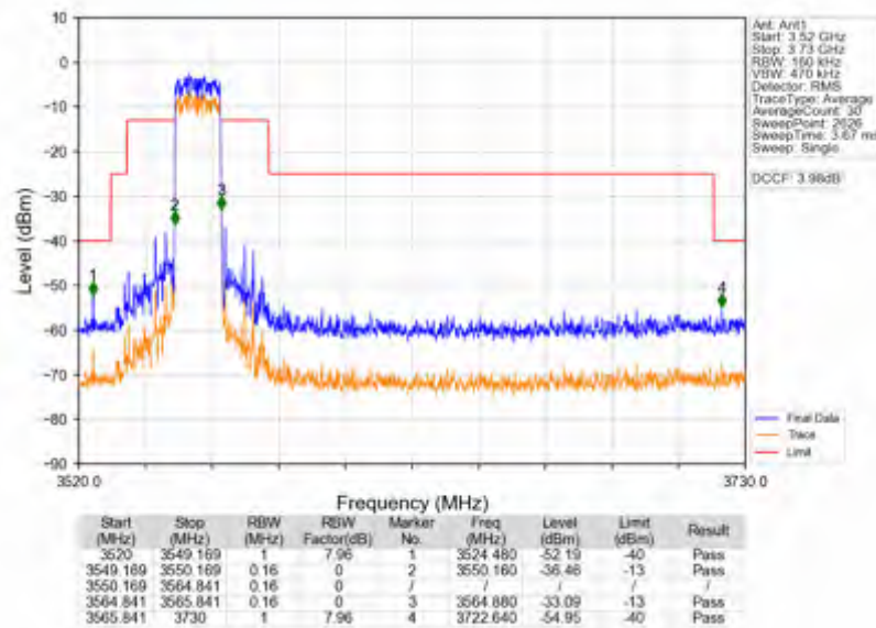
n78d_15kHz_SISO_NTNV_15MHz_CP-OFDM QPSK_3557.505MHz_Outer_Full
