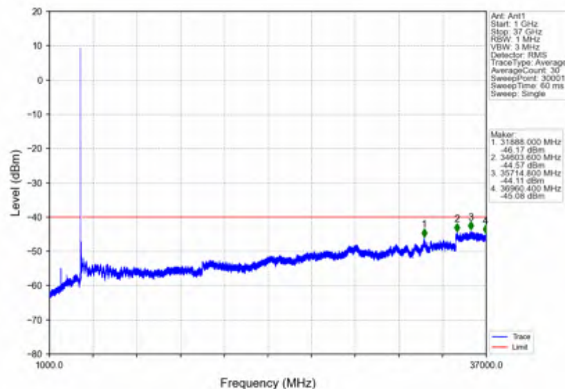
n78d_15kHz_SISO_NTNV_10MHz_DFT-s-OFDM PI/2 BPSK_3555MHz_Outer_Full
