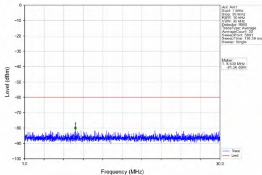
n78d_15kHz_SISO_NTNV_15MHz_CP-OFDM QPSK_3557.505MHz_Edge_1RB_Left
