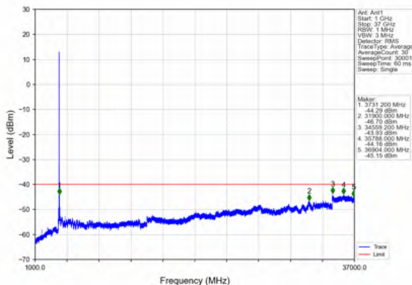
n78d_15kHz_SISO_NTNV_10MHz_DFT-s-OFDM PI/2 BPSK_3694.995MHz_Outer_Full
