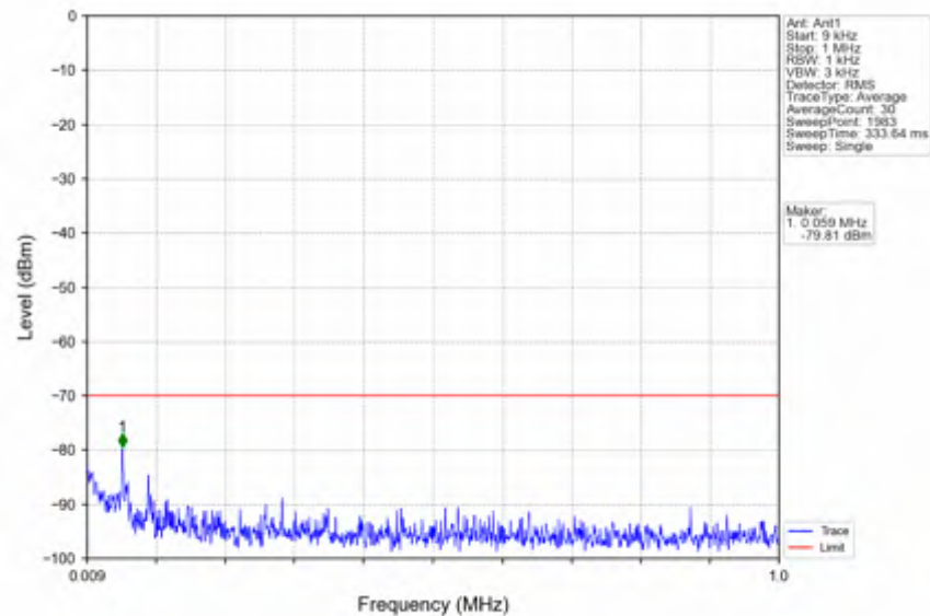
n78d_15kHz_SISO_NTNV_15MHz_CP-OFDM_QPSK_3625.005MHz_Edge_1RB_Left
