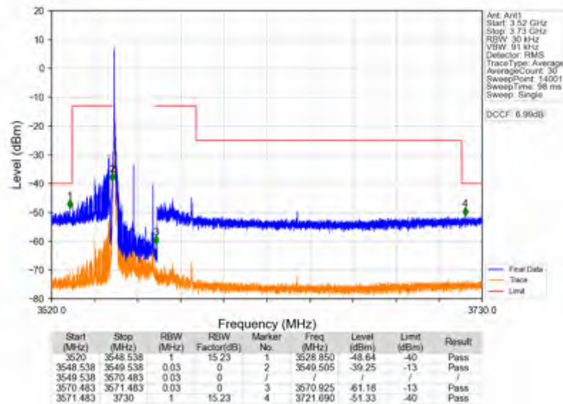
n78d_15kHz_SISO_NTNV_20MHz_DFT-s-OFDM PI/2 BPSK_3560.01MHz_Edge_1RB_Left
