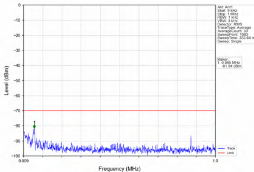
n78d_15kHz_SISO_NTNV_15MHz_CP-OFDM_QPSK_3557.505MHz_Inner_1RB_Left
