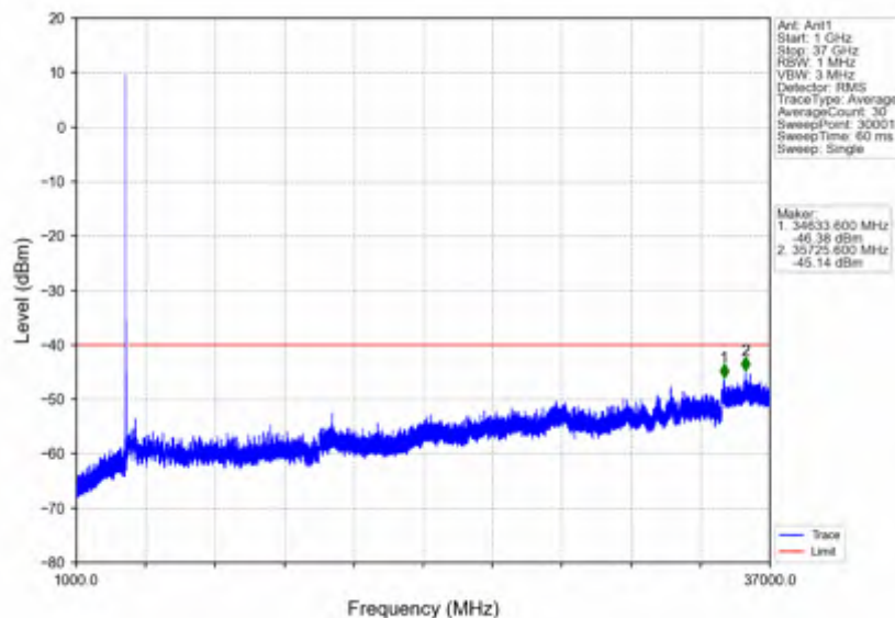
n78d_15kHz_SISO_NTV_20MHz_CP-OFDM QPSK_3625.005MHz_Edge_1RB_Left
