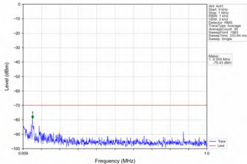
n78d_15kHz_SISO_NTNV_20MHz_DFT-s-OFDM QPSK_3690MHz_Edge_1RB_Right
