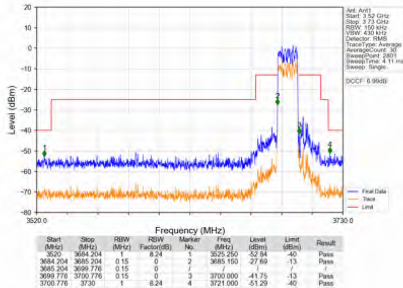
n78d_15kHz_SISO_NTNV_15MHz_DFT-s-OFDM_QPSK_3692.49MHz_Outer_Full
