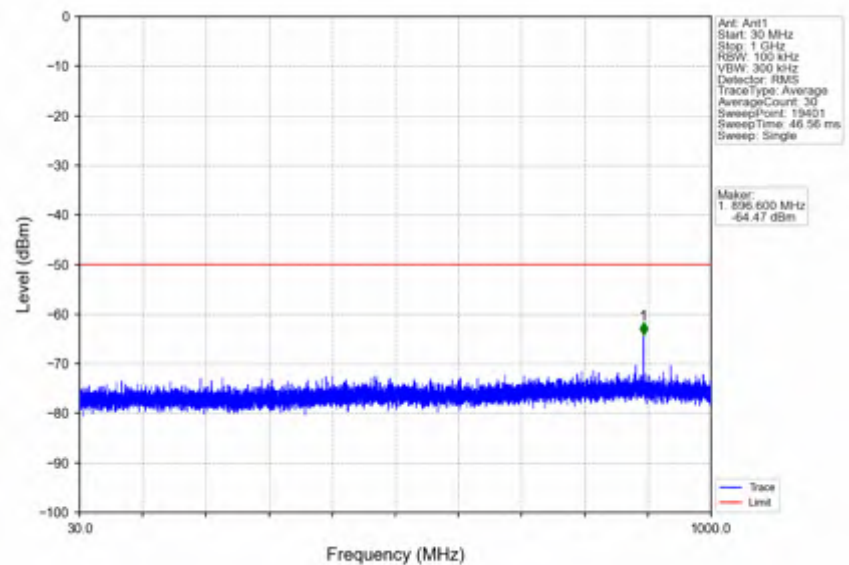
n78d_15kHz_SISO_NTNV_10MHz_DFT-s-OFDM QPSK_3625.005MHz_Edge_1RB_Left
