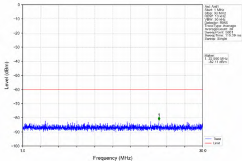
n78d_15kHz_SISO_NTNV_15MHz_DFT-s-OFDM_QPSK_3557.505MHz_Inner_1RB_Left
