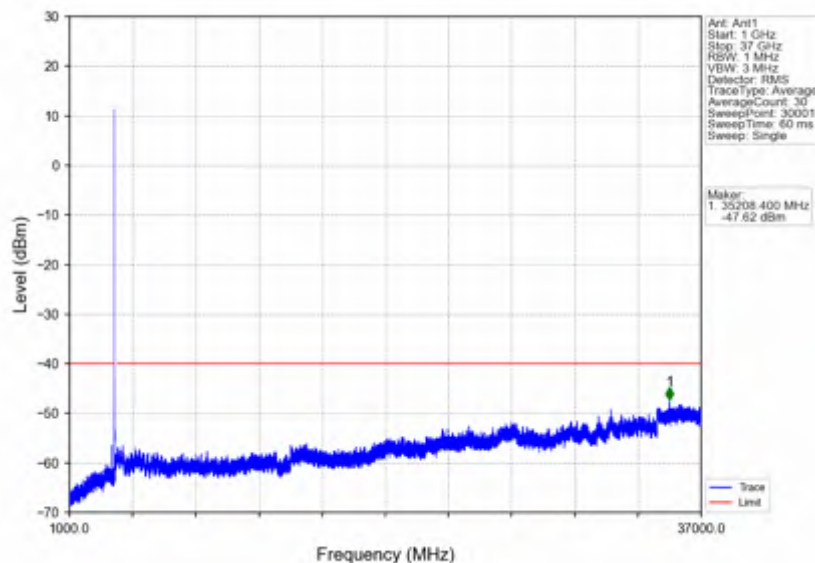
n78d_15kHz_SISO_NTNV_10MHz_CP-OFDM QPSK_3555MHz_Outer_Full
