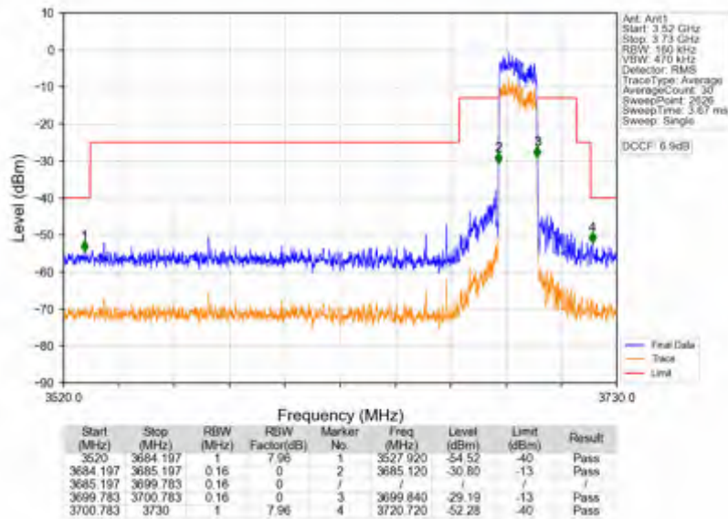
n78d_15kHz_SISO_NTNV_15MHz_CP-OFDM QPSK_3692.49MHz_Outer_Full
