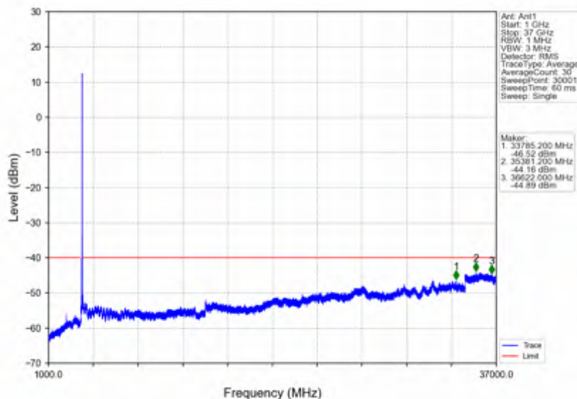
n78d_15kHz_SISO_NTNV_20MHz_DFT-s-OFDM QPSK_3560.01MHz_Edge_1RB_Left
