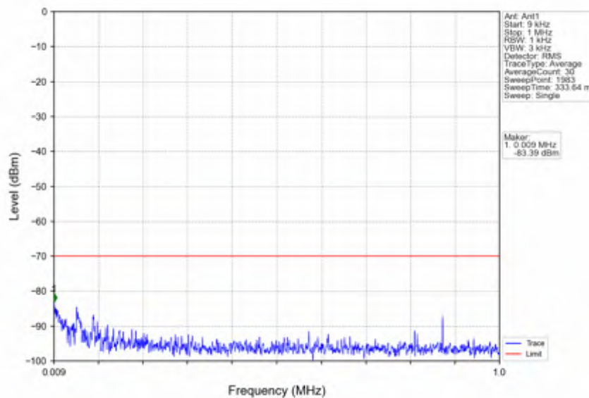
n78d_15kHz_SISO_NTNV_10MHz_CP-OFDM_QPSK_3694.995MHz_Inner_1RB_Right
