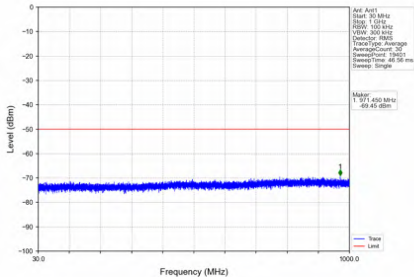
n78d_15kHz_SISO_NTNV_20MHz_CP-OFDM_QPSK_3690MHz_Outer_Full
