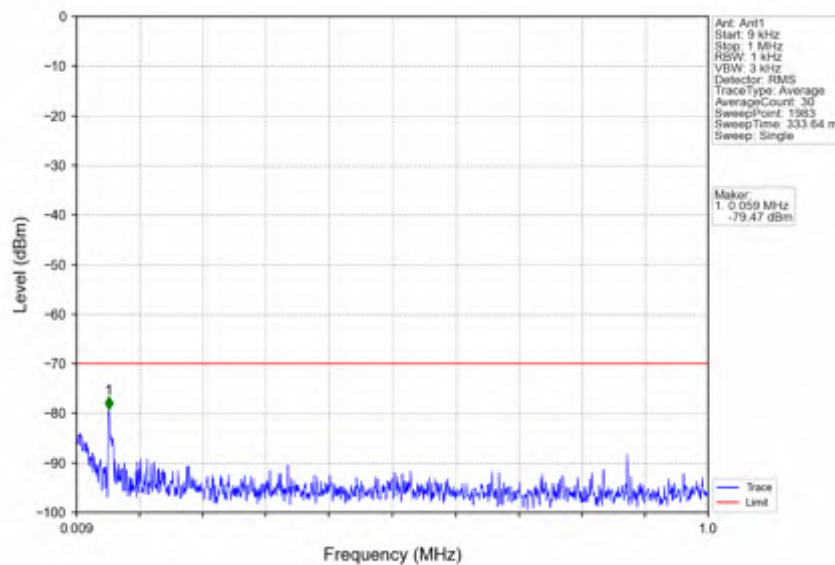
n78d_15kHz_SISO_NTNV_15MHz_DFT-s-OFDM QPSK_3557.505MHz_Outer_Full
