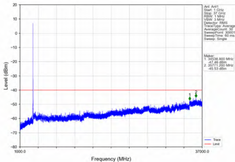
n78d_15kHz_SISO_NTNV_20MHz_CP-OFDM_QPSK_3560.01MHz_Outer_Full
