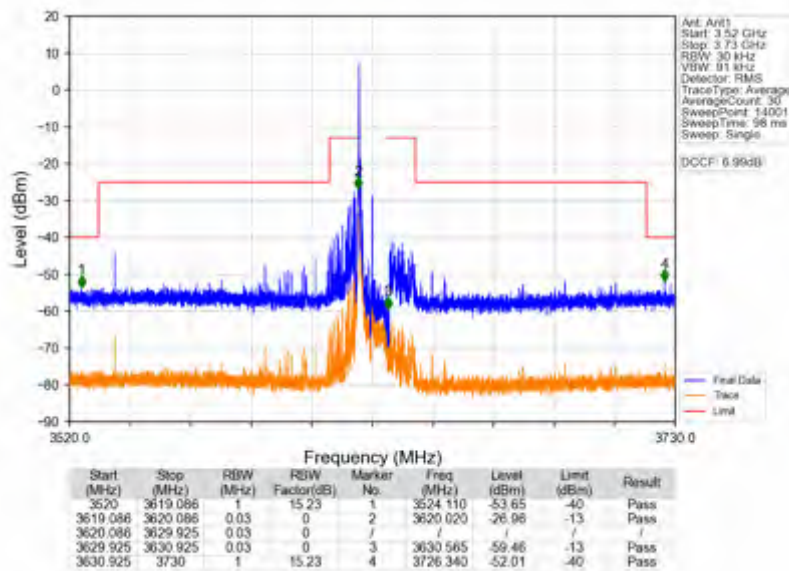
n78d_15kHz_SISO_NTNV_10MHz_CP-OFDM QPSK_3625.005MHz_Edge_1RB_Left
