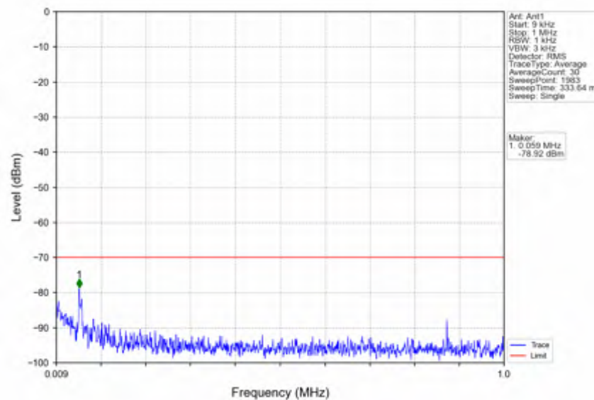
n78d_15kHz_SISO_NTNV_15MHz_CP-OFDM_QPSK_3557.505MHz_Edge_1RB_Left
