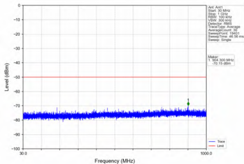
n78d_15kHz_SISO_NTNV_10MHz_DFT-s-OFDM_QPSK_3555MHz_Outer_Full
