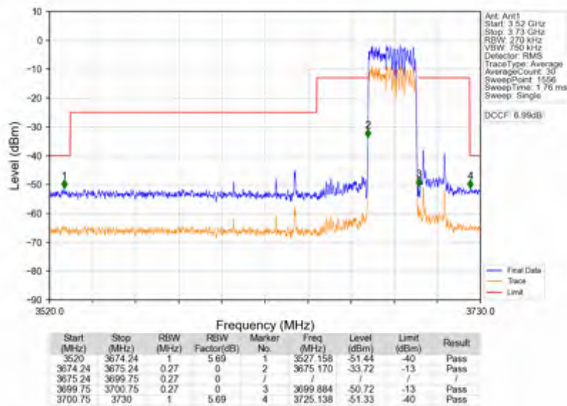
n78d 15kHz SISO NTNV 25MHz DFT-s-OFDM PI/2 BPSK 3687.495MHz Outer Full
