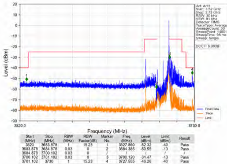
n78d_15kHz_SISO_NTNV_15MHz_DFT-s-OFDM QPSK_3692.49MHz_Edge_1RB_Right
