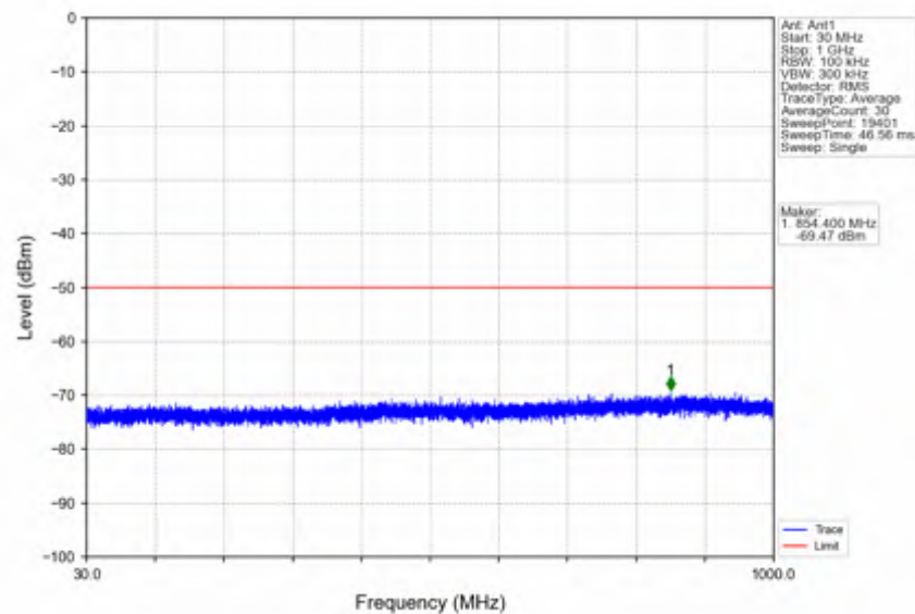
n78d_15kHz_SISO_NTNV_20MHz_DFT-s-OFDM_QPSK_3690MHz_Outer_Full
