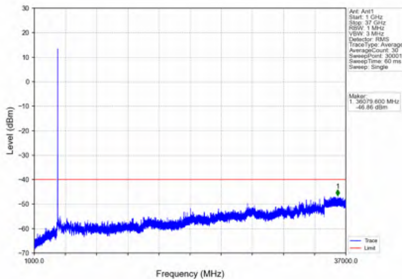
n78d_15kHz_SISO_NTNV_15MHz_CP-OFDM QPSK_3692.49MHz_Outer_Full
