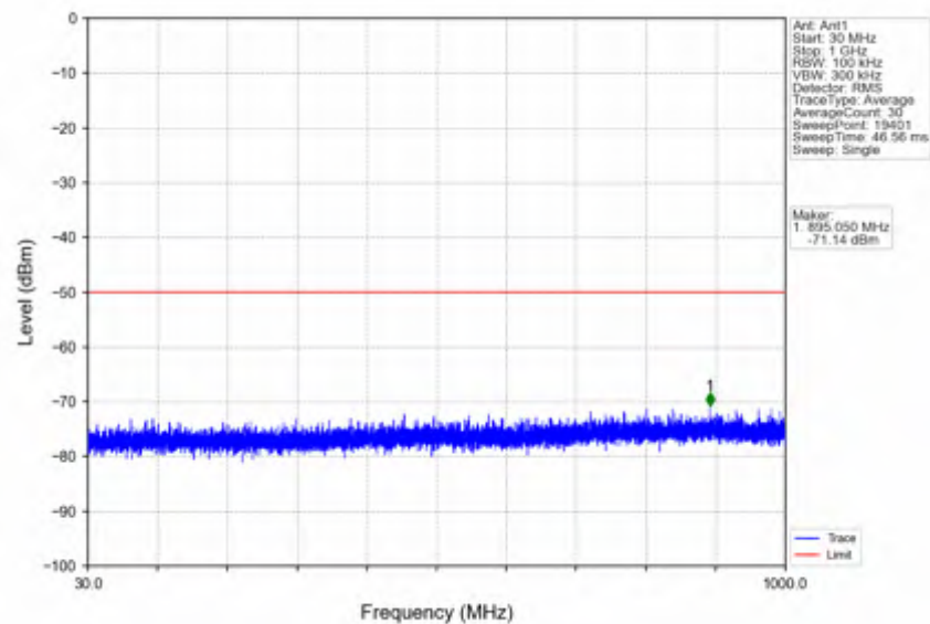
n78d_15kHz_SISO_NTNV_10MHz_CP-OFDM_QPSK_3555MHz_Edge_1RB_Left
