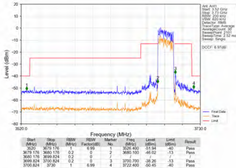
n78d_15kHz_SISO_NTNV_20MHz_DFT-s-OFDM_QPSK_3690MHz_Outer_Full
