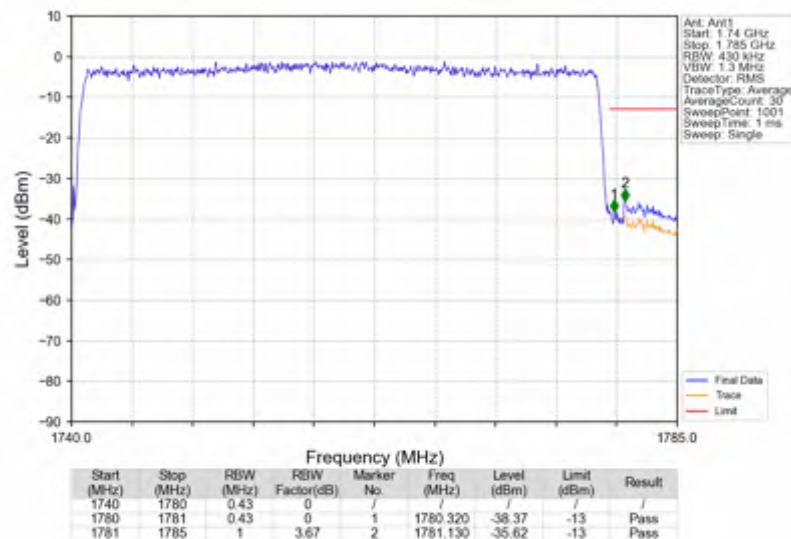
n66_30kHz_SISO_NTNV_40MHz_CP-OFDM QPSK_1760MHz_Outer_Full
