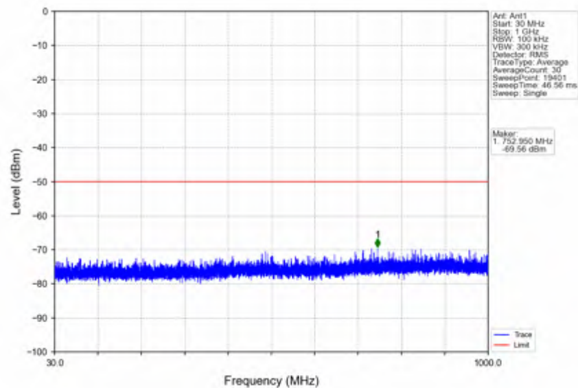
n78d_15kHz_SISO_NTNV_15MHz_CP-OFDM QPSK_3692.49MHz_Edge_1RB_Right
