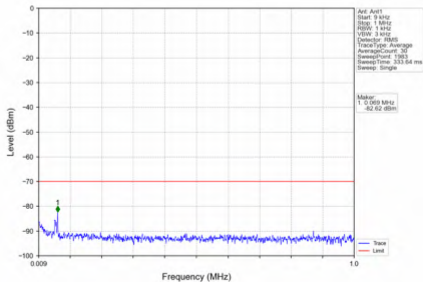
n78d_15kHz_SISO_NTNV_20MHz_CP-OFDM_QPSK_3690MHz_Outer_Full
