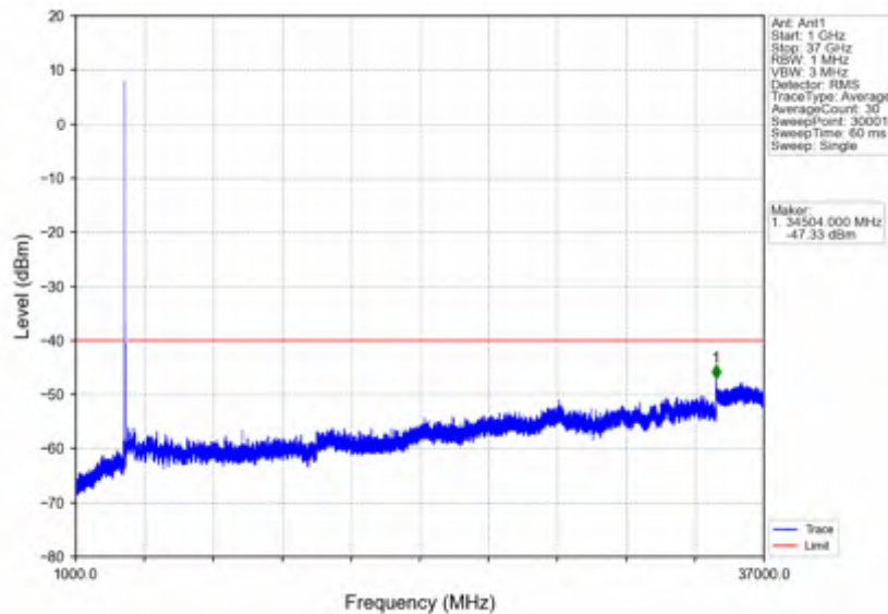
n78d_15kHz_SISO_NTNV_15MHz_DFT-s-OFDM_QPSK_3557.505MHz_Edge_1RB_Left
