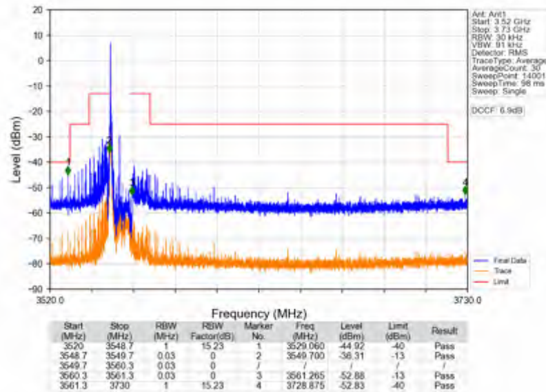
n78d_15kHz_SISO_NTNV_10MHz_CP-OFDM_QPSK_3555MHz_Edge_1RB_Left
