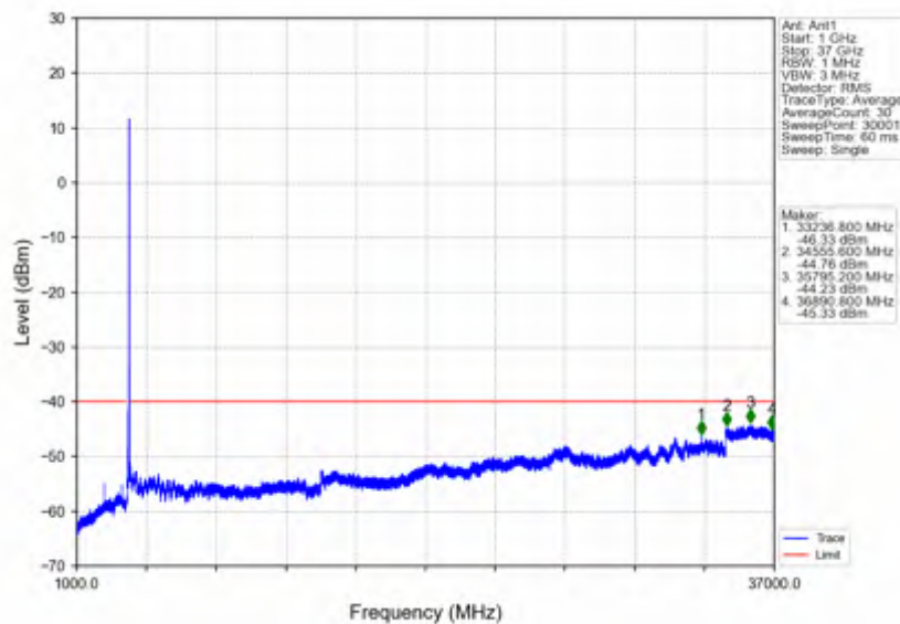
n78d_15kHz_SISO_NTNV_20MHz_DFT-s-OFDM_PI/2_BPSK_3690MHz_Outer_Full
