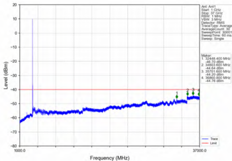
n78d_15kHz_SISO_NTNV_20MHz_DFT-s-OFDM_PI/2_BPSK_3560.01MHz_Outer_Full
