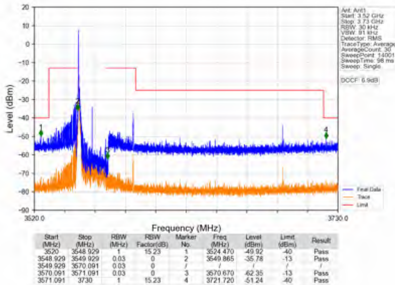
n78d_15kHz_SISO_NTNV_20MHz_DFT-s-OFDM QPSK_3560.01MHz_Edge_1RB_Left
