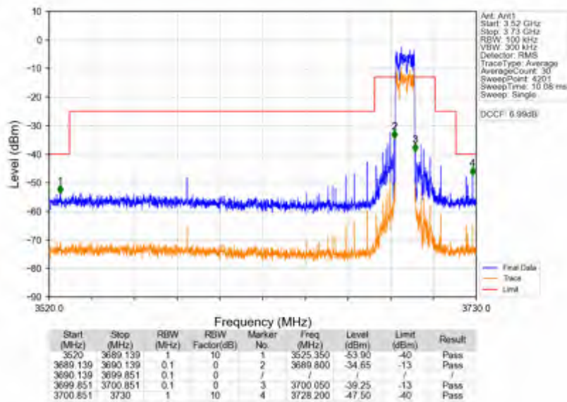
n78d_15kHz_SISO_NTNV_10MHz_CP-OFDM QPSK_3694.995MHz_Outer_Full
