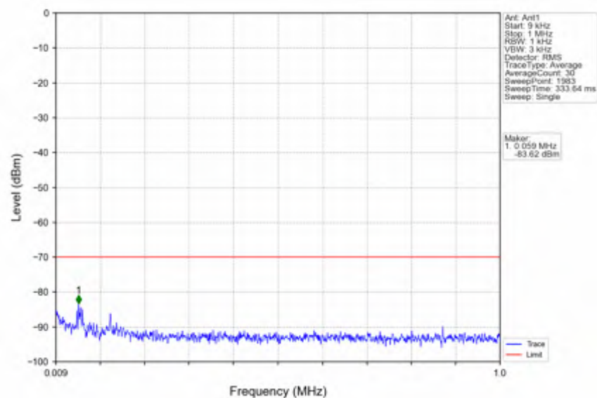
n78d_15kHz_SISO_NTNV_20MHz_DFT-s-OFDM PI/2 BPSK_3560.01MHz_Edge_1RB_Left
