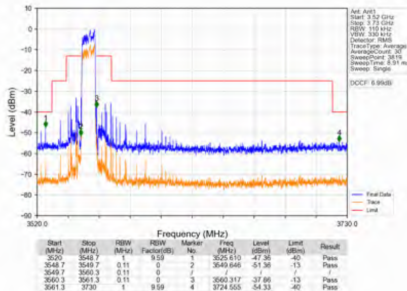
n78d_15kHz_SISO_NTNV_10MHz_DFT-s-OFDM_QPSK_3555MHz_Outer_Full
