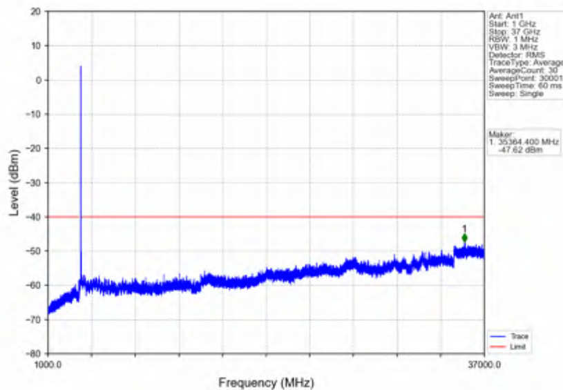
n78d_15kHz_SISO_NTNV_10MHz_DFT-s-OFDM QPSK_3694.995MHz_Inner_1RB_Right
