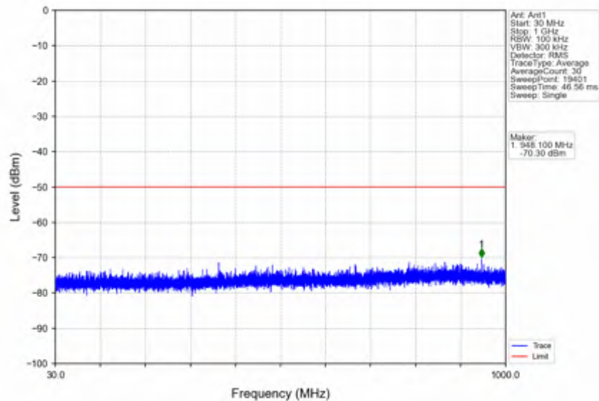
n78d_15kHz_SISO_NTNV_15MHz_DFT-s-OFDM_QPSK_3557.505MHz_Edge_1RB_Left
