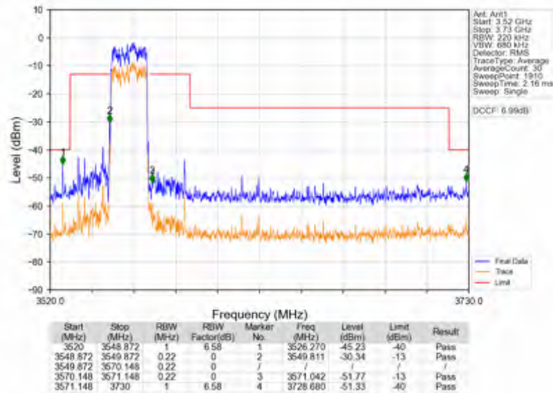
n78d_15kHz_SISO_NTNV_20MHz_DFT-s-OFDM_QPSK_3560.01MHz_Outer_Full
