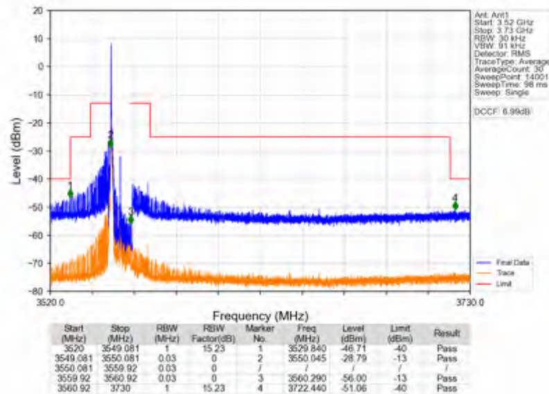
n78d_15kHz_SISO_NTNV_10MHz_DFT-s-OFDM_PI/2_BPSK_3555MHz_Edge_1RB_Left
