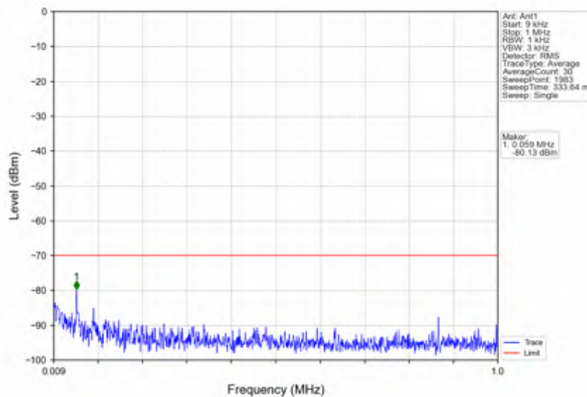
n78d_15kHz_SISO_NTNV_15MHz_DFT-s-OFDM_QPSK_3692.49MHz_Outer_Full
