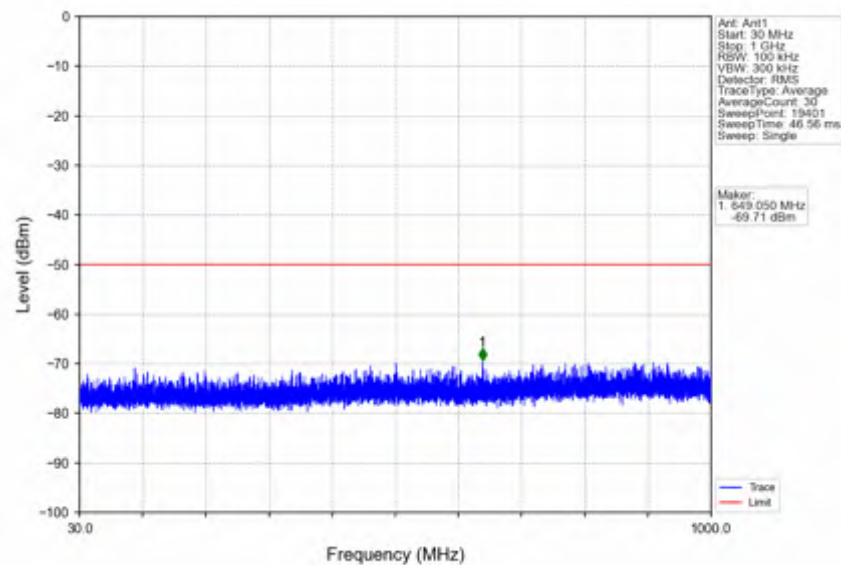
n78d_15kHz_SISO_NTNV_20MHz_DFT-s-OFDM QPSK_3625.005MHz_Edge_1RB_Left
