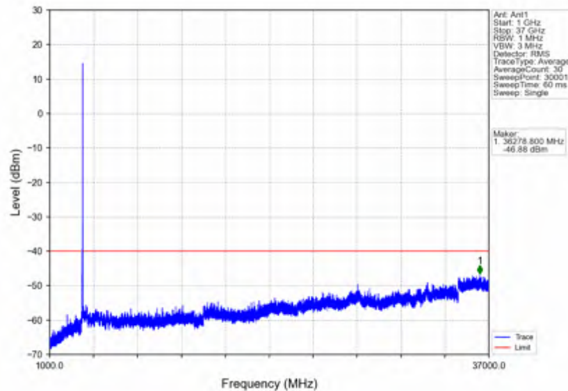
n78d_15kHz_SISO_NTNV_20MHz_DFT-s-OFDM_QPSK_3690MHz_Inner_1RB_Right
