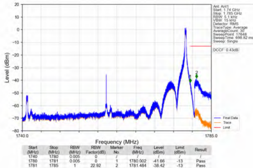
n66_30kHz_SISO_NTNV_40MHz_CP-OFDM QPSK_1760MHz_Edge_1RB_Right
