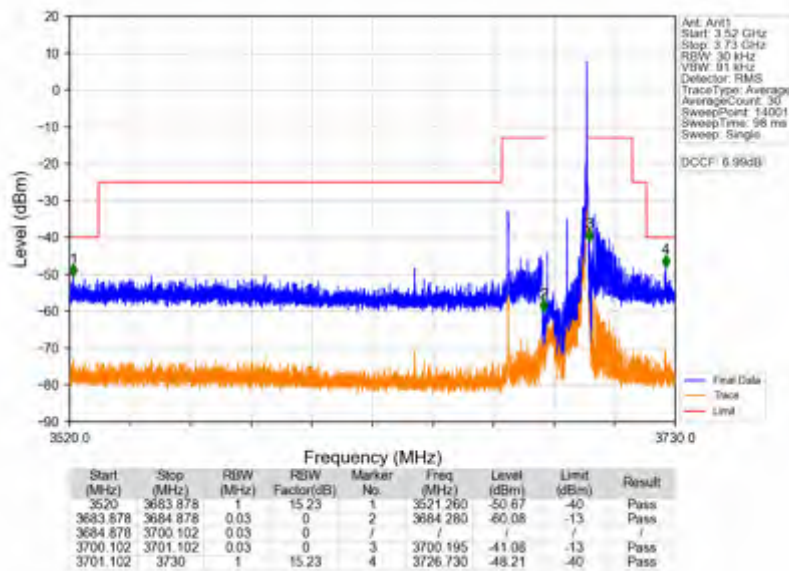
n78d_15kHz_SISO_NTNV_15MHz_DFT-s-OFDM_QPSK_3692.49MHz_Inner_1RB_Right
