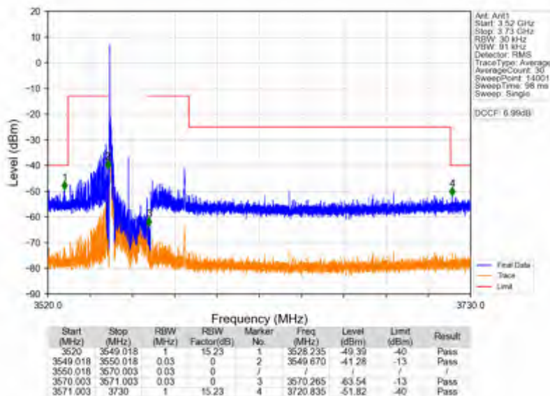
n78d_15kHz_SISO_NTNV_20MHz_DFT-s-OFDM_QPSK_3560.01MHz_Inner_1RB_Left
