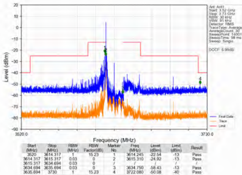
n78d_15kHz_SISO_NTV_20MHz_CP-OFDM QPSK_3625.005MHz_Edge_1RB_Left
