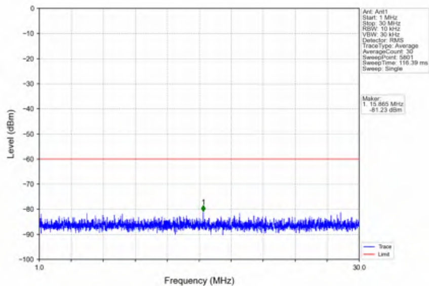
n78d_15kHz_SISO_NTNV_15MHz_DFT-s-OFDM QPSK_3692.49MHz_Edge_1RB_Right
