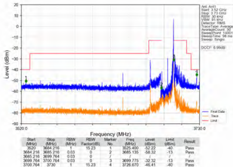
n78d_15kHz_SISO_NTNV_15MHz_CP-OFDM_QPSK_3692.49MHz_Inner_1RB_Right
