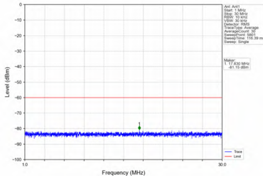
n78d_15kHz_SISO_NTNV_20MHz_CP-OFDM QPSK_3690MHz_Edge_1RB_Right
