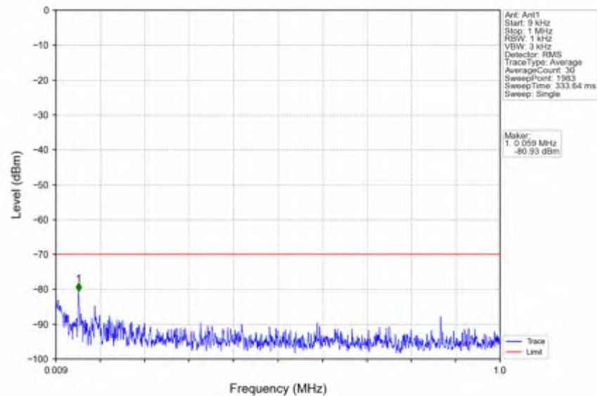
n78d_15kHz_SISO_NTNV_15MHz_DFT-s-OFDM QPSK_3692.49MHz_Inner_1RB_Right
