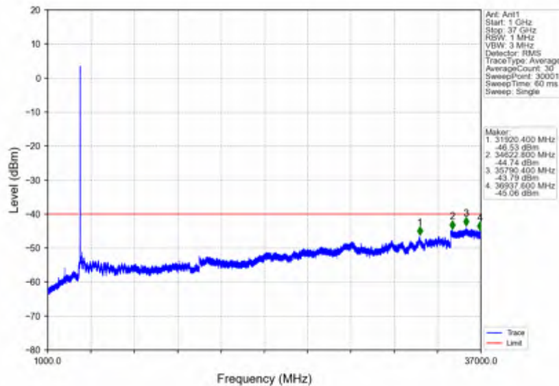
n78d_15kHz_SISO_NTNV_20MHz_CP-OFDM_QPSK_3690MHz_Outer_Full
