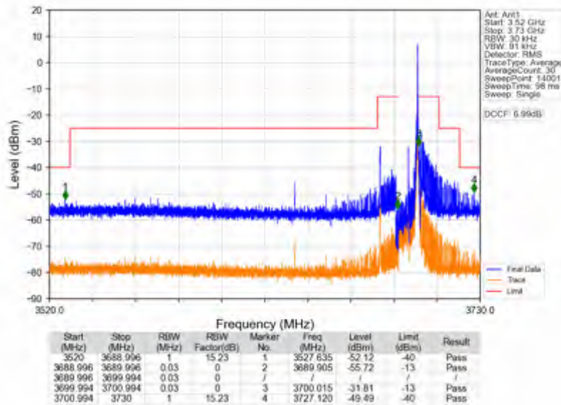
n78d_15kHz_SISO_NTNV_10MHz_DFT-s-OFDM QPSK_3694.995MHz_Edge_1RB_Right
