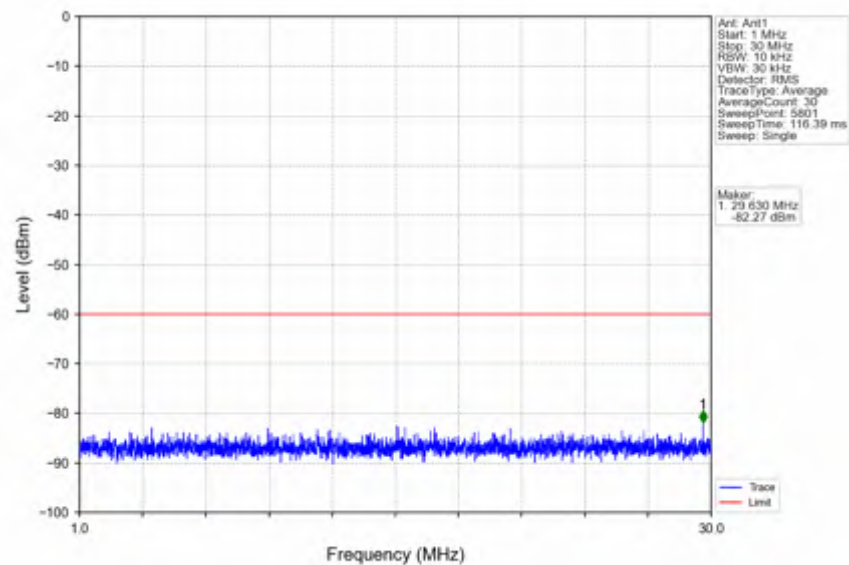
n78d_15kHz_SISO_NTNV_10MHz_CP-OFDM QPSK_3625.005MHz_Edge_1RB_Left
