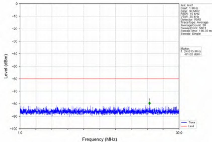
n78d_15kHz_SISO_NTNV_15MHz_CP-OFDM_QPSK_3692.49MHz_Inner_1RB_Right
