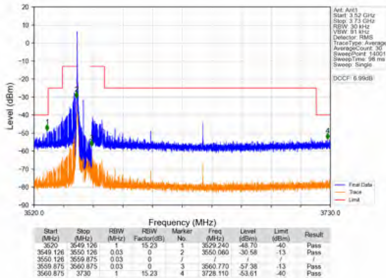
n78d_15kHz_SISO_NTNV_10MHz_DFT-s-OFDM_QPSK_3555MHz_Inner_1RB_Left
