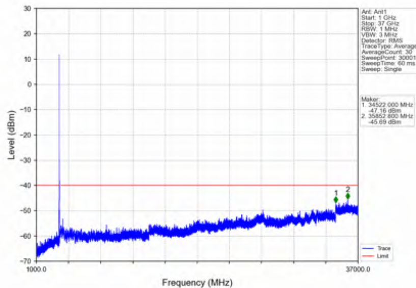
n78d_15kHz_SISO_NTNV_15MHz_CP-OFDM QPSK_3557.505MHz_Outer_Full
