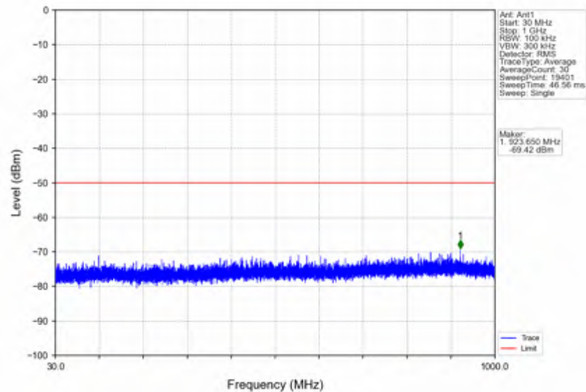
n78d_15kHz_SISO_NTNV_15MHz_CP-OFDM QPSK_3557.505MHz_Outer_Full
