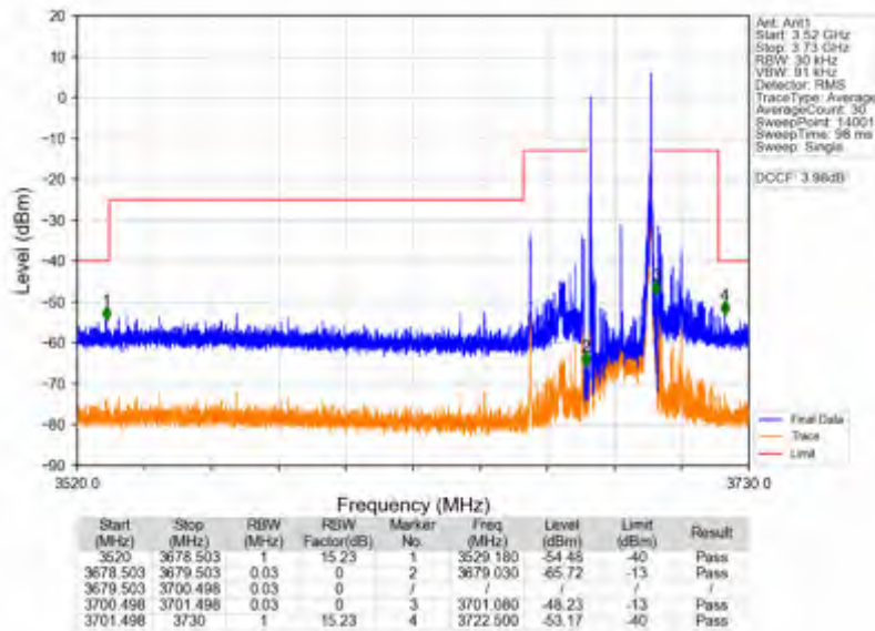
n78d_15kHz_SISO_NTNV_20MHz_DFT-s-OFDM QPSK_3690MHz_Edge_1RB_Right
