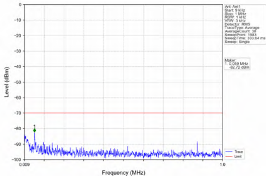
n78d_15kHz_SISO_NTNV_10MHz_CP-OFDM_QPSK_3555MHz_Outer_Full
