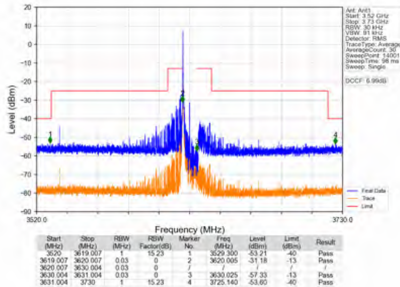
n78d_15kHz_SISO_NTNV_10MHz_DFT-s-OFDM QPSK_3625.005MHz_Edge_1RB_Left
