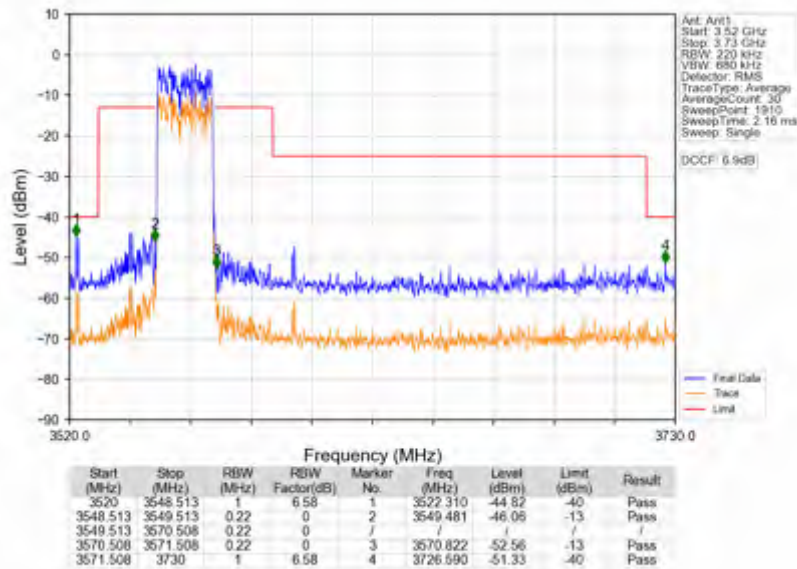
n78d_15kHz_SISO_NTNV_20MHz_CP-OFDM_QPSK_3560.01MHz_Outer_Full
