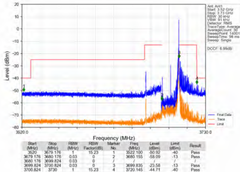
n78d_15kHz_SISO_NTNV_20MHz_CP-OFDM QPSK_3690MHz_Edge_1RB_Right
