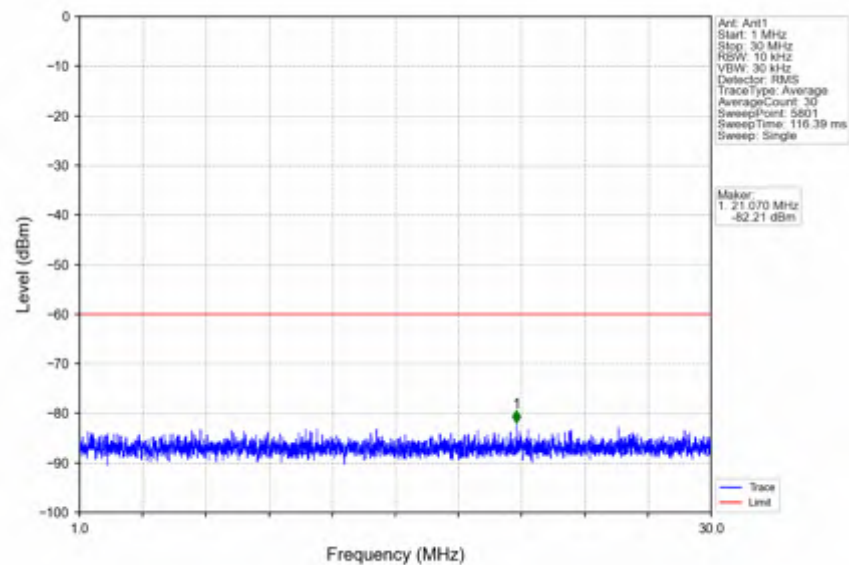
n78d_15kHz_SISO_NTNV_15MHz_DFT-s-OFDM_QPSK_3557.505MHz_Edge_1RB_Left
