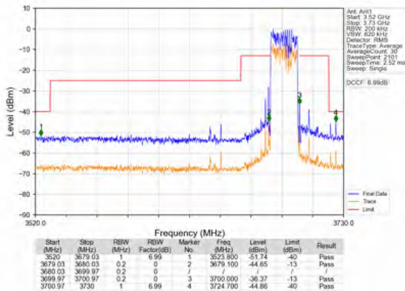
n78d_15kHz_SISO_NTNV_20MHz_DFT-s-OFDM_PI/2_BPSK_3690MHz_Outer_Full
