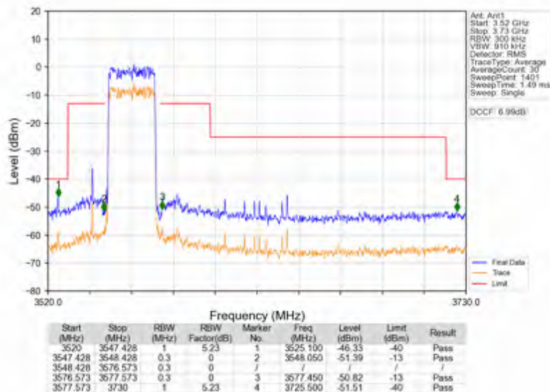
n78d_15kHz_SISO_NTNV_25MHz_DFT-s-OFDM_PI/2_BPSK_3562.5MHz_Outer_Full
