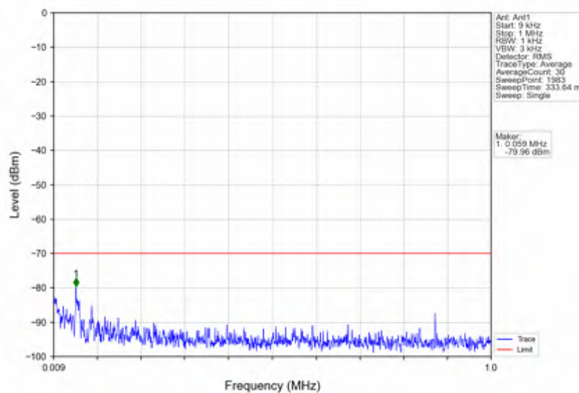
n78d_15kHz_SISO_NTNV_20MHz_CP-OFDM_QPSK_3690MHz_Inner_1RB_Right
