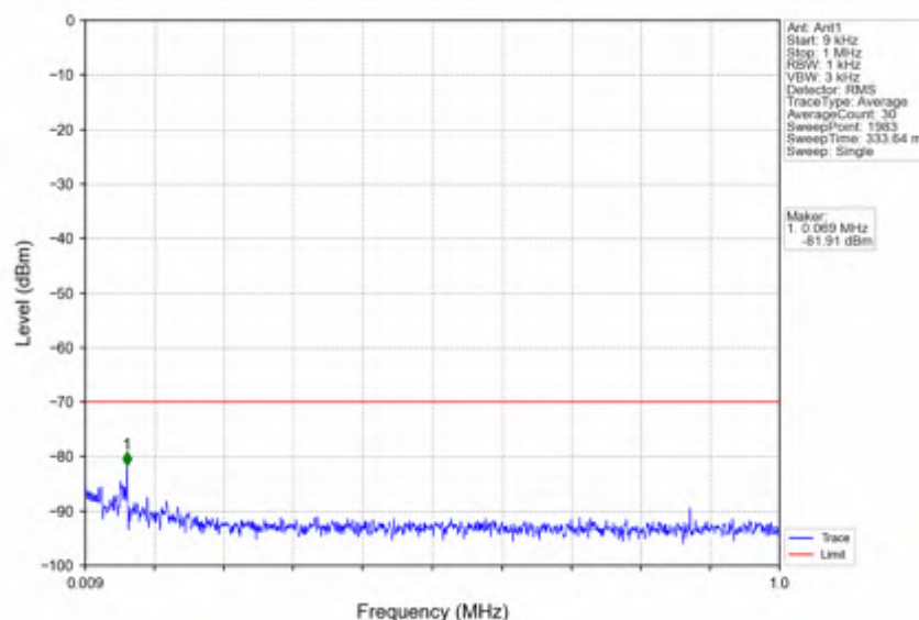
n78d_15kHz_SISO_NTNV_20MHz_CP-OFDM QPSK_3690MHz_Edge_1RB_Right
