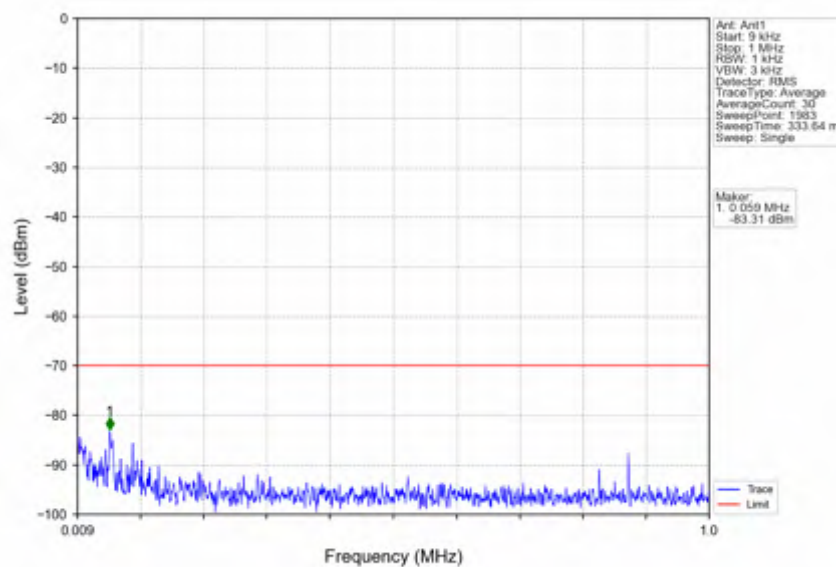
n78d_15kHz_SISO_NTNV_10MHz_DFT-s-OFDM QPSK_3625.005MHz_Edge_1RB_Left
