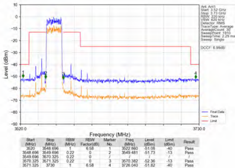
n78d_15kHz_SISO_NTNV_20MHz_DFT-s-OFDM_PI/2_BPSK_3560.01MHz_Outer_Full
