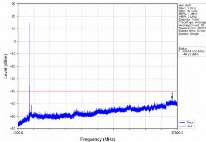
n78d_15kHz_SISO_NTNV_15MHz_DFT-s-OFDM_QPSK_3557.505MHz_Inner_1RB_Left
