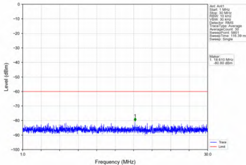
n78d_15kHz_SISO_NTNV_15MHz_DFT-s-OFDM QPSK_3625.005MHz_Edge_1RB_Left
