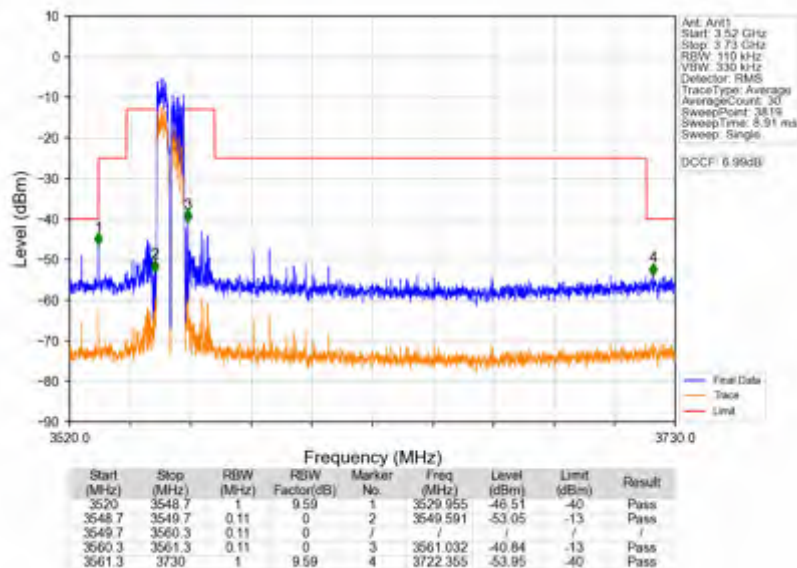
n78d_15kHz_SISO_NTNV_10MHz_CP-OFDM QPSK_3555MHz_Outer_Full
