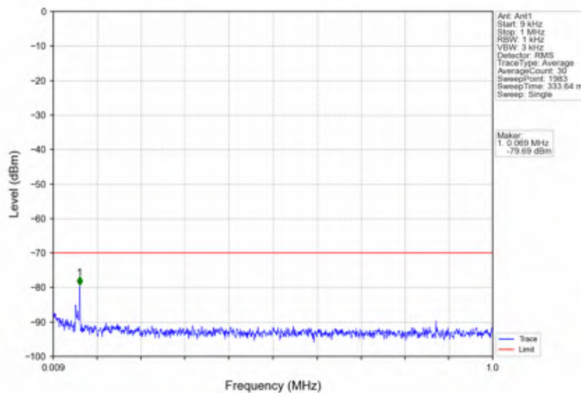
n78d_15kHz_SISO_NTNV_20MHz_DFT-s-OFDM_QPSK_3690MHz_Outer_Full
