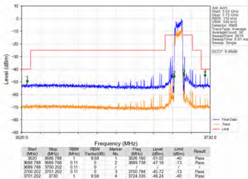
n78d_15kHz_SISO_NTNV_10MHz_DFT-s-OFDM PI/2 BPSK_3694.995MHz_Outer_Full
