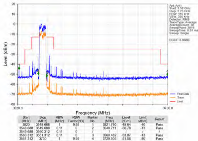
n78d_15kHz_SISO_NTNV_10MHz_DFT-s-OFDM PI/2 BPSK_3555MHz_Outer_Full
