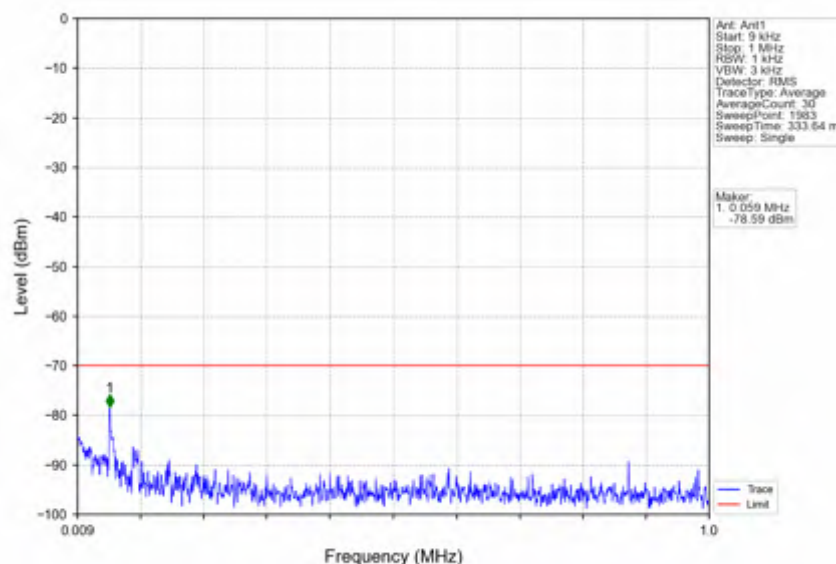
n78d_15kHz_SISO_NTNV_15MHz_CP-OFDM_QPSK_3692.49MHz_Inner_1RB_Right
