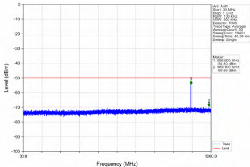
n78d_15kHz_SISO_NTNV_10MHz_DFT-s-OFDM PI/2 BPSK_3555MHz_Edge_1RB_Left
