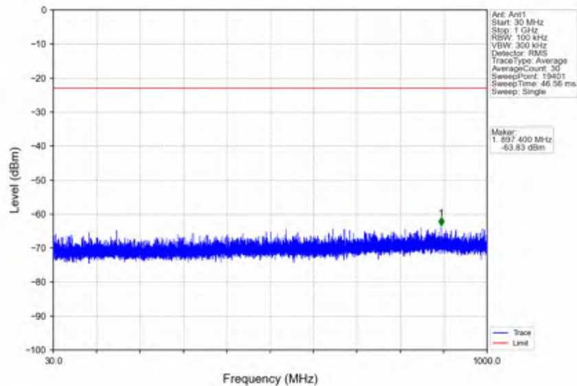
n66_30kHz_SISO_NTNV_40MHz_CP-OFDM QPSK_1760MHz_Outer_Full
