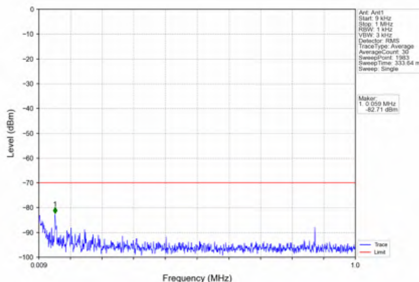
n78d_15kHz_SISO_NTNV_10MHz_DFT-s-OFDM QPSK_3694.995MHz_Outer_Full
