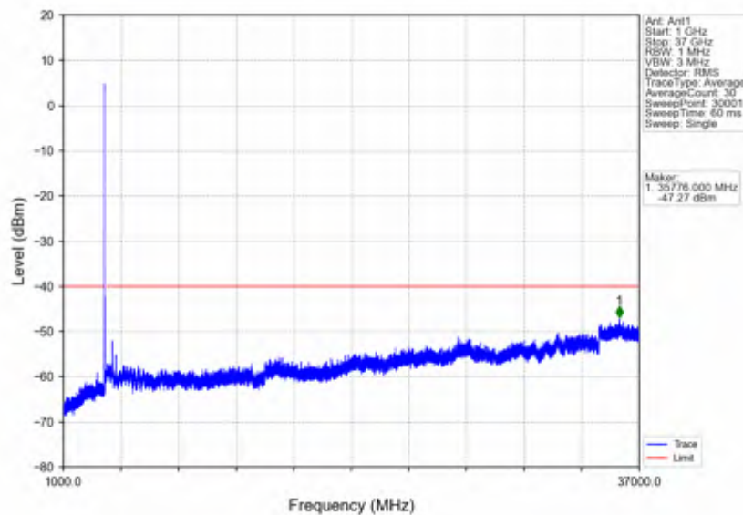
n78d 15kHz SISO NTN 10MHz CP-OFDM QPSK 3555MHz Outer Full
