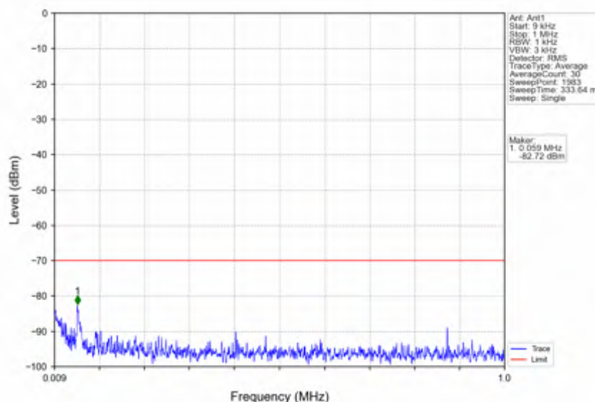
n78d_15kHz_SISO_NTNV_10MHz_DFT-s-OFDM_QPSK_3555MHz_Outer_Full
