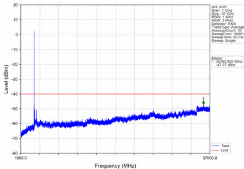
n78d_15kHz_SISO_NTNV_10MHz_DFT-s-OFDM_QPSK_3555MHz_Inner_1RB_Left
