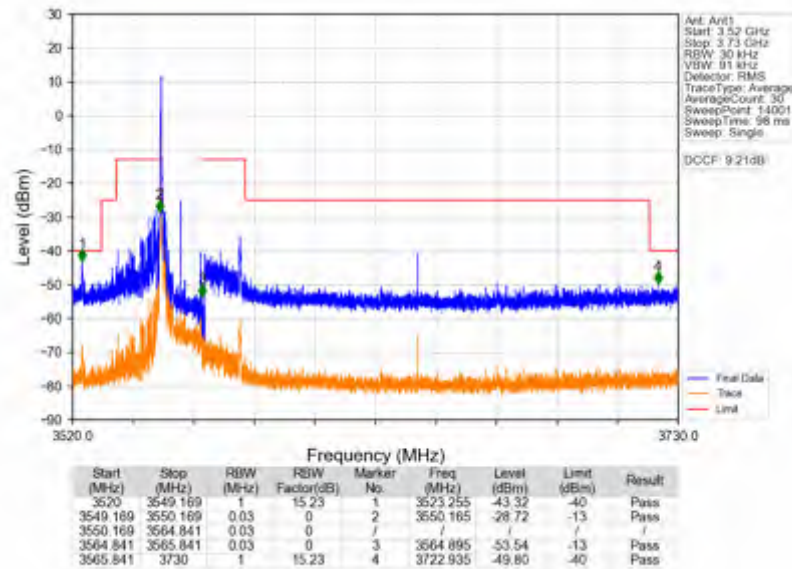
n78d_15kHz_SISO_NTNV_15MHz_CP-OFDM_QPSK_3557.505MHz_Inner_1RB_Left
