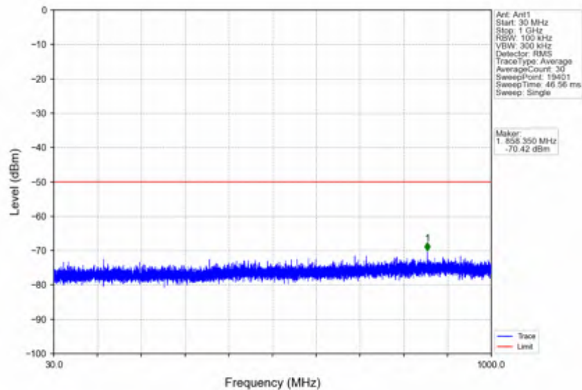
n78d_15kHz_SISO_NTNV_15MHz_DFT-s-OFDM_QPSK_3557.505MHz_Inner_1RB_Left
