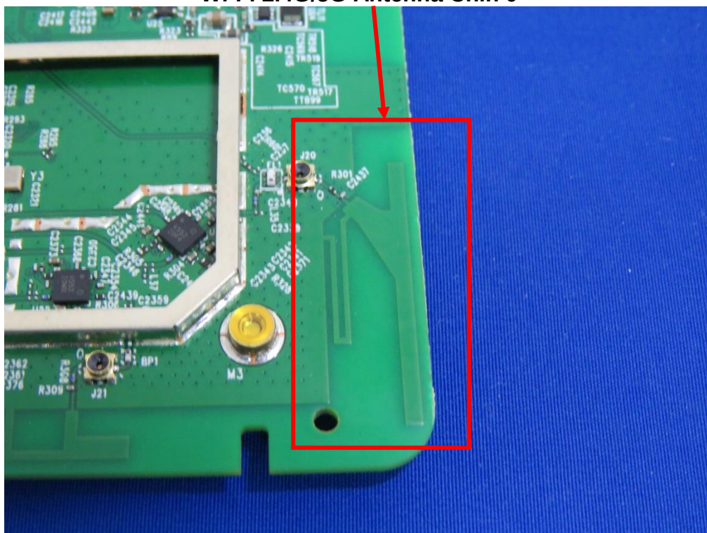
Wi-Fi 2.4G/5G Antenna Chin 0
