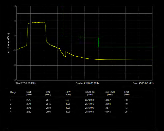
Band7 16QAM BW=10MHz Channel=21400 RB Size=27 Position=#0 Normal
