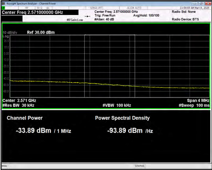
Band7 16QAM BW=20MHz Channel=21350 RB Size=27 Position=#0 Normal
