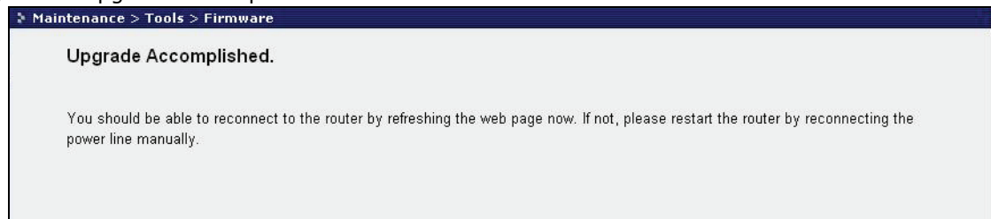
Figure 40 Upgrade Accomplished
