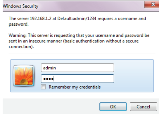
Figure 3 Login Screen
