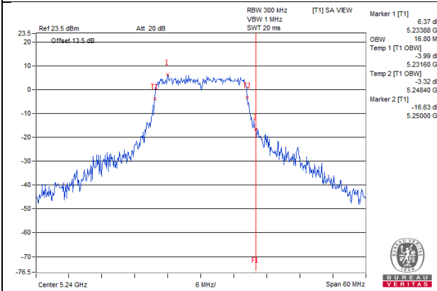
802.11ac(VHT20)_Chain0 / CH48
