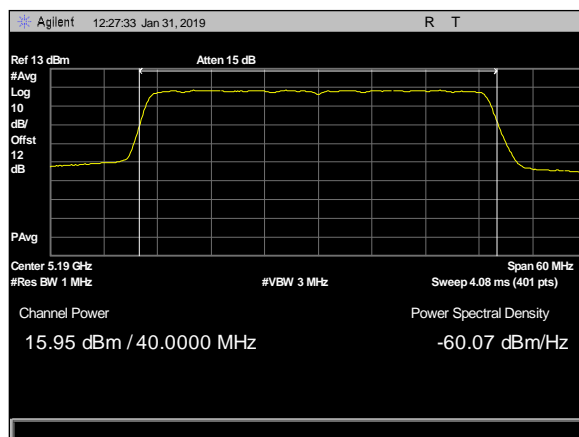
Plot 8. Output Power,5dBi- 2x2, 5190MHz, c1
