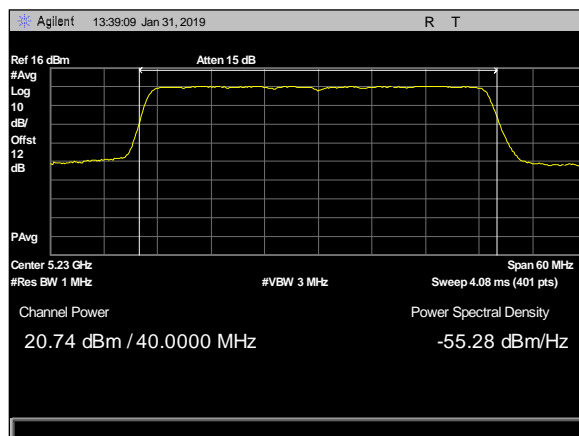
Plot 7. Output Power,2dBi- 2x2, 5230MHz, c2
