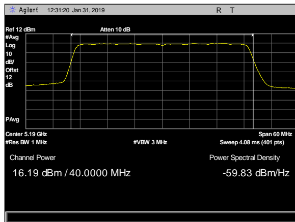
Plot 9. Output Power,5dBi- 2x2, 5190MHz, c2
