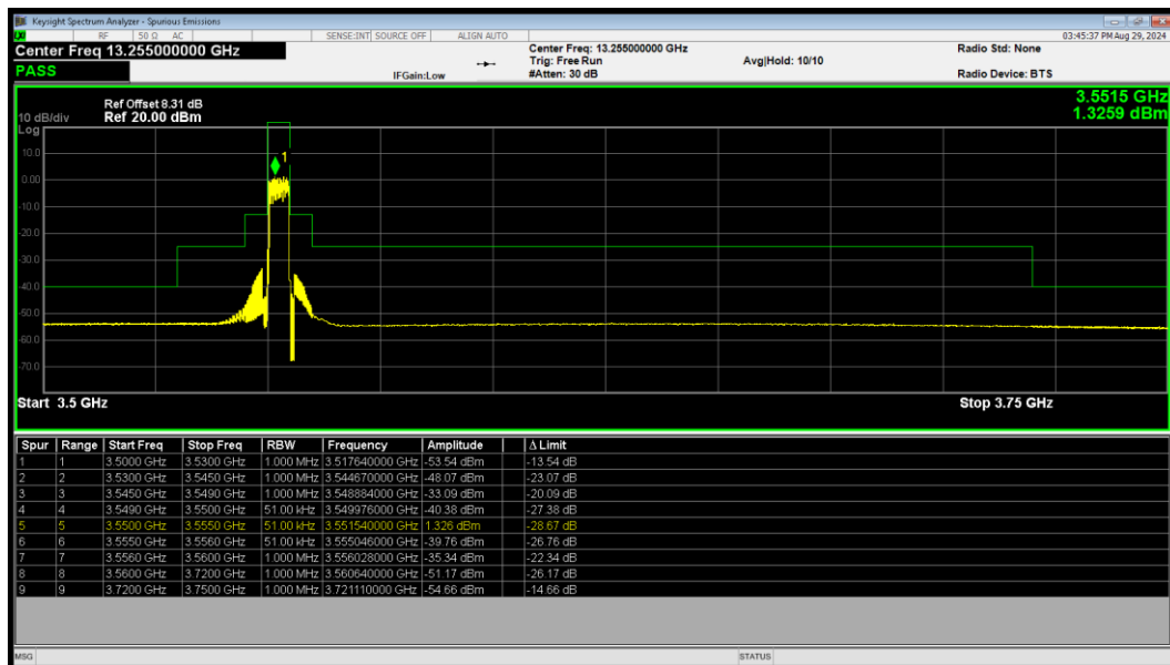
LTE Band 48 64QAM BW=5MHz LowChannel=55265 RB Size=25 Position=#0
