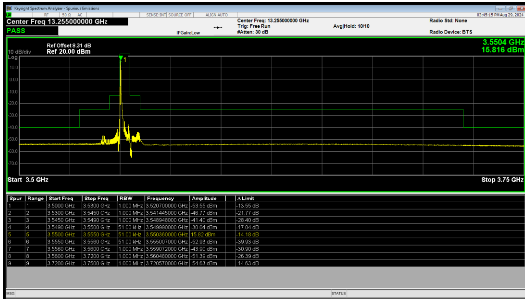
LTE Band 48 64QAM BW=5MHz LowChannel=55265 RB Size=1 Position=#0
