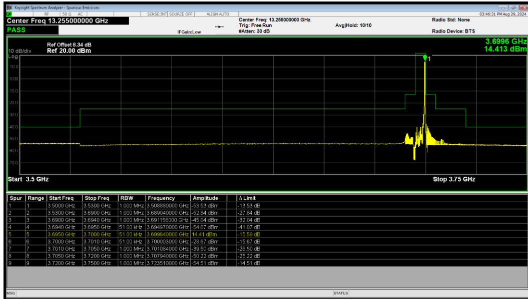
LTE Band 48 16QAM BW=5MHz HighChannel=56715 RB Size=1 Position=#Max
