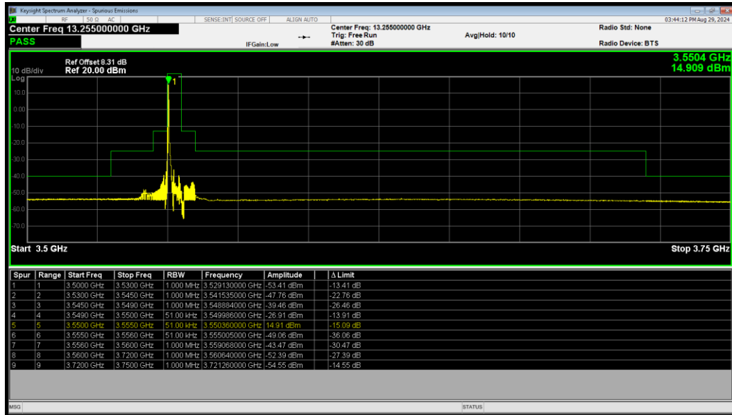
LTE Band 48 QPSK BW=5MHz LowChannel=55265 RB Size=1 Position=#0
