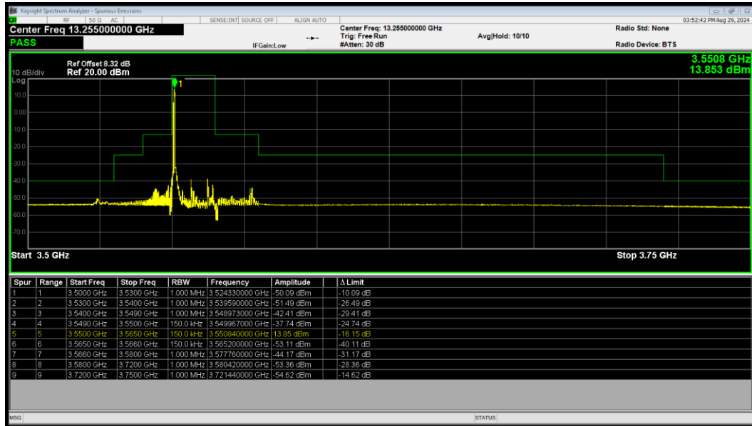
LTE Band 48 64QAM BW=15MHz LowChannel=55315 RB Size=1 Position=#0
