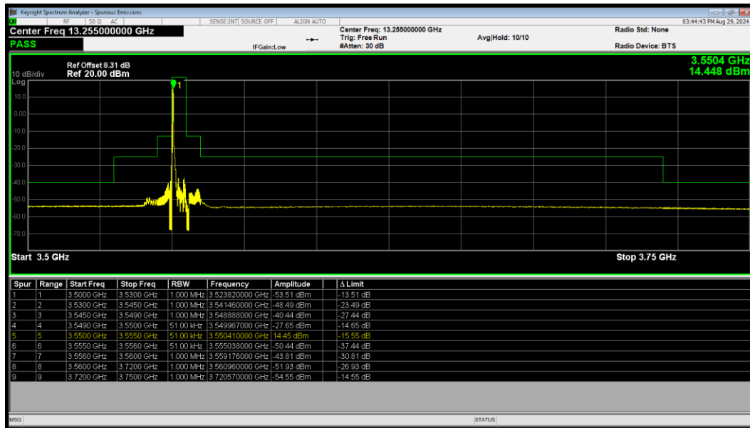
LTE Band 48 16QAM BW=5MHz LowChannel=55265 RB Size=1 Position=#0
