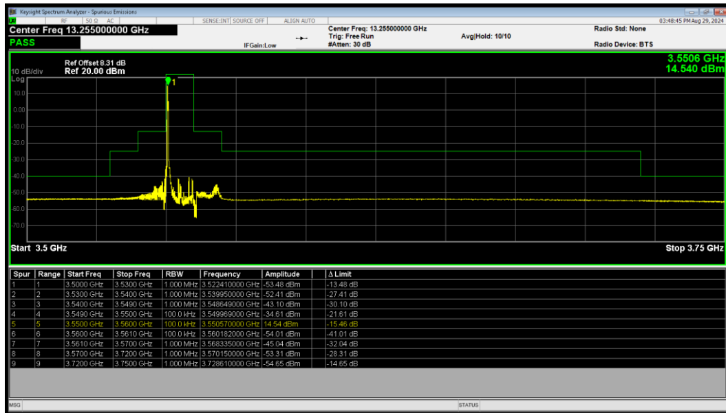
LTE Band 48 64QAM BW=10MHz LowChannel=55290 RB Size=1 Position=#0
