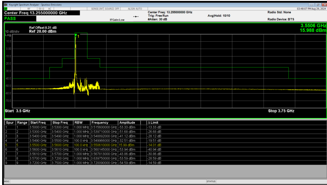
LTE Band 48 16QAM BW=10MHz LowChannel=55290 RB Size=1 Position=#0
