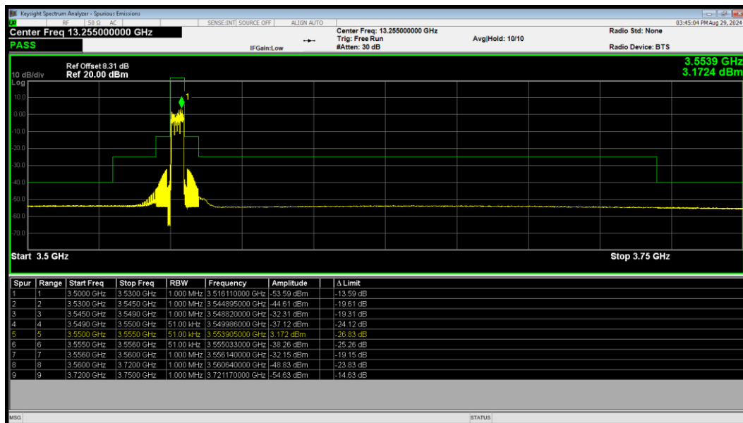
LTE Band 48 16QAM BW=5MHz LowChannel=55265 RB Size=25 Position=#0
