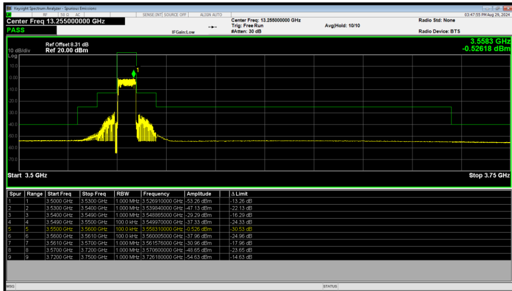
LTE Band 48 QPSK BW=10MHz LowChannel=55290 RB Size=50 Position=#0
