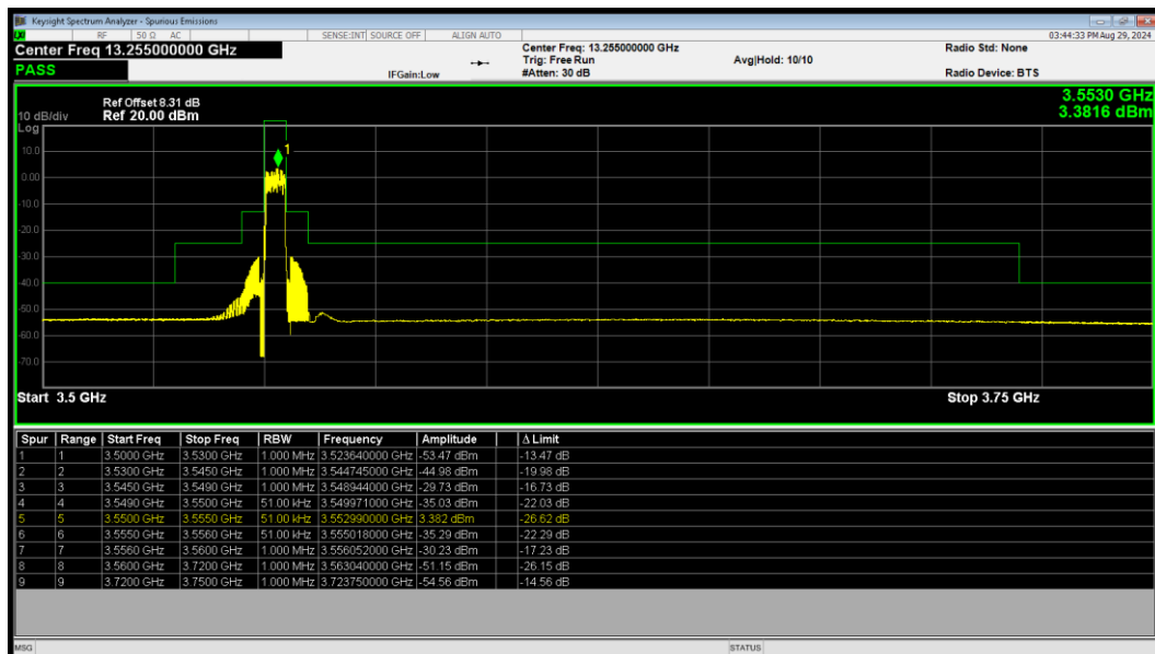
LTE Band 48 QPSK BW=5MHz LowChannel=55265 RB Size=25 Position=#0
