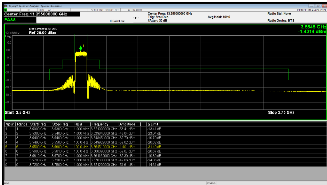
LTE Band 48 16QAM BW=10MHz LowChannel=55290 RB Size=50 Position=#0
