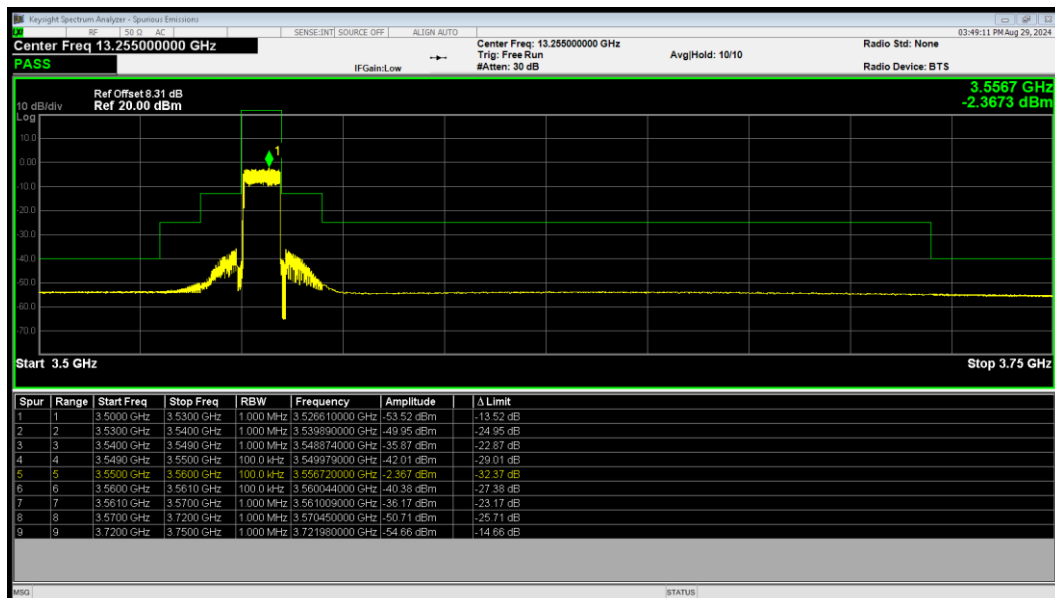
LTE Band 48 64QAM BW=10MHz LowChannel=55290 RB Size=50 Position=#0
