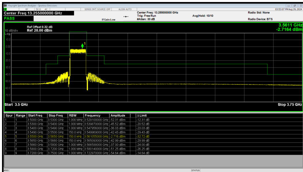
LTE Band 48 64QAM BW=15MHz LowChannel=55315 RB Size=75 Position=#0
