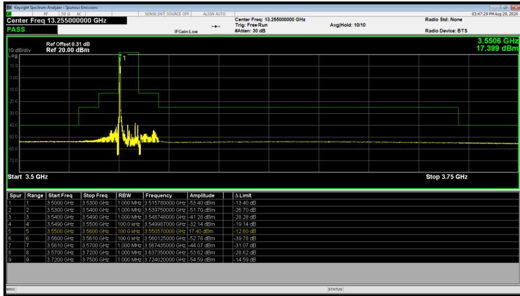
LTE Band 48 QPSK BW=10MHz LowChannel=55290 RB Size=1 Position=#0
