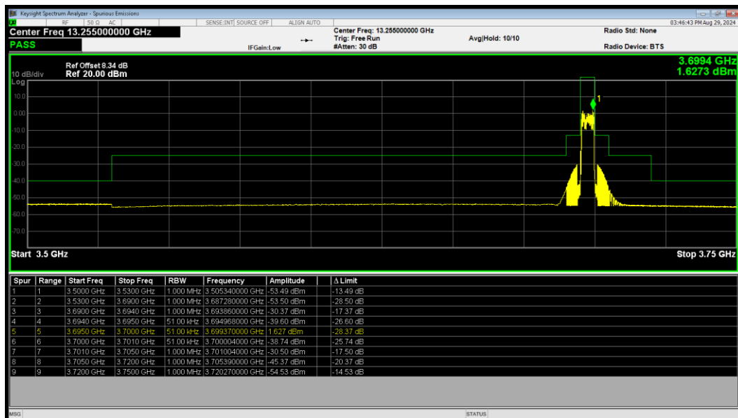
LTE Band 48 16QAM BW=5MHz HighChannel=56715 RB Size=25 Position=#0
