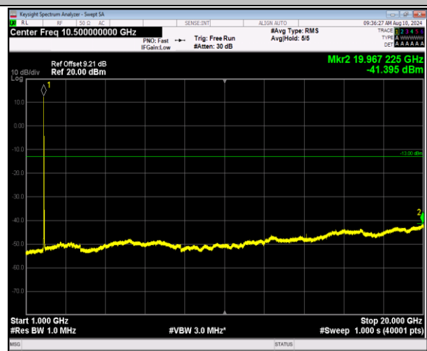
2-2-5MHz-20MHz-16QAM-16QAM-18633-18750-1RB#0-1RB#99-1000~20000MHz-PASS
