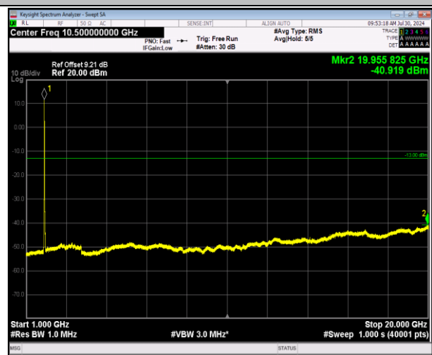
2-2-5MHz-20MHz-64QAM-64QAM-18633-18750-25RB#0-1 00RB#0-1000~20000MHz-PASS
