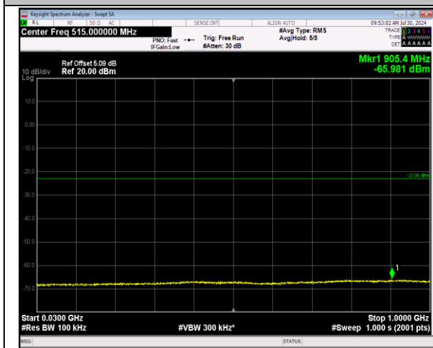
2-2-5MHz-20MHz-64QAM-64QAM-18633-18750-25RB#0 -100RB#0-30~1000MHz-PASS
