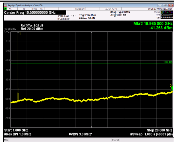
2-2-5MHz-20MHz-16QAM-16QAM-18633-18750-1RB#24-0RB#0-1000~20000MHz-PASS
