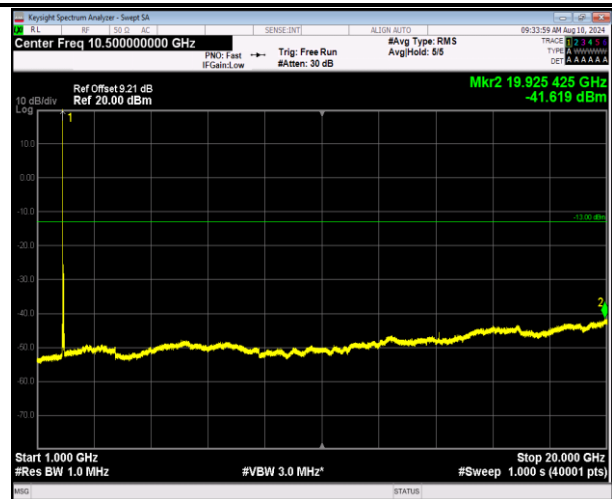
2-2-5MHz-20MHz-16QAM-16QAM-18633-18750-1RB#0-0RB#0-1000~20000MHz-PASS
