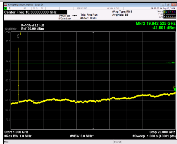
2-2-5MHz-20MHz-QPSK-QPSK-18633-18750-25RB#0-100 RB#0-1000~20000MHz-PASS
