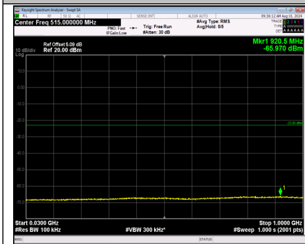
2-2-5MHz-20MHz-16QAM-16QAM-18633-18750-1RB#0-1RB#99-30~1000MHz-PASS
