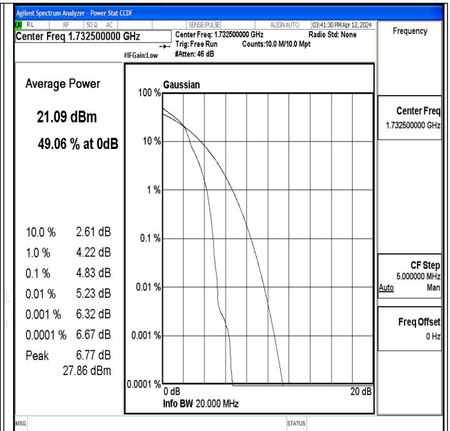
Band4-20MHz-16QAM-20175-1RB#0-PASS
