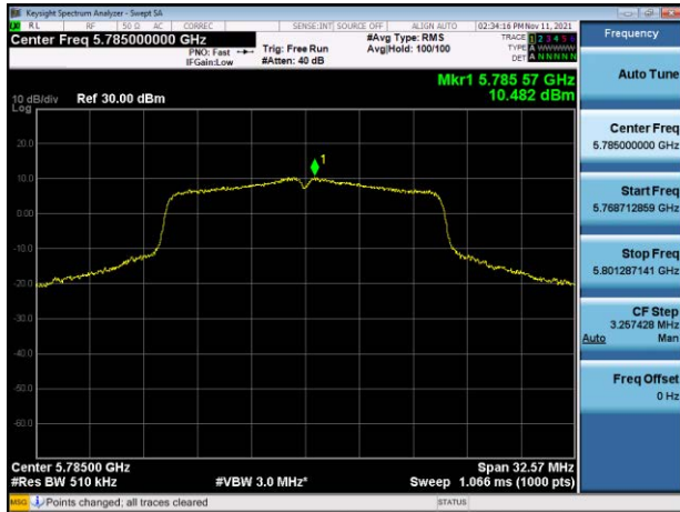
802.11n HT20 (CH 157 : 5785 MHz) – Chain 0
