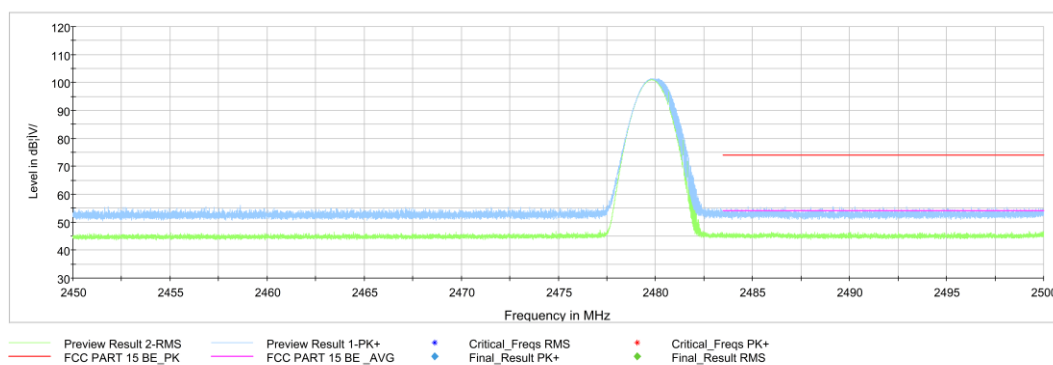
Fig.59. Frequency Band Edges: GFSK, Channel 78, Hopping Off, ch11, 2.45 GHz - 2.50GHz
