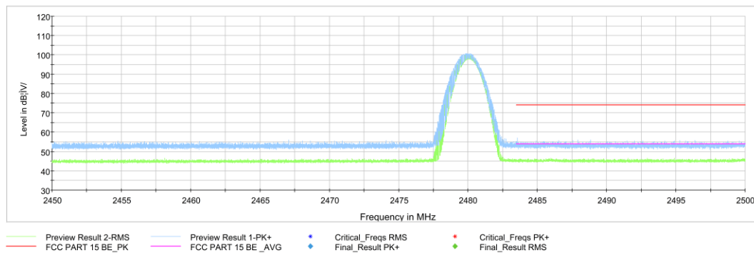
Fig.61. Frequency Band Edges: \pi/4 DQPSK, Channel 78, Hopping Off, 2.45 GHz - 2.50GHz
