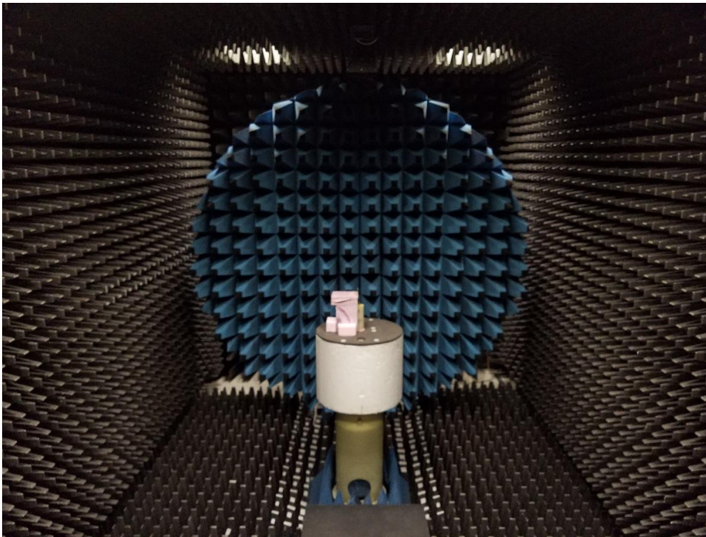
Figure 2 Antenna Chamber
