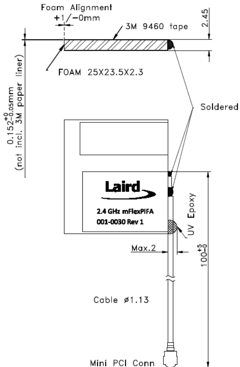
Figure 1: Physical dimensions
