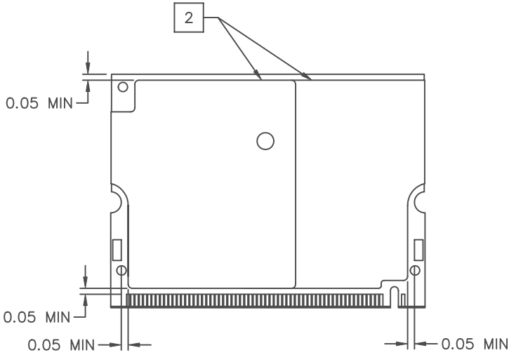
SECONDARY SIDE INSULATION PLACEMENT STEP 3
