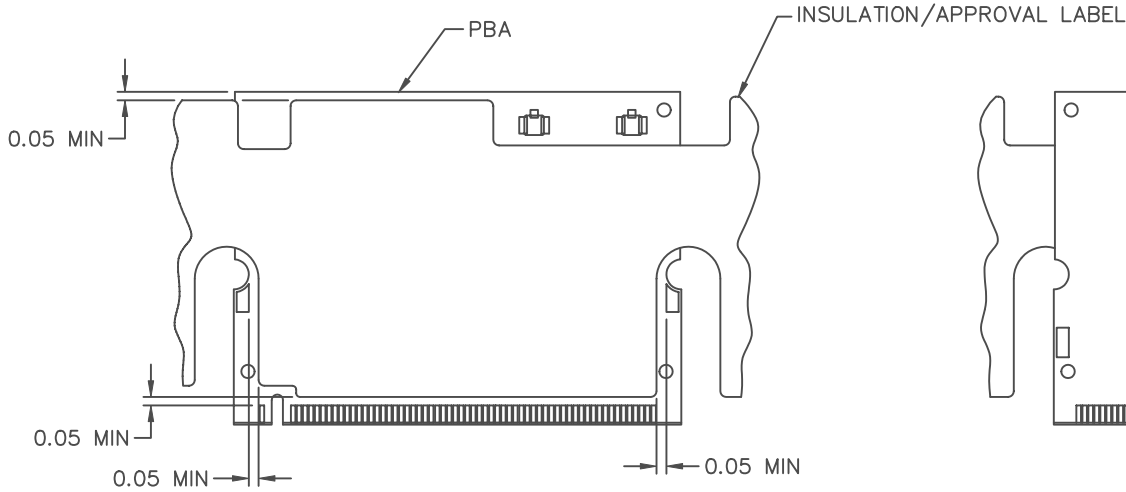
PRIMARY SIDE INSULATION PLACEMENT STEP 1
