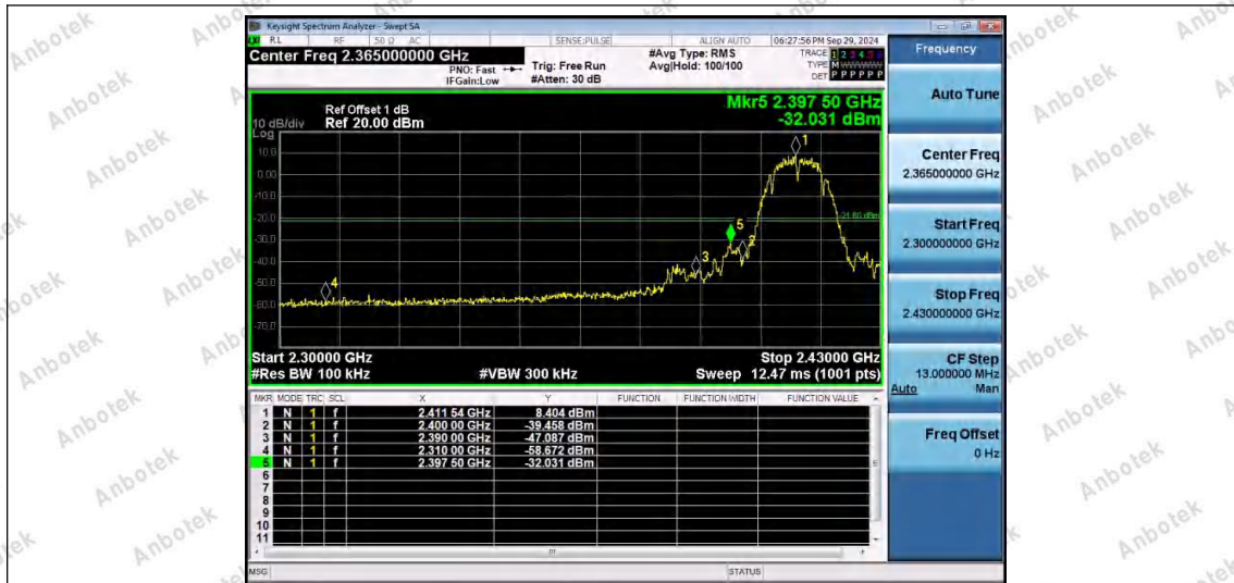
11B-Ant1-2412-PASS
