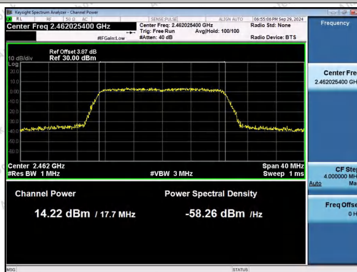
11N20SISO-Ant1-2462-PASS
