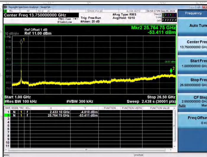
11N20SISO-Ant1-2437-1000~26500-PASS
