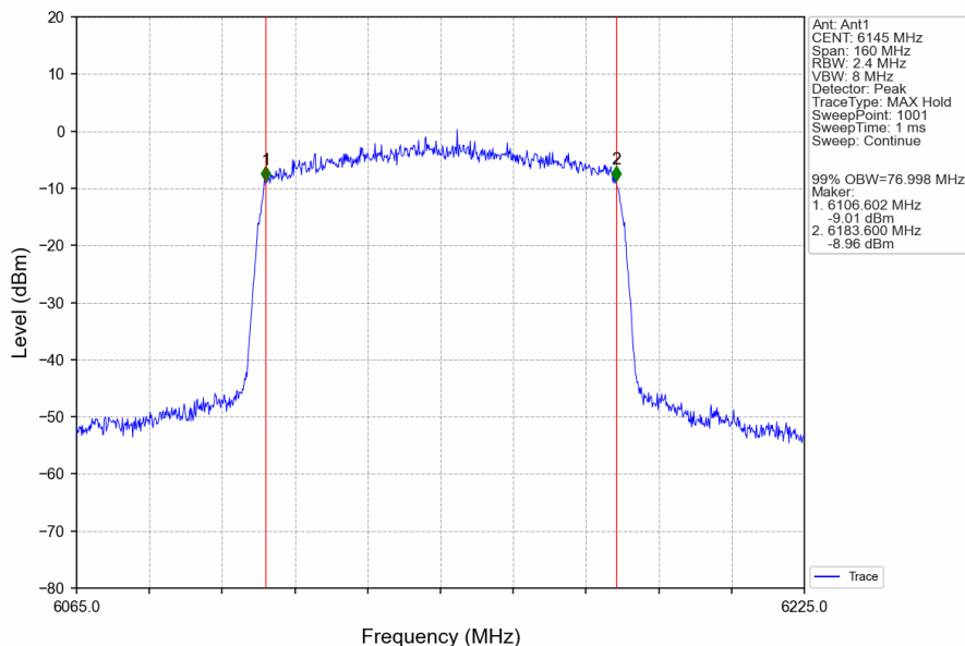
802.11ax(HEW80)_MCH_6145MHz_RU996_Left_Ant1_NTNV
