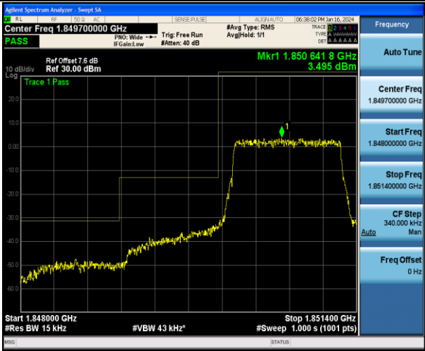
Band2_1.4MHz_QPSK_18607_6RB#0
