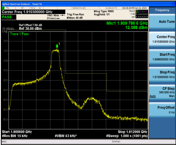
Band2_1.4MHz_QPSK_19193_1RB#5
