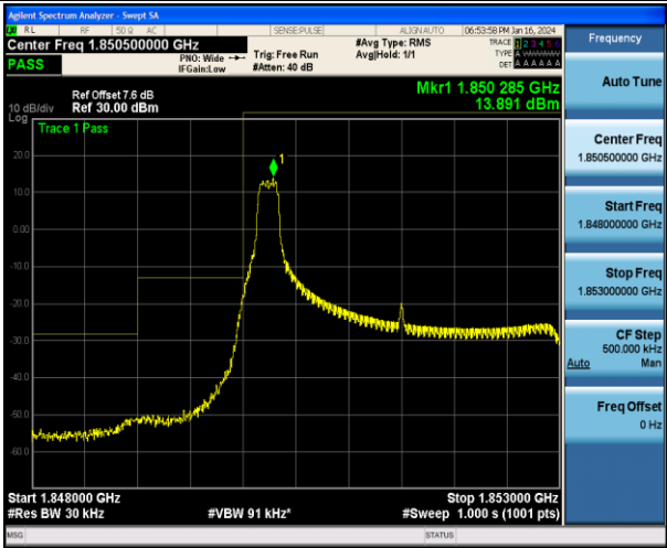
Band2_3MHz_16QAM_18615_1RB#0
