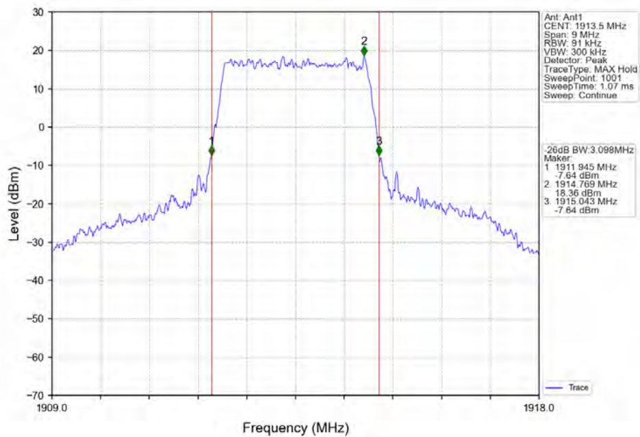
Band25_3MHz_64QAM_HCH_1913.5MHz_RB_15_0_NTN
