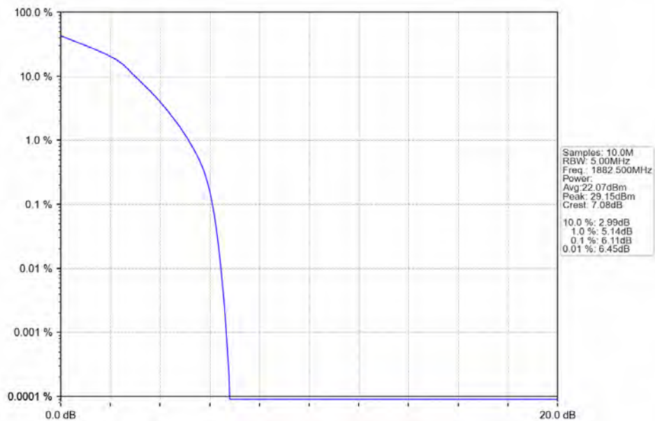
Band25_5MHz_64QAM_MCH_1882.5MHz_RB_25_0_NTV
