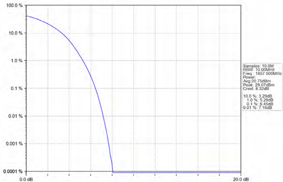
Band25_15MHz_16QAM_LCH_1857.5MHz_RB_75_0_NTV
