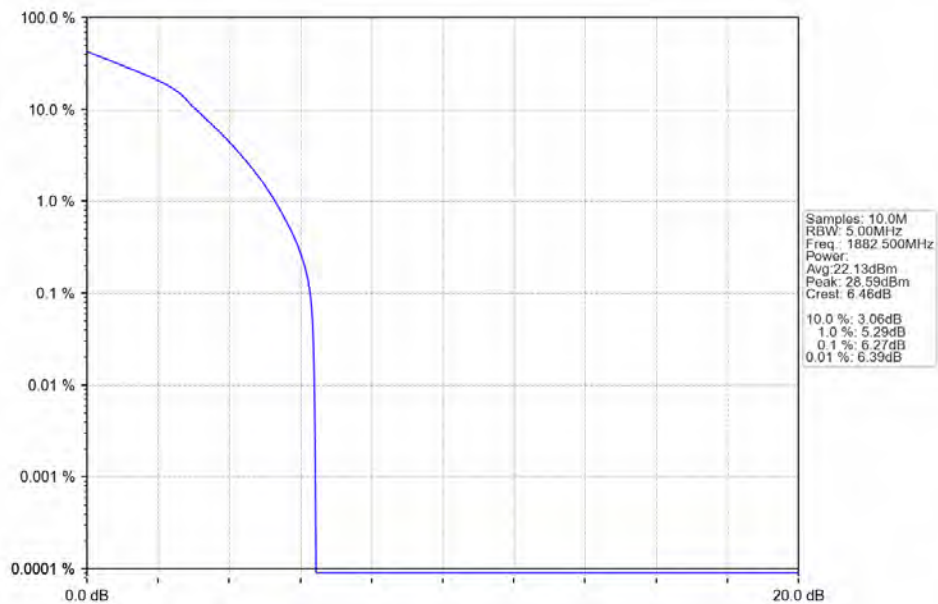
Band25_1.4MHz_64QAM_MCH_1882.5MHz_RB_6_0_NTN
