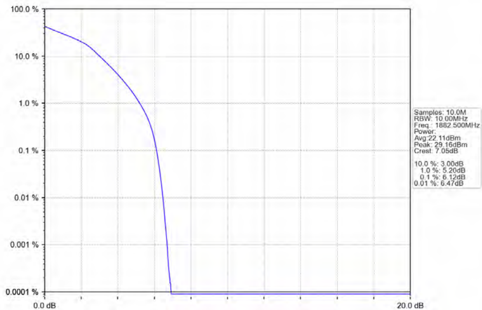
Band25_10MHz_64QAM_MCH_1882.5MHz_RB_50_0 NTN
