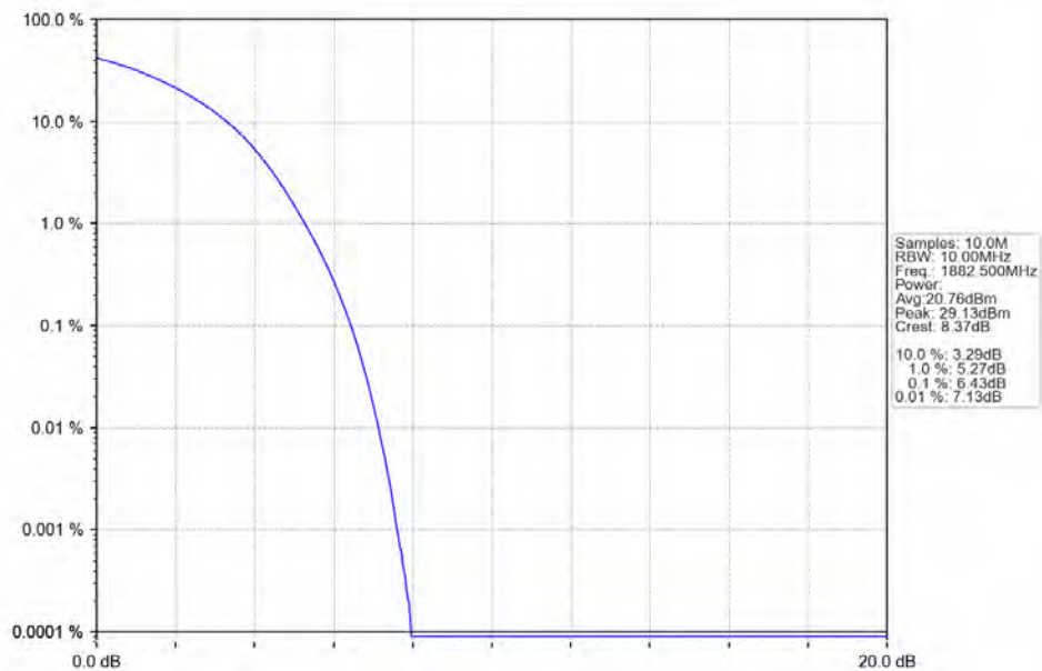
Band25_15MHz_64QAM_MCH_1882.5MHz_RB_75_0 NTN
