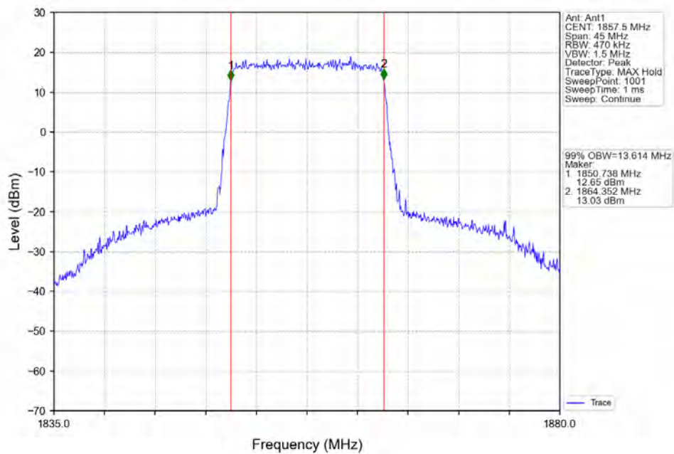
Band25_15MHz_16QAM_LCH_1857.5MHz_RB_75_0_NTV
