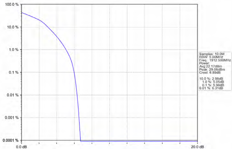
Band25_5MHz_16QAM_HCH_1912.5MHz_RB_25_0_NTN
