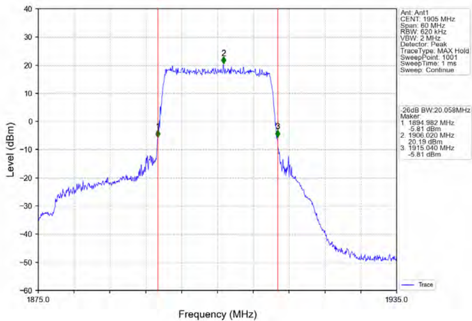
Band25_20MHz_QPSK_HCH_1905MHz_RB_100_0_NTN
