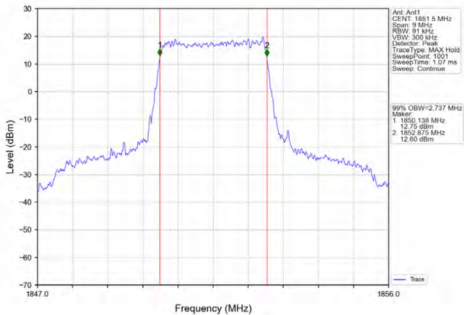
Band25_3MHz_QPSK_LCH_1851.5MHz_RB_15_0 NTN
