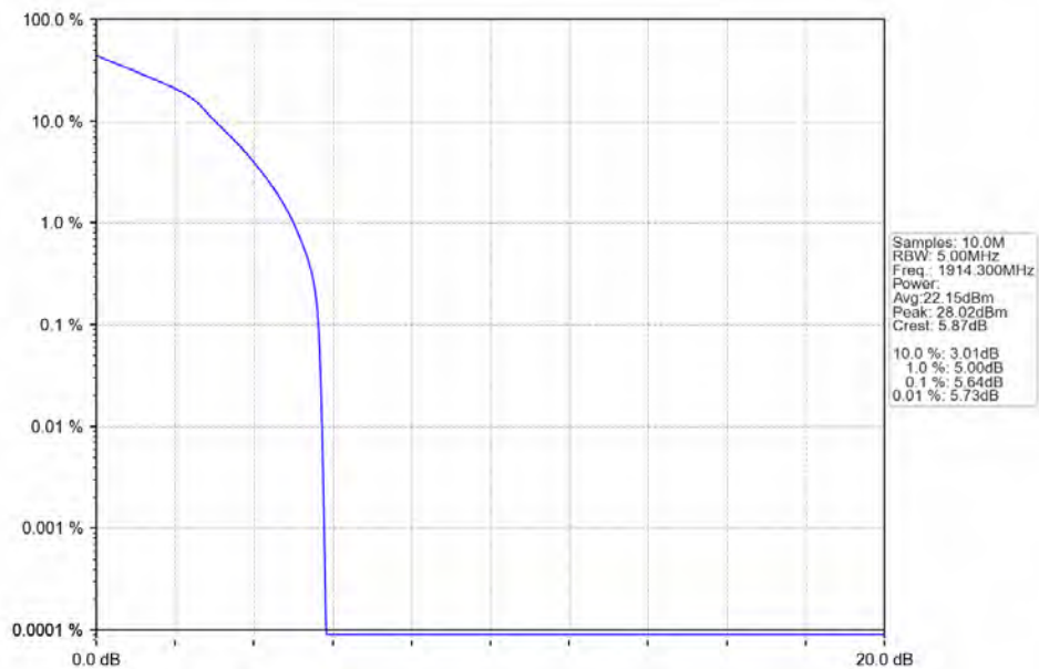
Band25_1.4MHz_16QAM_HCH_1914.3MHz_RB_6_0_NTN
