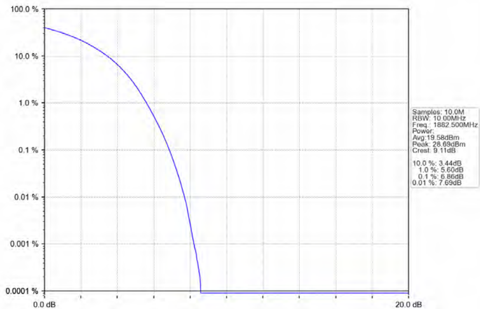
Band25_20MHz_64QAM_MCH_1882.5MHz_RB_100_0_NTN
