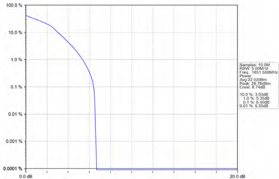
Band25_3MHz_16QAM_LCH_1851.5MHz_RB_15_0_NTV
