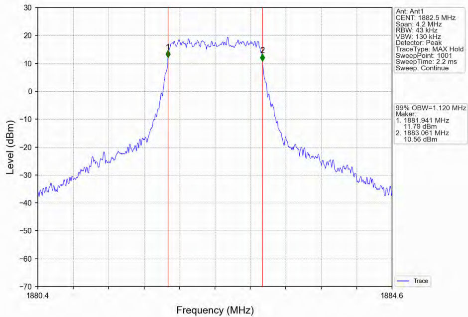
Band25_1.4MHz_64QAM_MCH_1882.5MHz_RB_6_0_NTN
