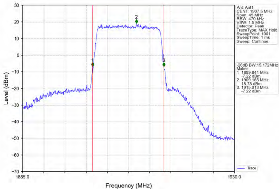
Band25_15MHz_16QAM_HCH_1907.5MHz_RB_75_0_NTN
