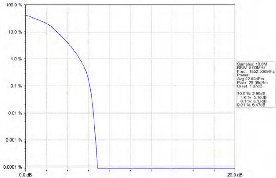
Band25 5MHz 64QAM LCH 1852.5MHz RB 25 0 NTV
