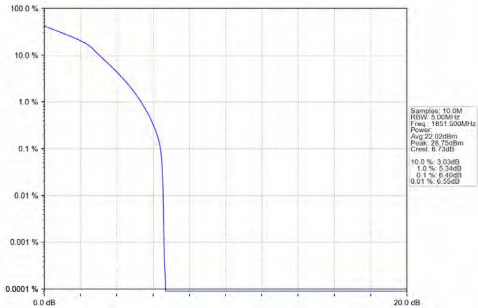
Band25 3MHz 64QAM LCH 1851.5MHz RB 15 0 NTV
