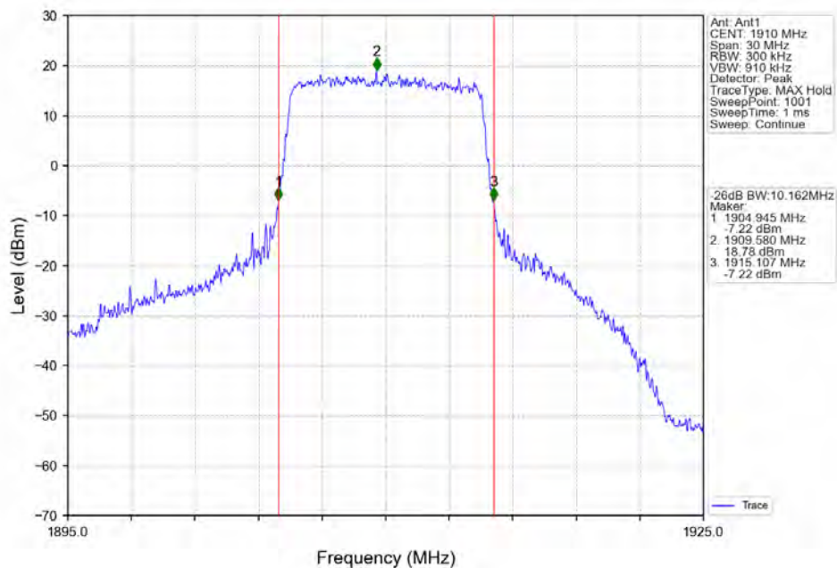
Band25_10MHz_64QAM_HCH_1910MHz_RB_50_0_NTN
