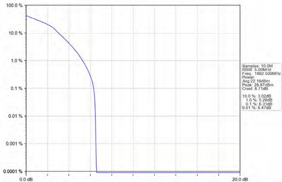
Band25_3MHz_64QAM_MCH_1882.5MHz_RB_15_0_NTV
