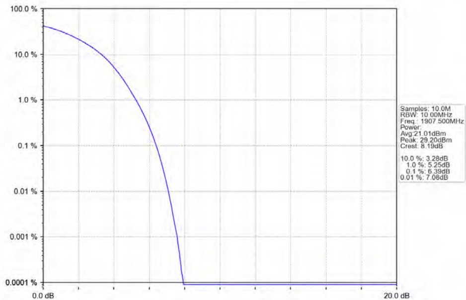
Band25_15MHz_16QAM_HCH_1907.5MHz_RB_75_0 NTN
