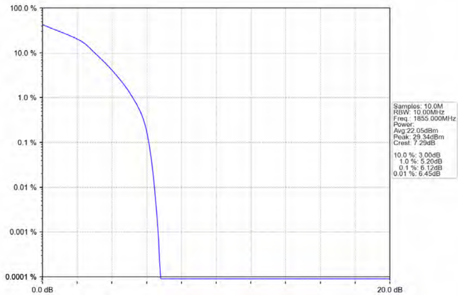
Band25 10MHz 64QAM LCH 1855MHz RB 50 0 NTN
