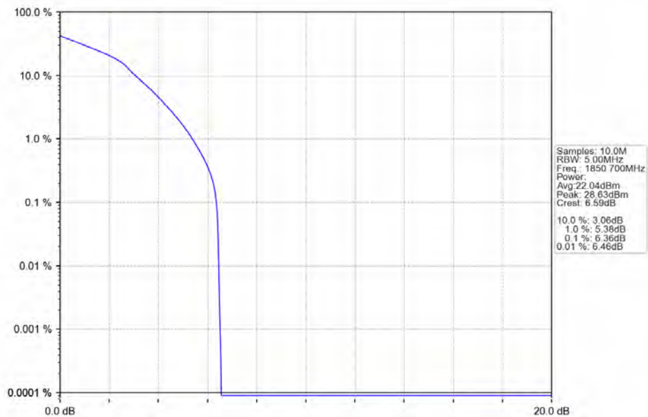
Band25_1.4MHz_16QAM_LCH_1850.7MHz_RB_6_0_NTN
