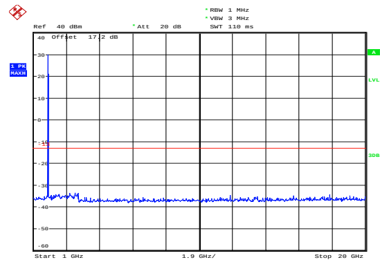
GSM 1900 CH-Low 1GHz ~ 20GHz
