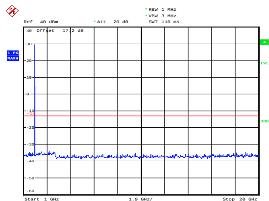
GSM 1900 CH-High 1GHz ~ 20GHz
