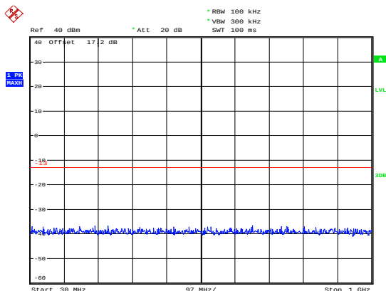
GSM 1900 CH-High 30MHz ~ 1GHz
