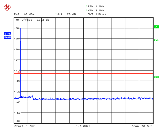
GSM 1900 CH- Middle 1GHz ~ 20GHz
