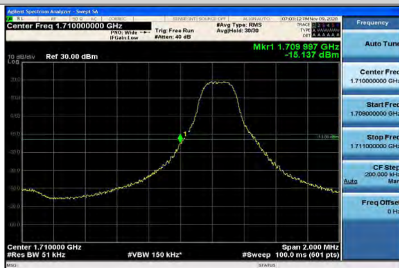
Band4-3MHz-16QAM-19965-1RB#14
