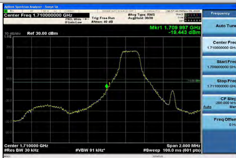
Band4-1.4MHz-16QAM-19957-1RB#5
