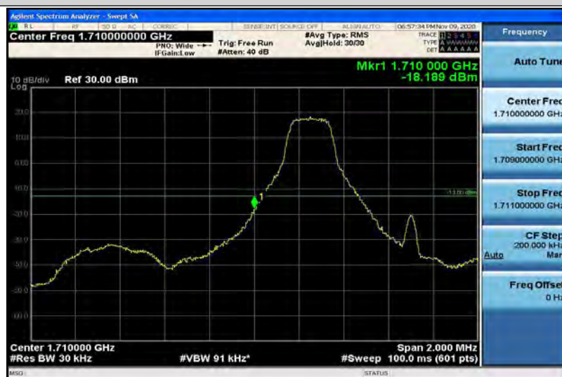
Band4-1.4MHz-QPSK-19957-1RB#5
