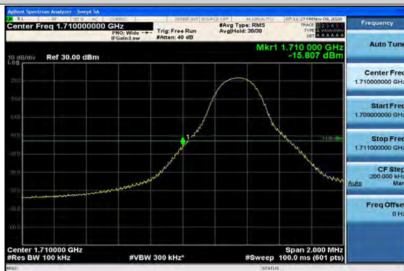
Band4-5MHz-16QAM-19975-1RB#24
