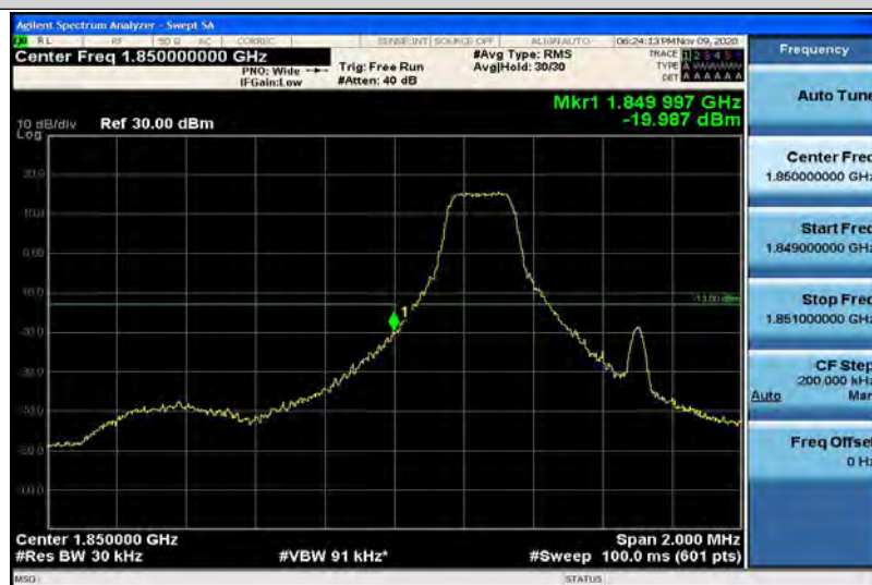
Band2-1.4MHz-16QAM-18607-1RB#5
