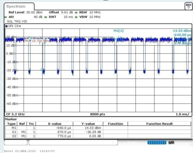
802.11n HT20_5200MHz
