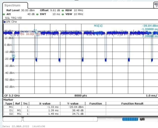
802.11a_5200 MHz
