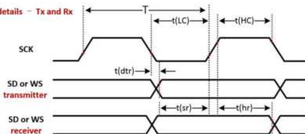
Figure 5.11- 1 I2S timing diagram
