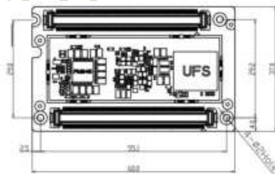
Figure 1.3-3 Bottom View
