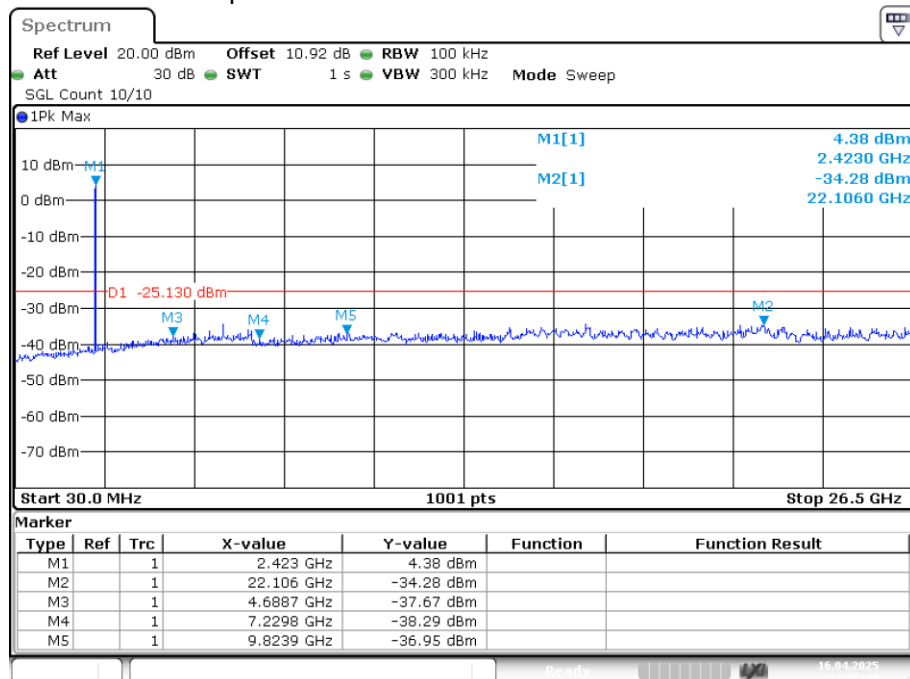
Tx. Spurious NVNT 2.4G 2410MHz Ant1 Emission
