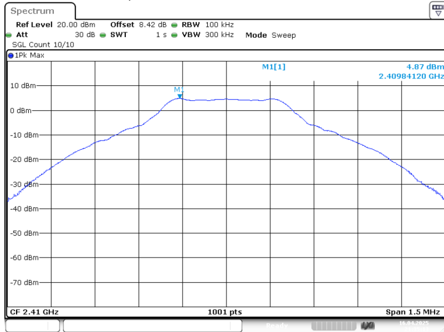
Tx. Spurious NVNT 2.4G 2410MHz Ant1 Ref
