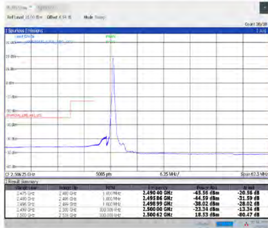
1-N7--15-25-L-4-CP-QPSK-Edge_1RB_Left-1@0-Ant1-PASS-see graph
