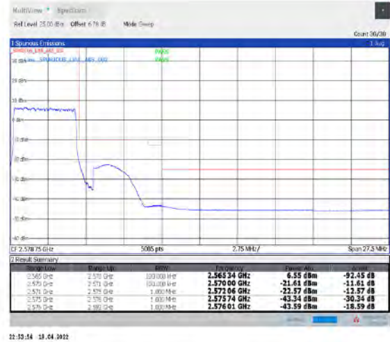
1-N7--15-5-H-3-DFT-PI2BPSK-Outer_Full-25@0-Ant1-PASS-see graph
