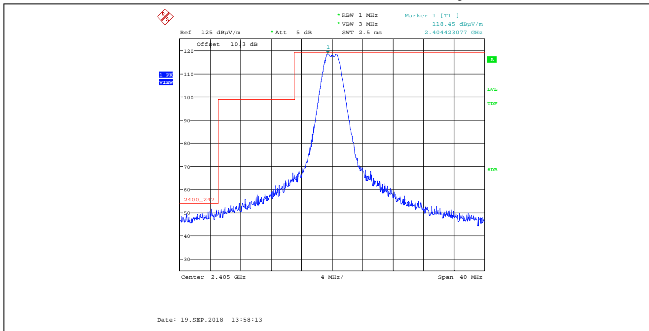
Plot 5.4.4.2.2. Band-Edge Radiated Emissions, Lower Band-edge Rx Antenna in Horizontal Polarization, O-QPSK Modulation, Power Setting 200, Ch 11, 2405 MHz
