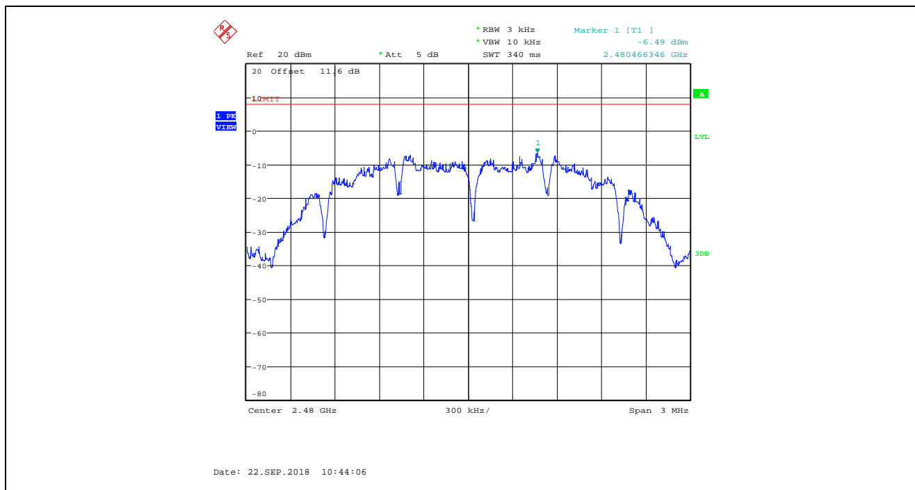
Plot 5.5.4.4. Power Spectral Density, O-QPSK Modulation, Power Setting 100, Channel 26, 2480 MHz
