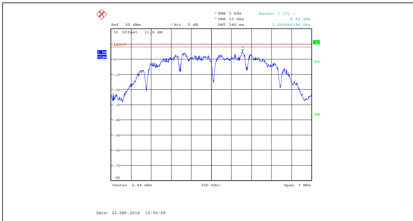
Plot 5.5.4.2. Power Spectral Density, O-QPSK Modulation, Power Setting 200, Channel 18, 2440 MHz
