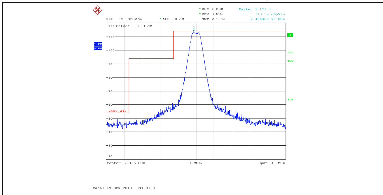
Plot 5.4.4.2.1. Band-Edge Radiated Emissions, Lower Band-edge Rx Antenna in Vertical Polarization, O-QPSK Modulation, Power Setting 200, Ch 11, 2405 MHz
