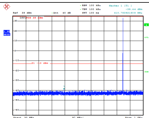
Channel 251: 30MHz~1GHz
