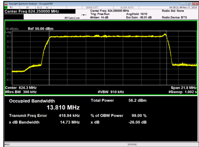
LTE15 Bottom Channel
