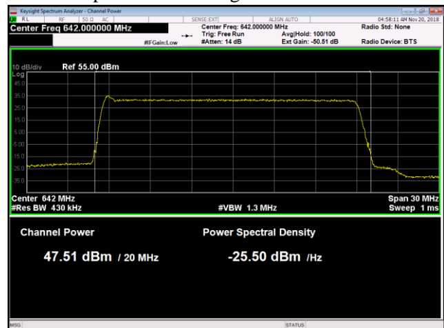
LTE20 Top Channel Average Power
