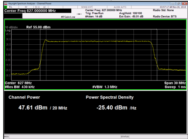
LTE20 Bottom Channel Average Power
