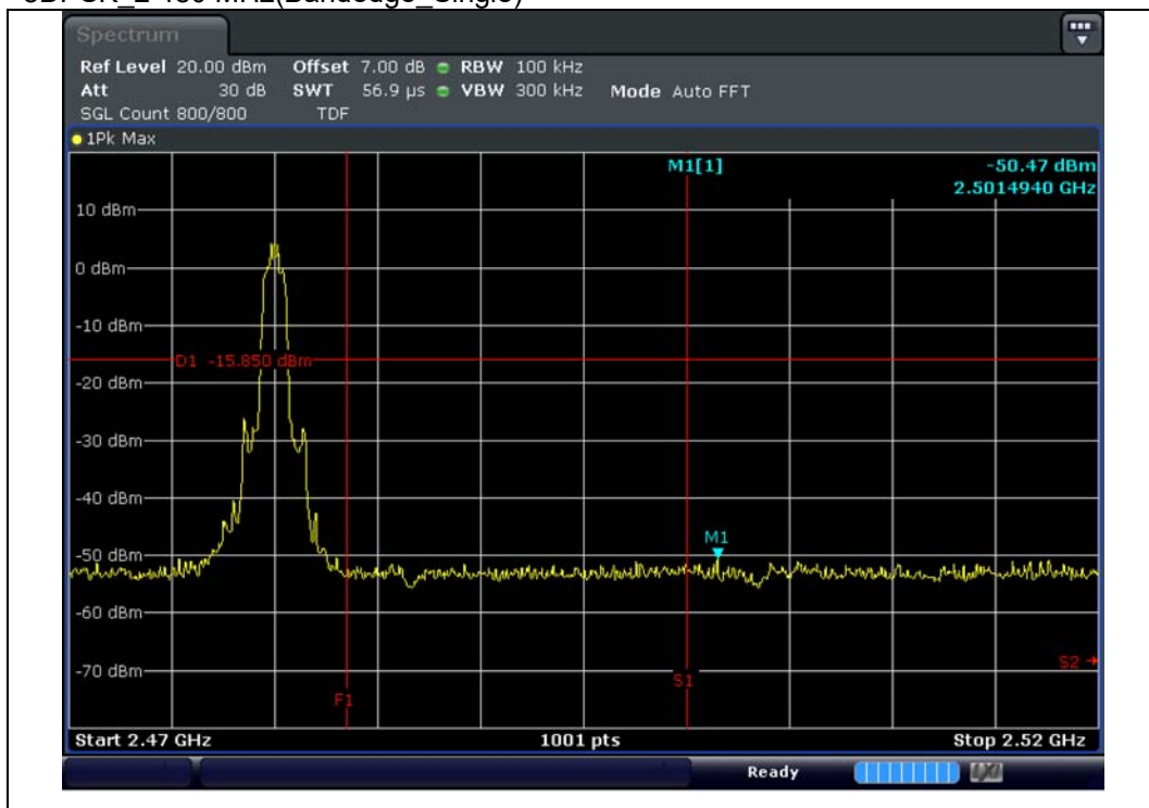
8DPSK_2 480 MHz(Bandedge_Single)
