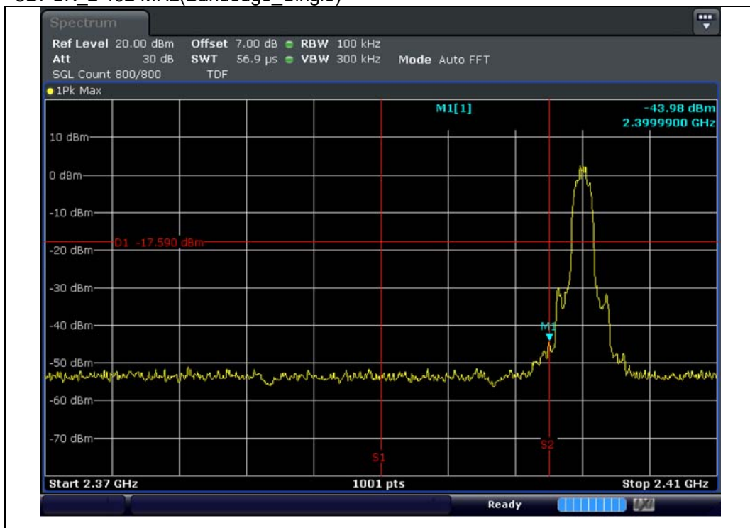
8DPSK_2_402 MHz(Bandedge_Single)
