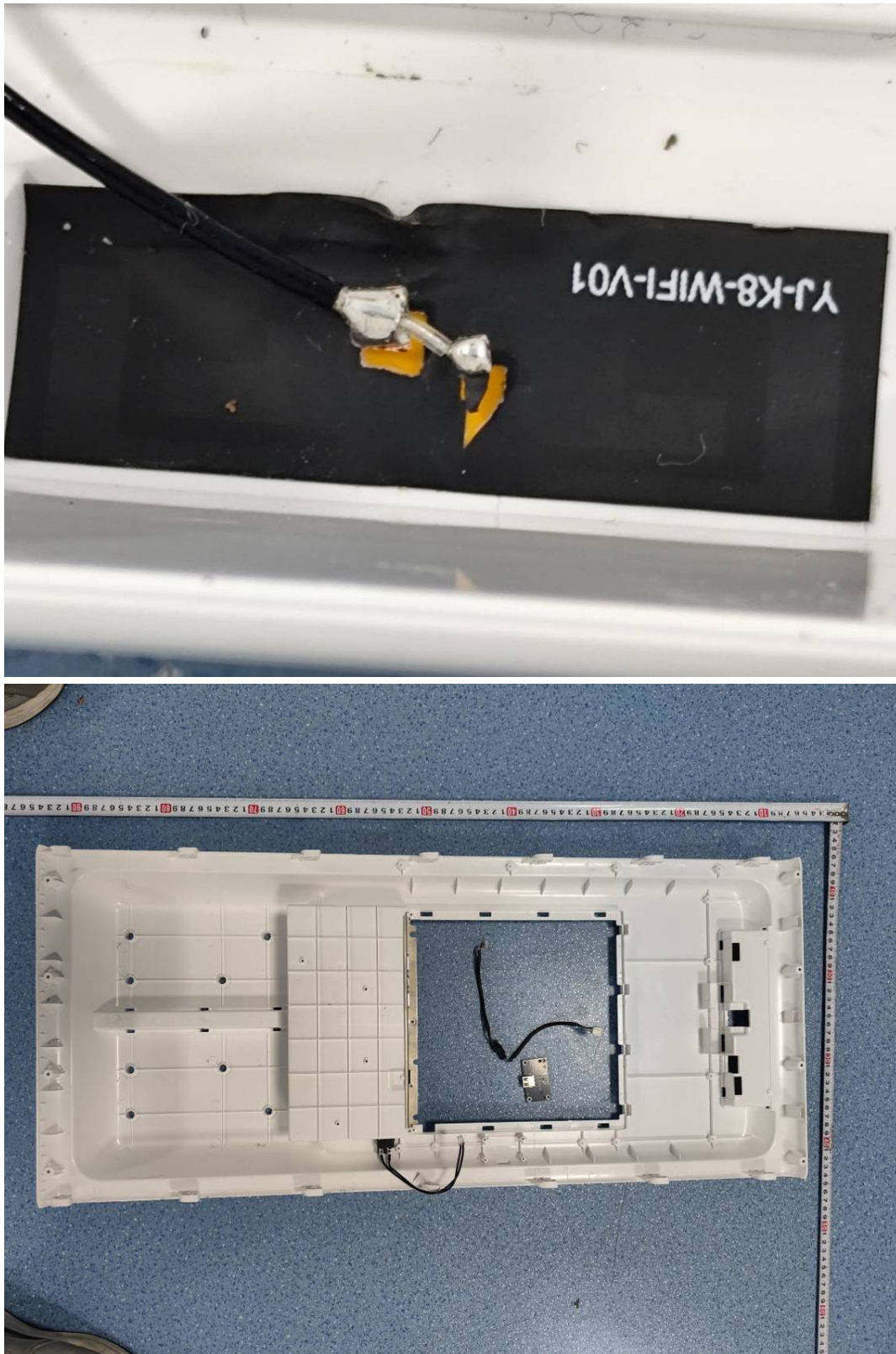
WIFI/Bluetooth antenna
