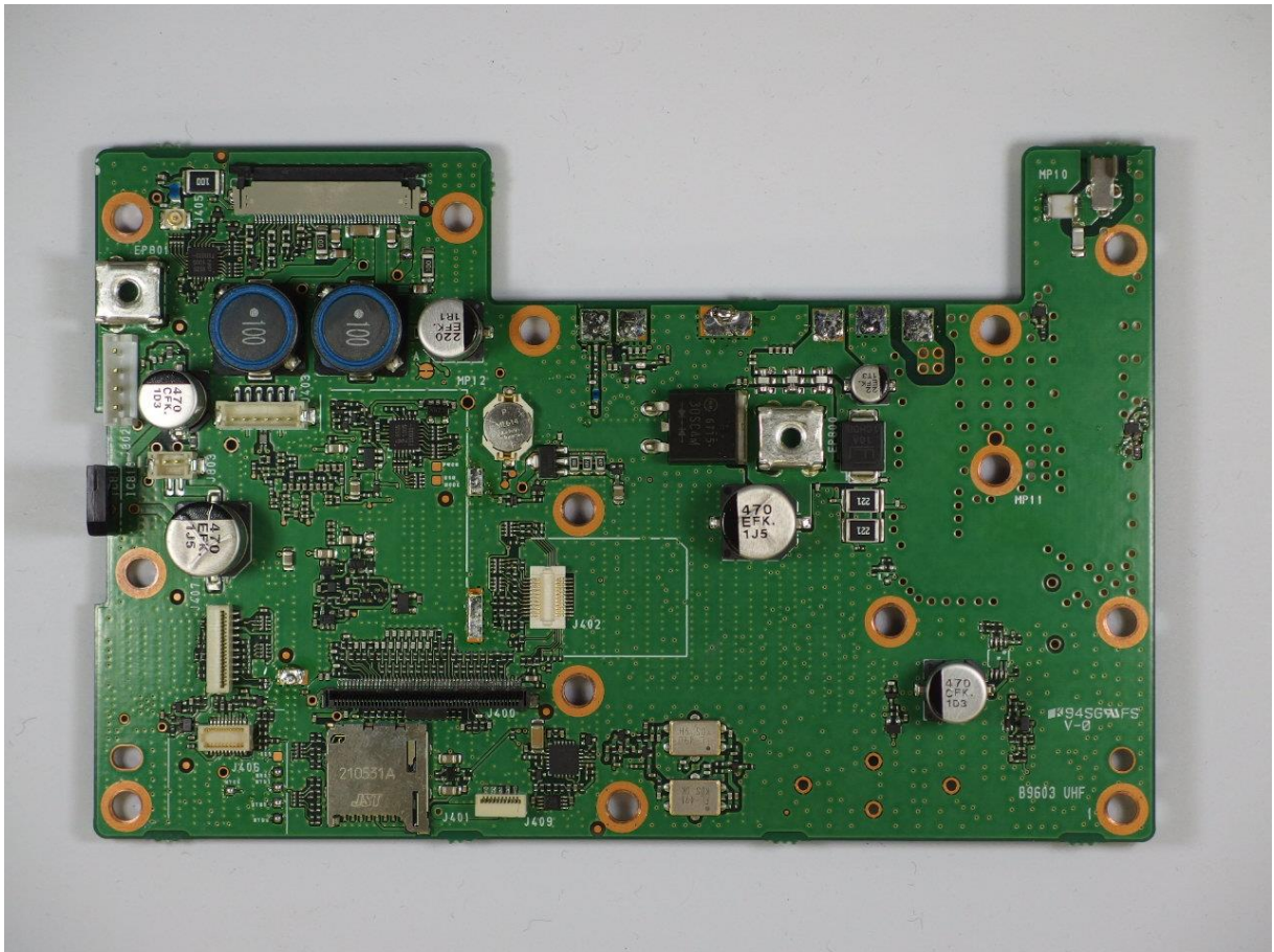
IC-F6400D/DS MAIN-C BOARD SIDE-A
