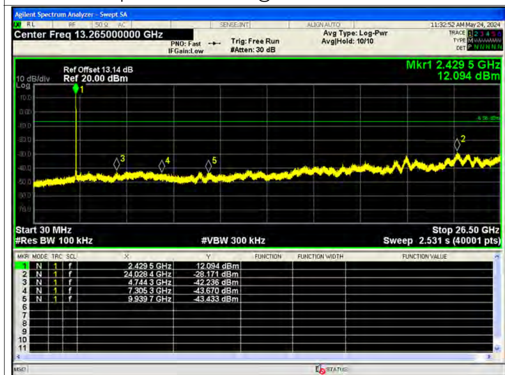
Tx. Spurious NVNT ax20 26@0 2437MHz Ant2 Emission
