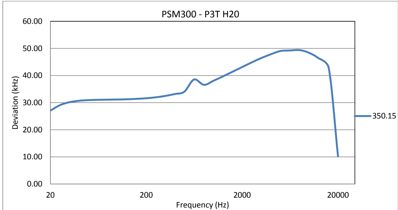
Deviation vs Frequency
