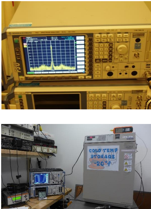
Figure B-1 - Test Setup for Frequency Stability
