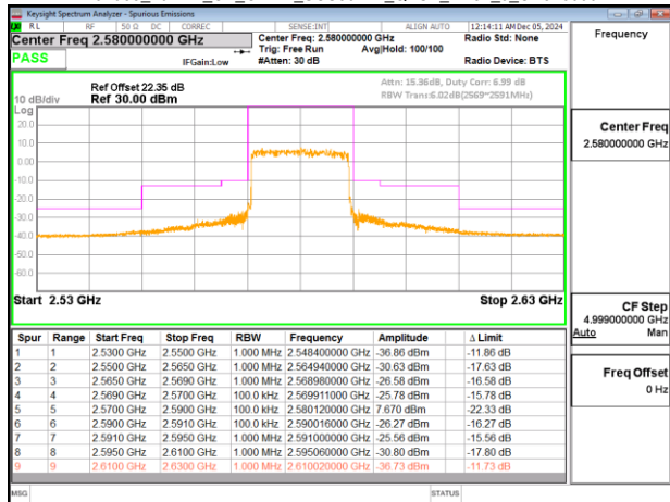
Band38_20MHz_CP_OFDM_SCS30kHz_QPSK_RB51_0_CH516000
