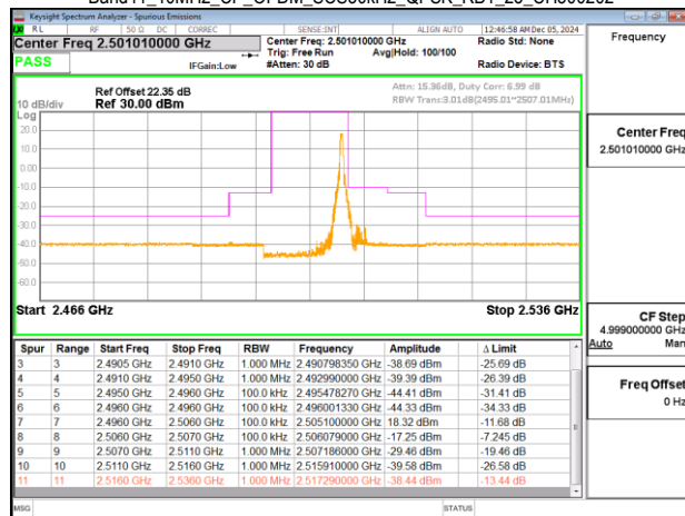
Band41_10MHz_CP_OFDM_SCS30kHz_QPSK_RB24_0_CH500202
