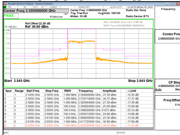
Band38_20MHz_CP_OFDM_SCS30kHz_QPSK_RB51_0_CH519000
