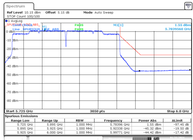
BE-NR-HIGH, MIMO-B, 802.11ax160-MCS0, Ch163
