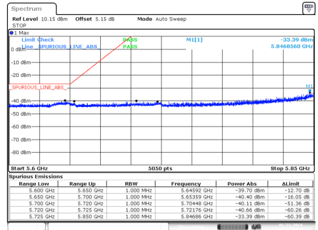
BE-NR-LOW, SISO-B, 802.11ax20-MCS0, Ch177
