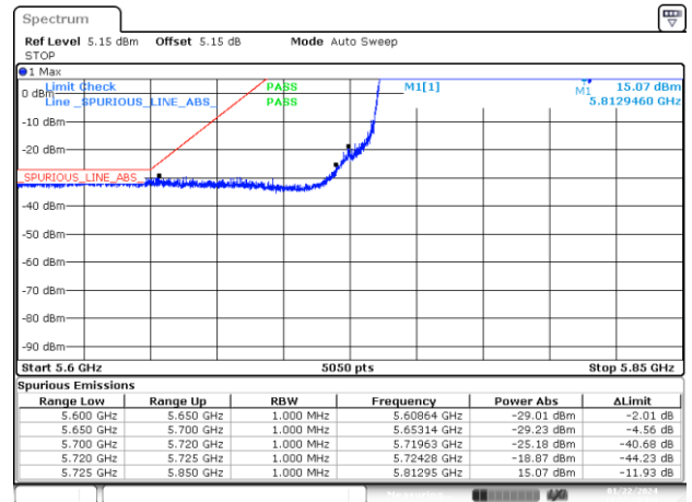
BE-NR-LOW, SISO-B, 802.11ax160-MCS0, Ch163
