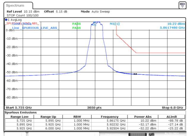
BE-NR-HIGH, MIMO-B, 802.11n20-HT0, Ch173
