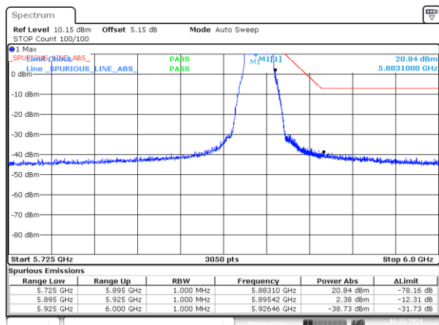
BE-NR-HIGH-PEAK, MIMO-B, 802.11n20-HT0, Ch177
