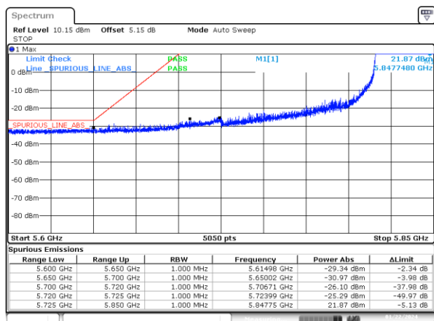
BE-NR-LOW, SISO-B, 802.11ax80-MCS0, Ch171
