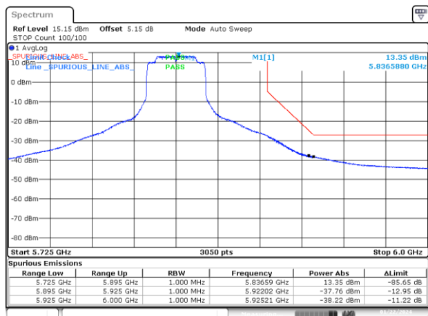
BE-NR-HIGH, SISO-B, 802.11ax40-MCS0, Ch167
