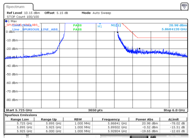
BE-NR-HIGH-PEAK, MIMO-B, 802.11ax80-MCS0, Ch171
