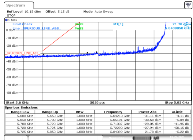
BE-NR-LOW, MIMO-B, 802.11ax80-MCS0, Ch171
