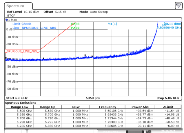
BE-NR-LOW, MIMO-A, 802.11n40-HT0, Ch167
