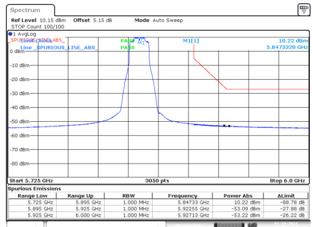
BE-NR-HIGH, MIMO-A, 802.11n20-HT0, Ch169
