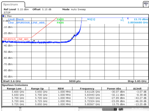
BE-NR-LOW, MIMO-A, 802.11ax160-MCS0, Ch163
