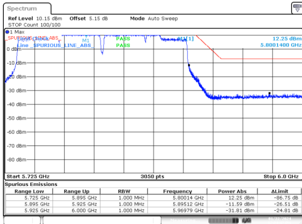
BE-NR-HIGH-PEAK, MIMO-B, 802.11ac160-VHT0, Ch163
