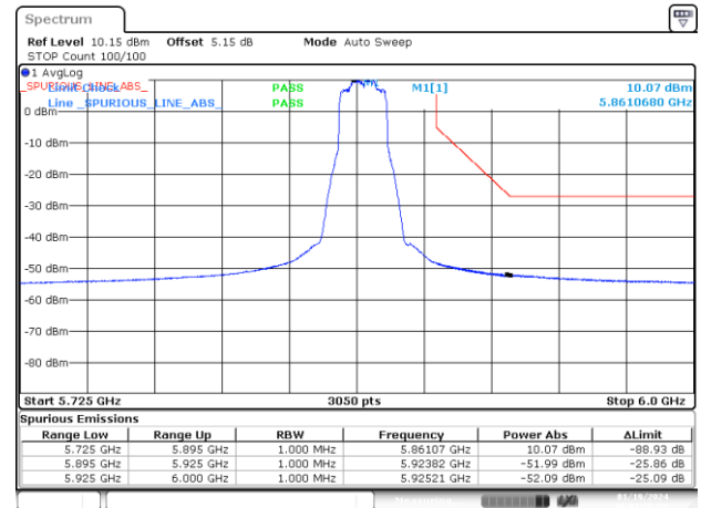
BE-NR-HIGH, MIMO-A, 802.11ax20-MCS0, Ch173
