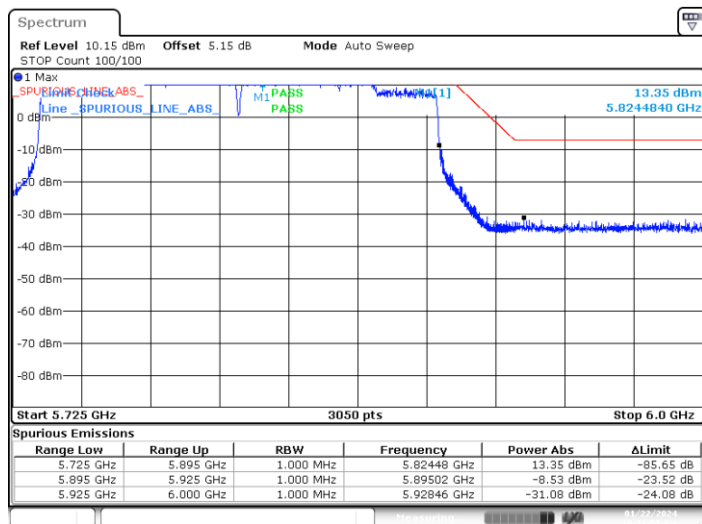
BE-NR-HIGH-PEAK, MIMO-A, 802.11ax160-MCS0, Ch163
