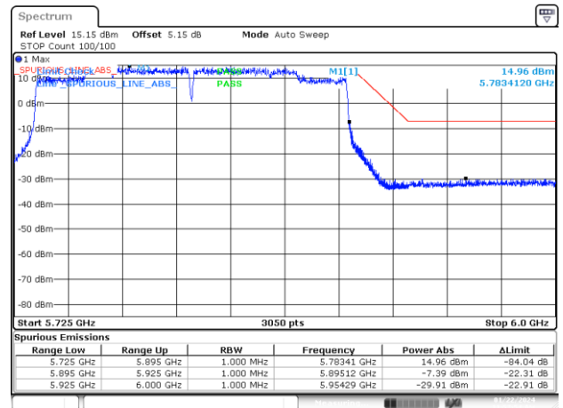
BE-NR-HIGH-PEAK, SISO-B, 802.11ax160-MCS0, Ch163
