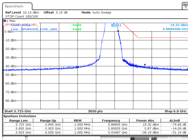
BE-NR-HIGH-PEAK, MIMO-A, 802.11n20-HT0, Ch177
