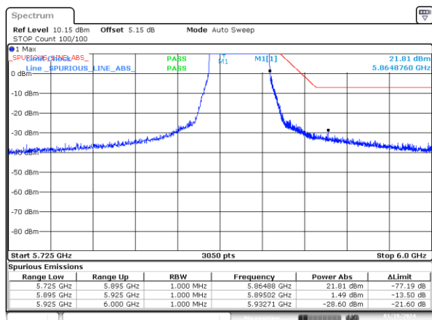
BE-NR-HIGH-PEAK, MIMO-A, 802.11ax40-MCS0, Ch175
