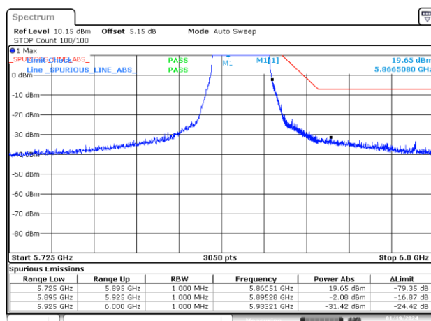
BE-NR-HIGH-PEAK, MIMO-A, 802.11n40-HT0, Ch175
