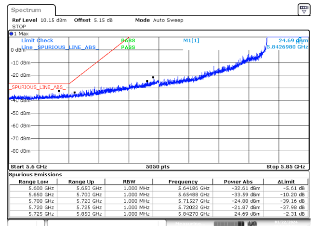
BE-NR-LOW, SISO-B, 802.11ax40-MCS0, Ch167
