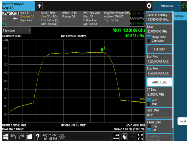
Plot 7-541. Peak Power Spectral Density Plot (B2_10M_1C_16QAM - Low Channel, Port 0)
