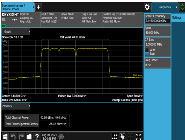
Plot 7-521. Conducted Average Output Power Plot (B66_5M+5M+10M+20M_4C_QPSK - Mid Channel, Port 0)
