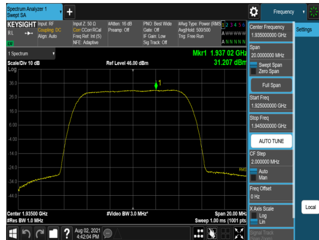
Plot 7-544. Peak Power Spectral Density Plot (B2_10M_1C_16QAM - Low Channel, Port 3)
