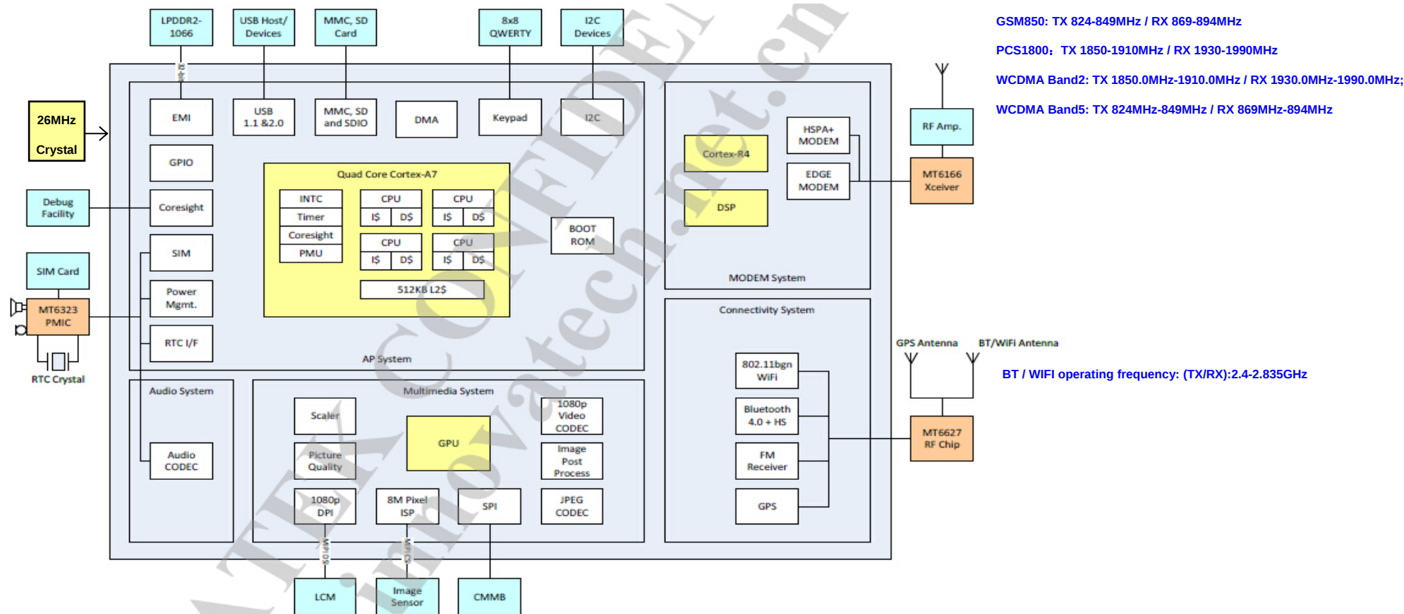
Figure 1-1: Block diagram of MT8382
