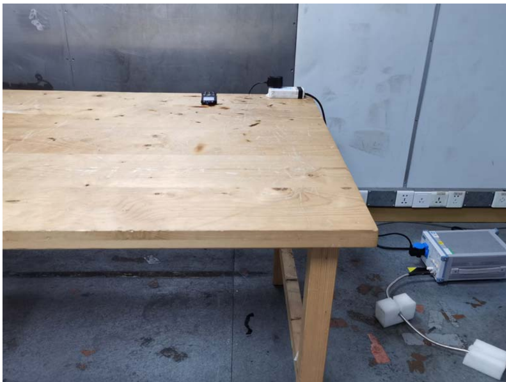
Photo of Power Line Conducted Emission Measurement
