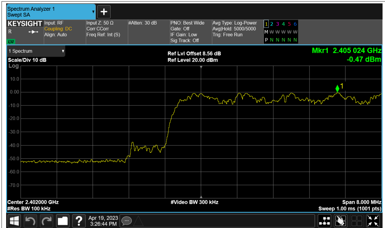
Band Edge(Hopping) NVNT 3-DH1 2402MHz Ant9 Hopping Emission
