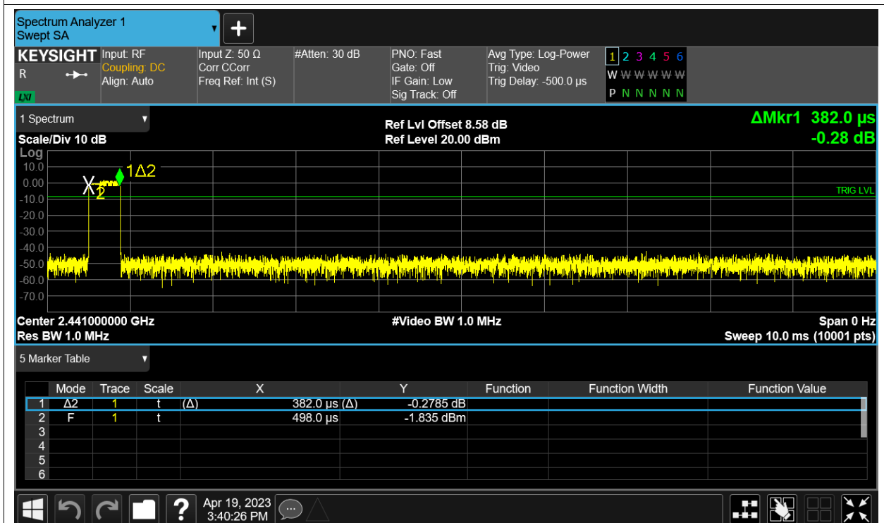
Dwell NVNT 2-DH3 2441MHz Ant9
