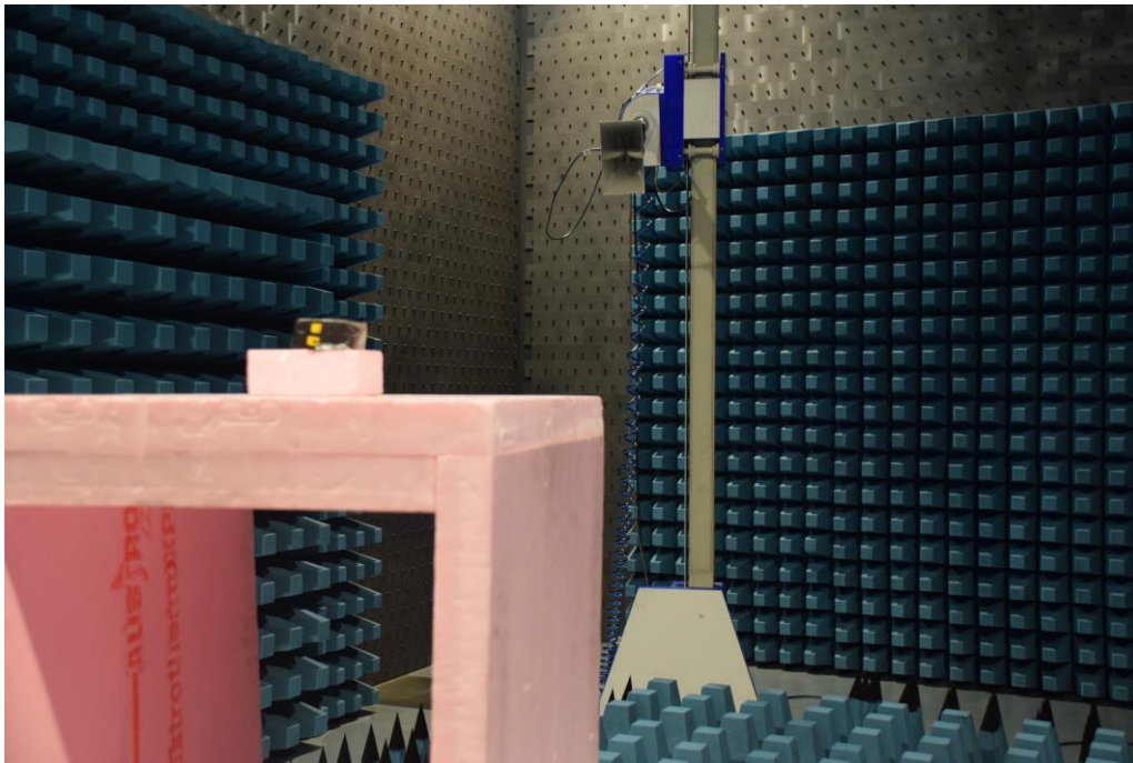
Picture 9: SAC, radiated emission 1 GHz – 4 GHz of FS14T, version FS14T (front view)
