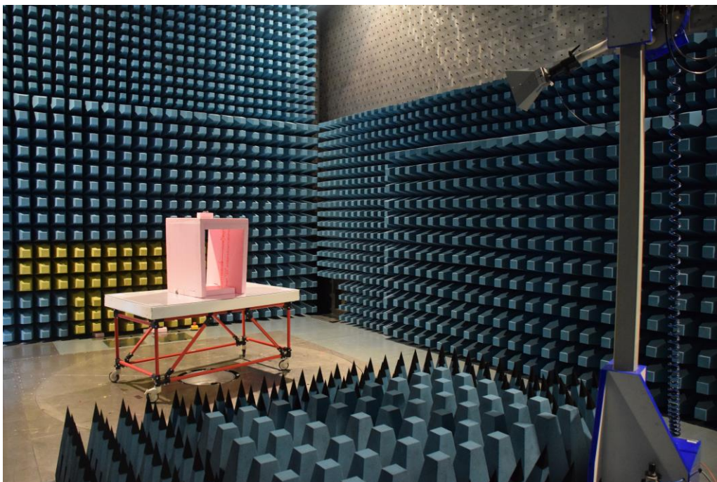
Picture 12: SAC, radiated emission 1 GHz – 4 GHz of FS14T, version FS14TK (rear view)
