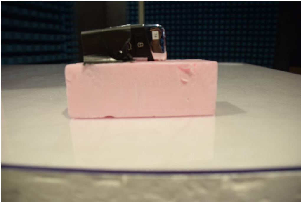
Picture 15: EUT-position Z
