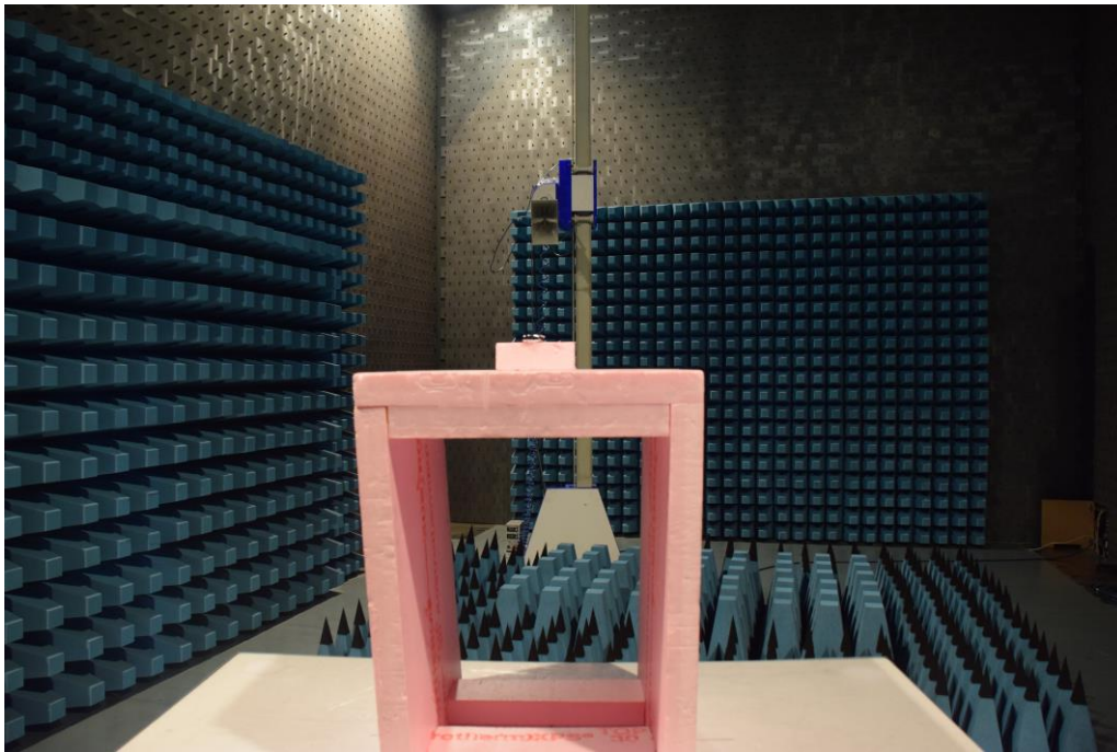
Picture 11: SAC, radiated emission 1 GHz – 4 GHz of FS14T, version FS14TK (front view)
