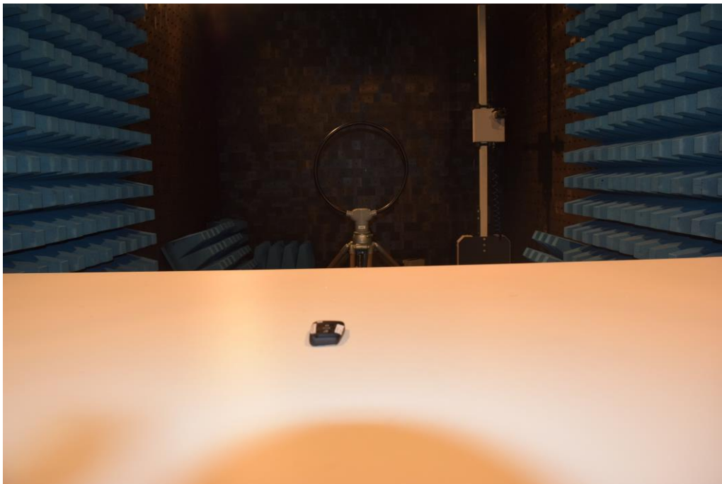
Picture 4: CDC, test setup radiated emission test 9 kHz -30 MHz of FS14T, version FS14TK (front view)
