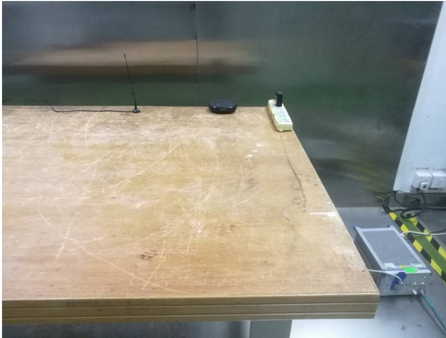
Conducted Emissions - Front View(Adapter: BLJ05K050100P-UA)
