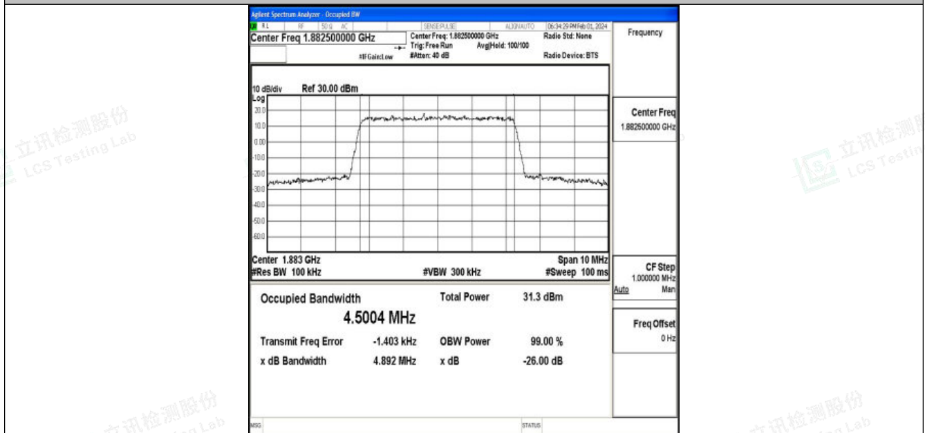
Band25-5MHz-16QAM-26365-25RB#0-PASS
