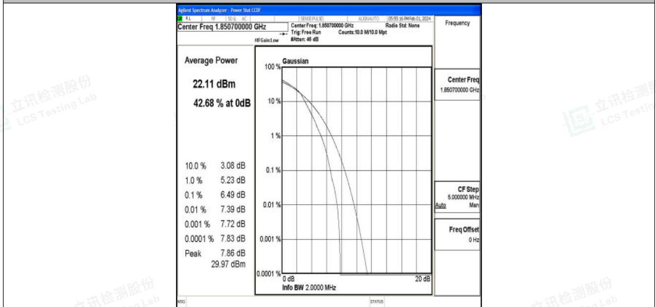
Band25-1.4MHz-16QAM-26047-6RB#0-PASS
