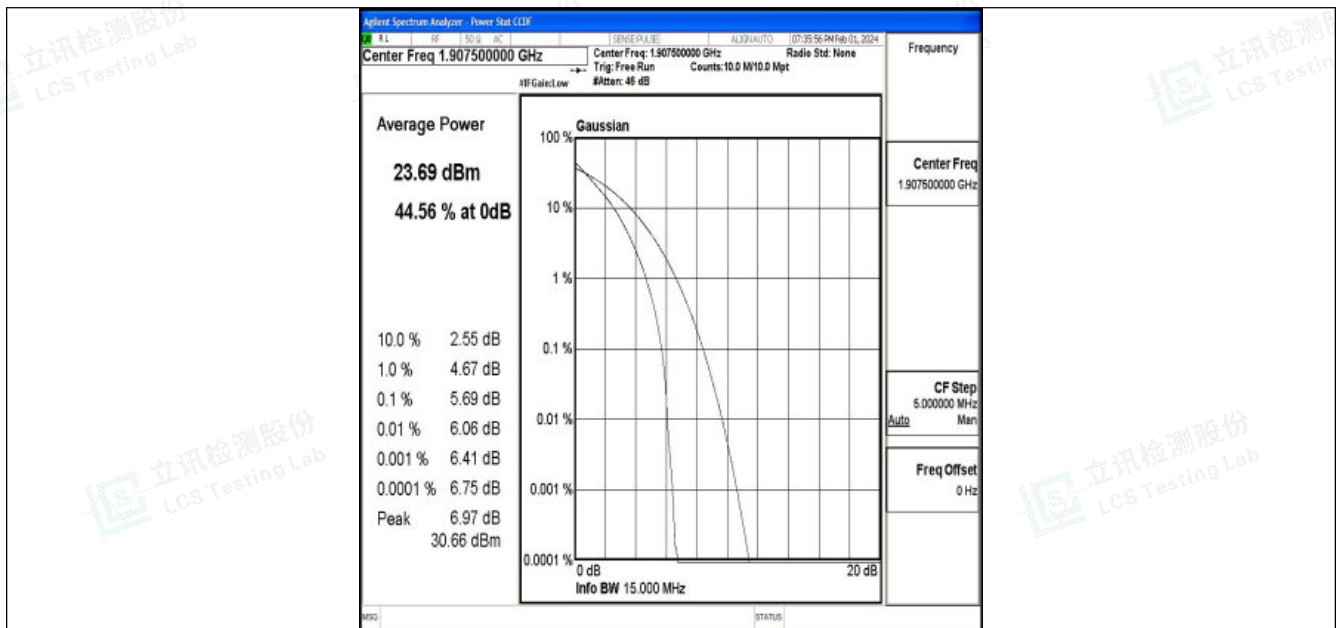
Band25-15MHz-QPSK-26615-75RB#0-PASS
