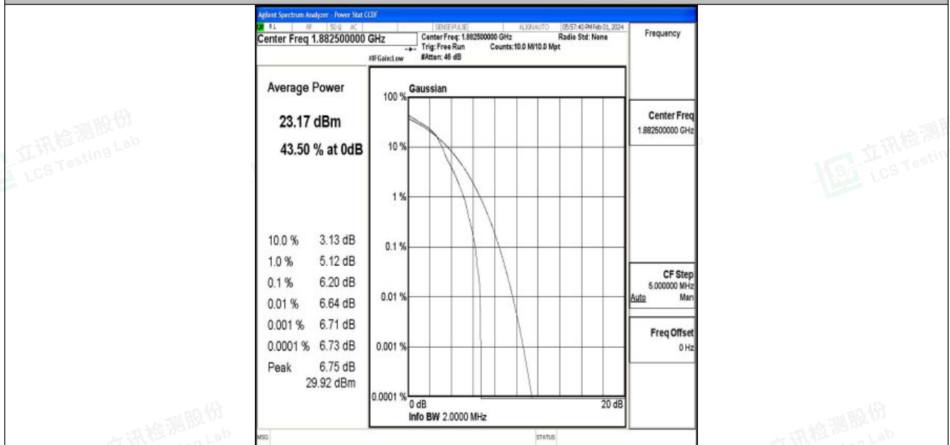
Band25-1.4MHz-16QAM-26365-1RB#0-PASS
