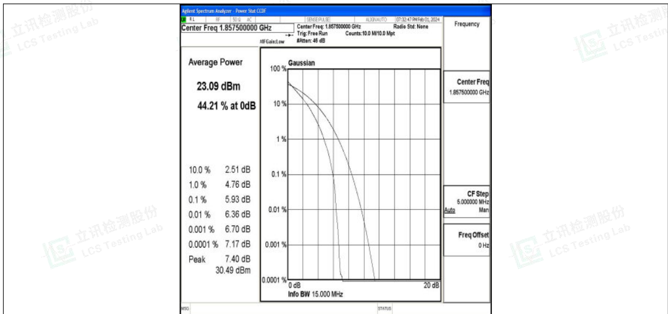
Band25-15MHz-QPSK-26115-75RB#0-PASS
