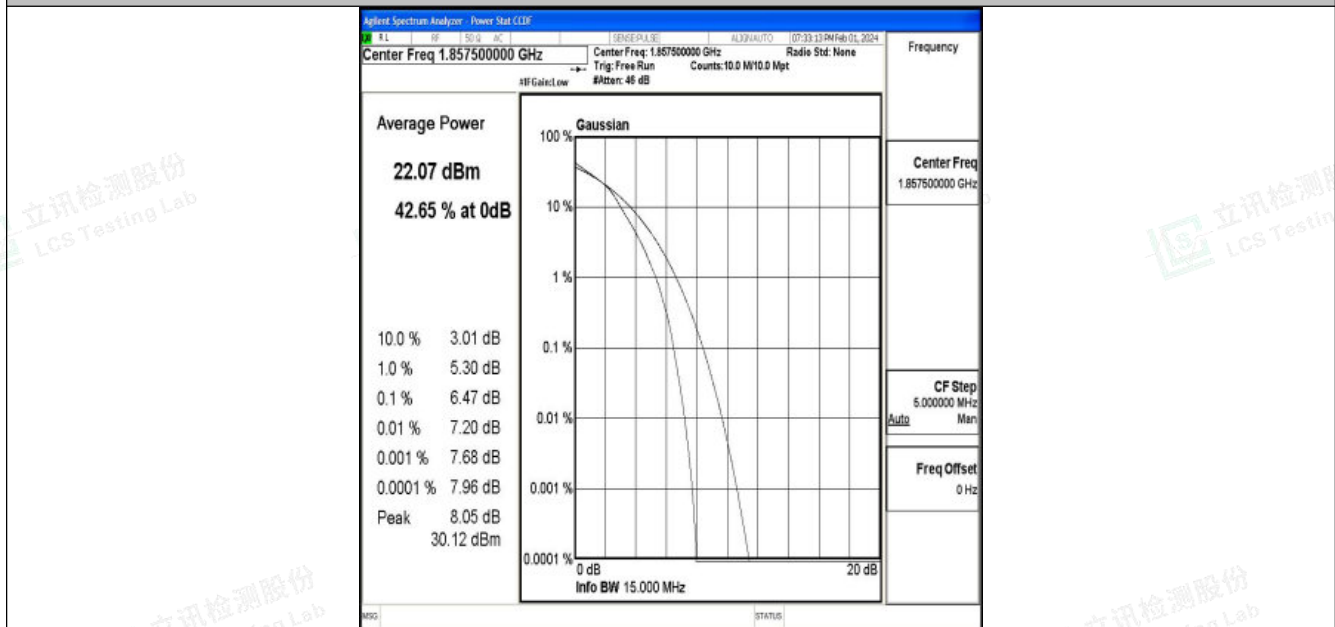
Band25-15MHz-16QAM-26115-75RB#0-PASS
