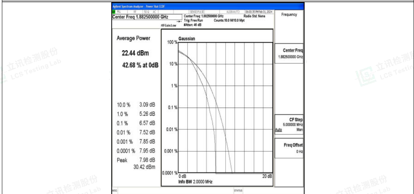
Band25-1.4MHz-16QAM-26365-6RB#0-PASS
