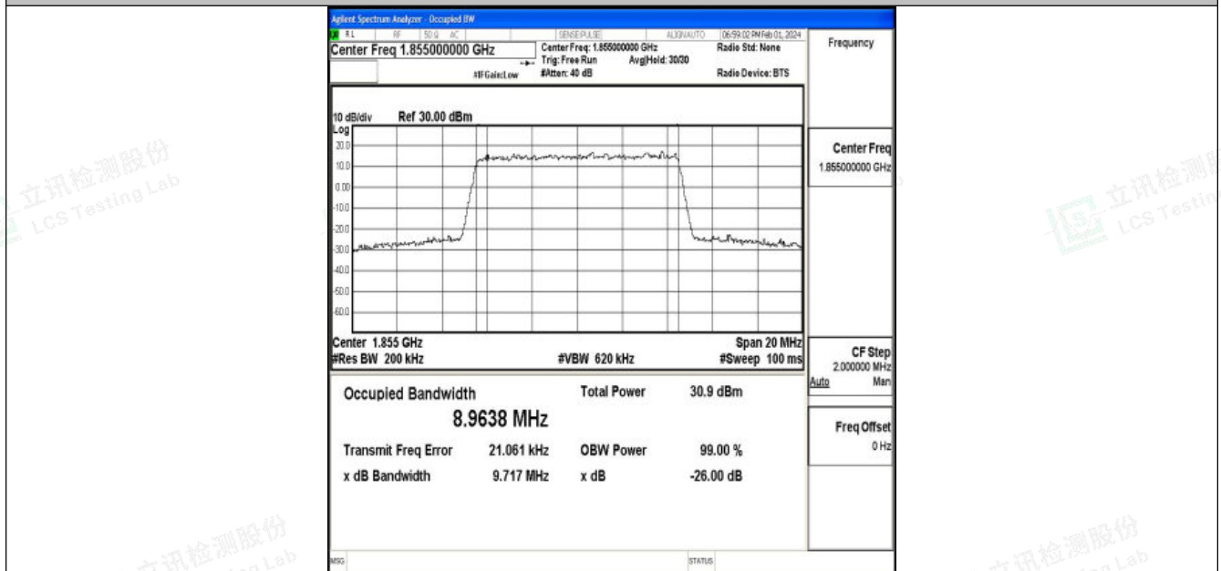
Band25-10MHz-16QAM-26090-50RB#0-PASS
