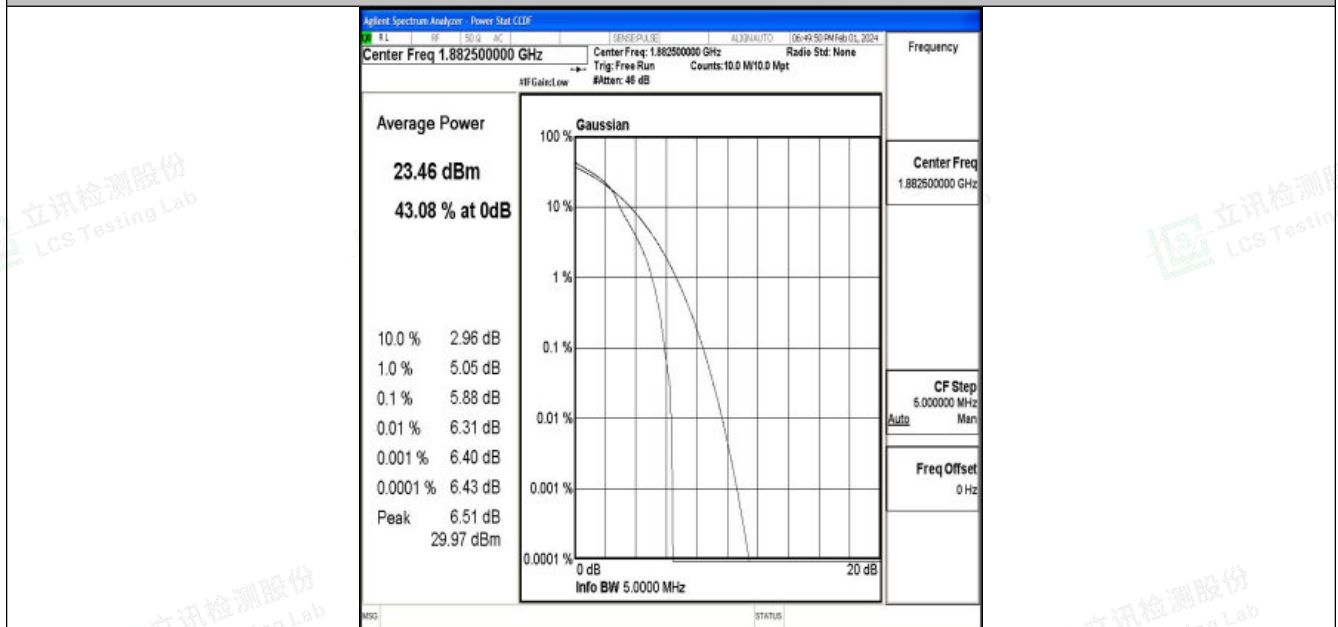
Band25-5MHz-16QAM-26365-1RB#0-PASS
