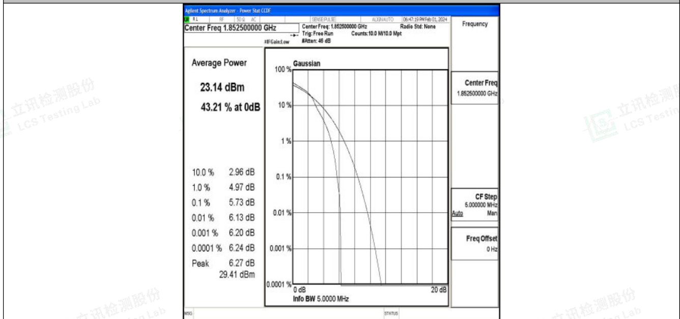
Band25-5MHz-16QAM-26065-1RB#0-PASS
