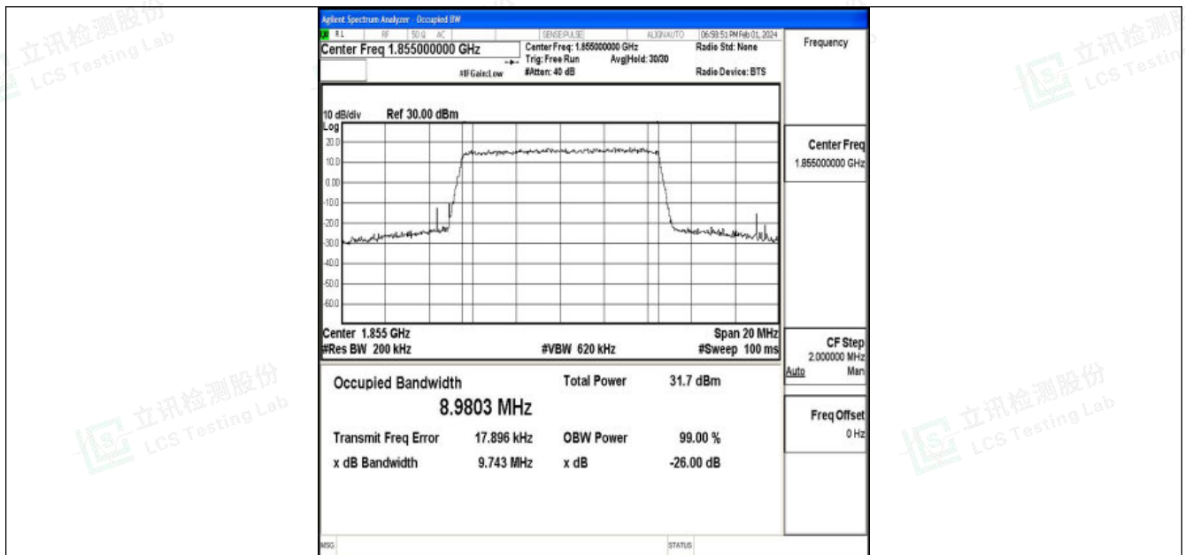
Band25-10MHz-QPSK-26090-50RB#0-PASS
