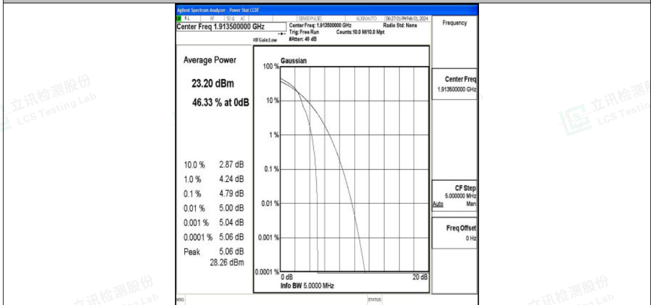
Band25-3MHz-16QAM-26675-1RB#0-PASS
