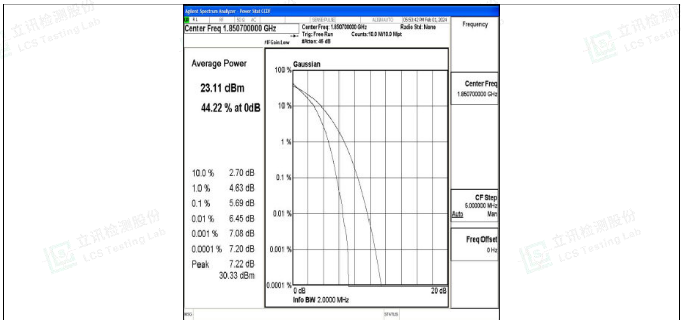
Band25-1.4MHz-QPSK-26047-6RB#0-PASS
