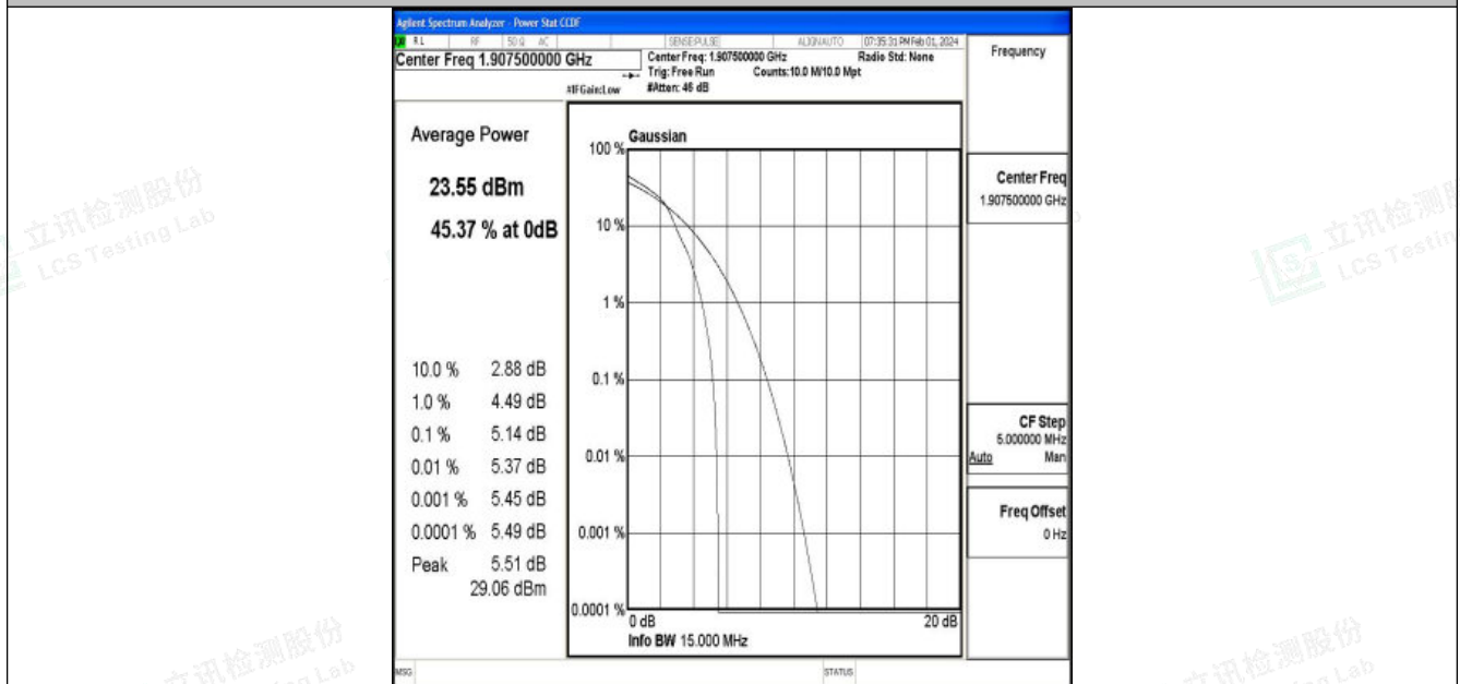
Band25-15MHz-16QAM-26615-1RB#0-PASS
