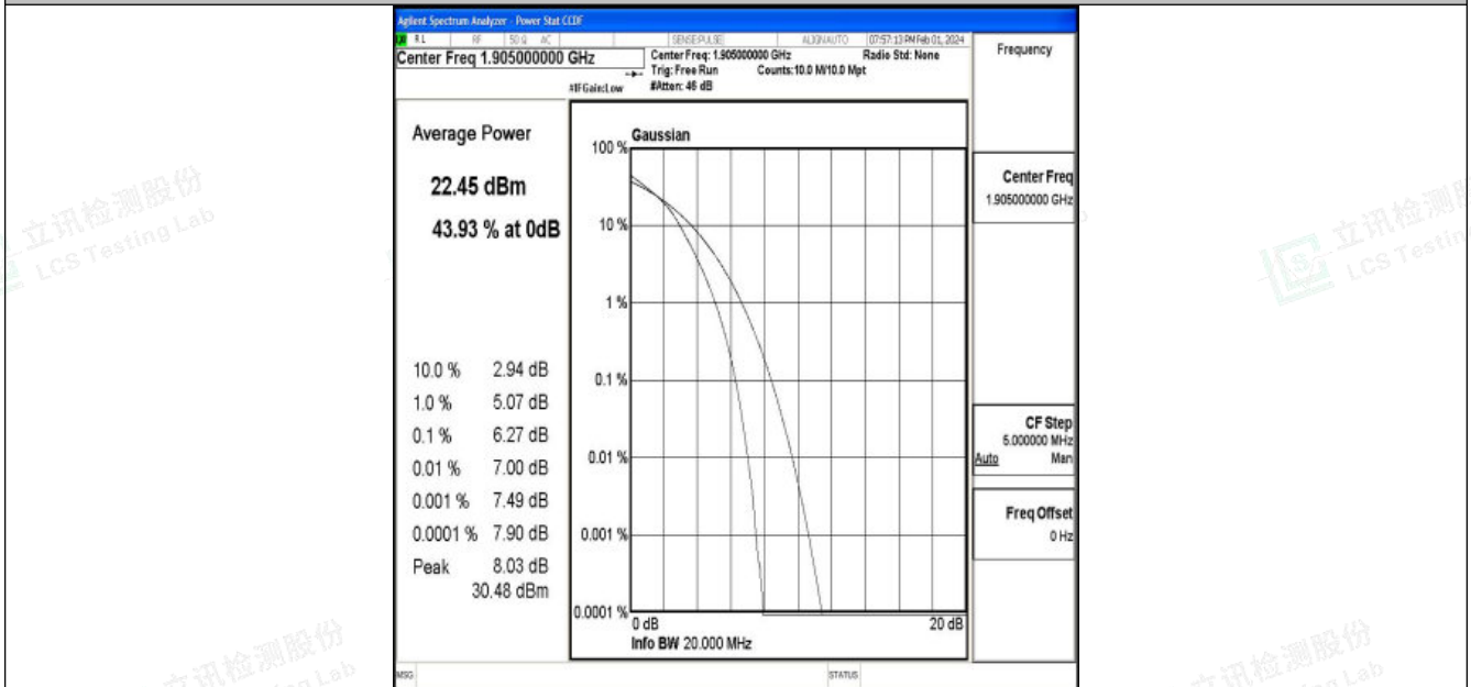
Band25-20MHz-16QAM-26590-100RB#0-PASS
