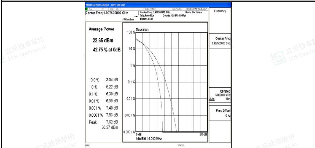
Band25-15MHz-16QAM-26615-75RB#0-PASS
