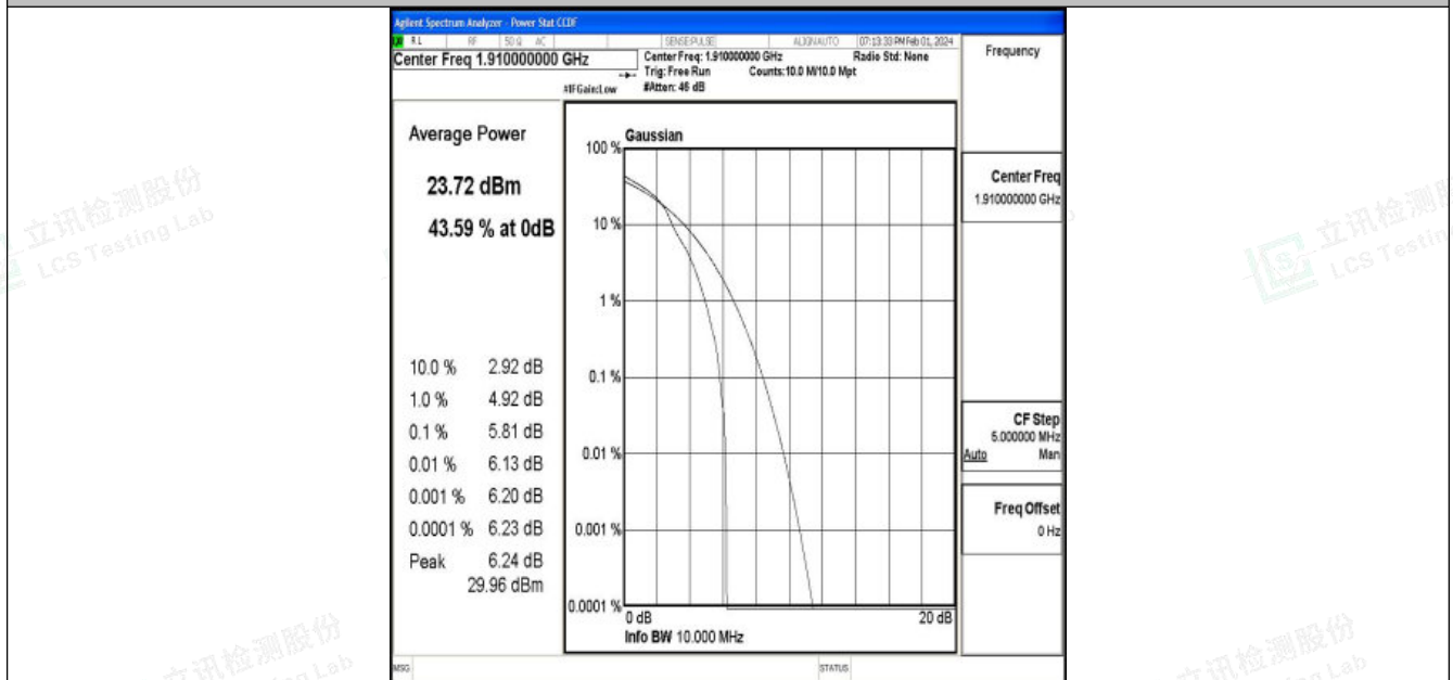
Band25-10MHz-16QAM-26640-1RB#0-PASS
