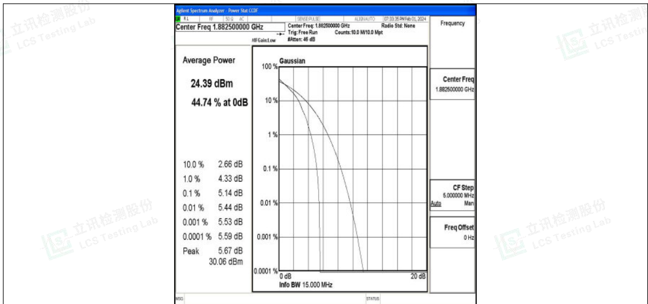
Band25-15MHz-QPSK-26365-1RB#0-PASS
