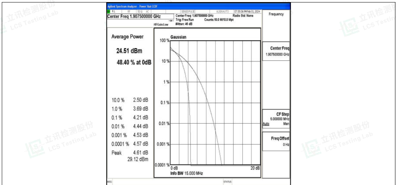
Band25-15MHz-QPSK-26615-1RB#0-PASS
