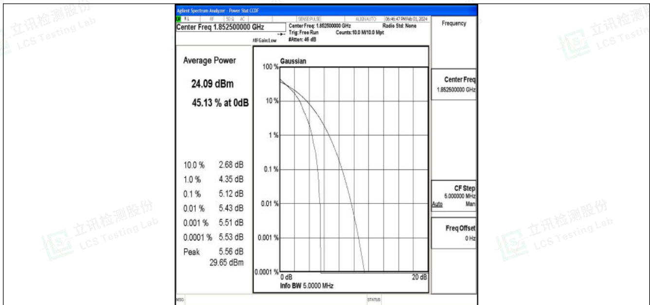
Band25-5MHz-QPSK-26065-1RB#0-PASS
