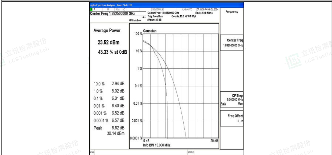
Band25-15MHz-16QAM-26365-1RB#0-PASS
